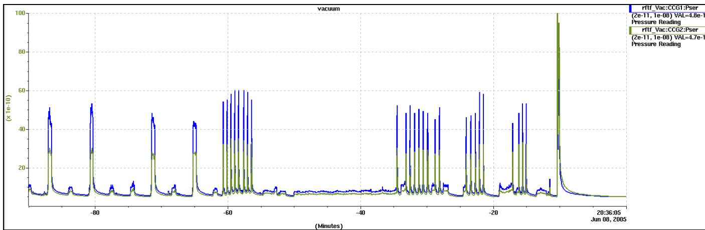
Figure 5.21: Auto cycle and constant power conditioning in standing wave mode
