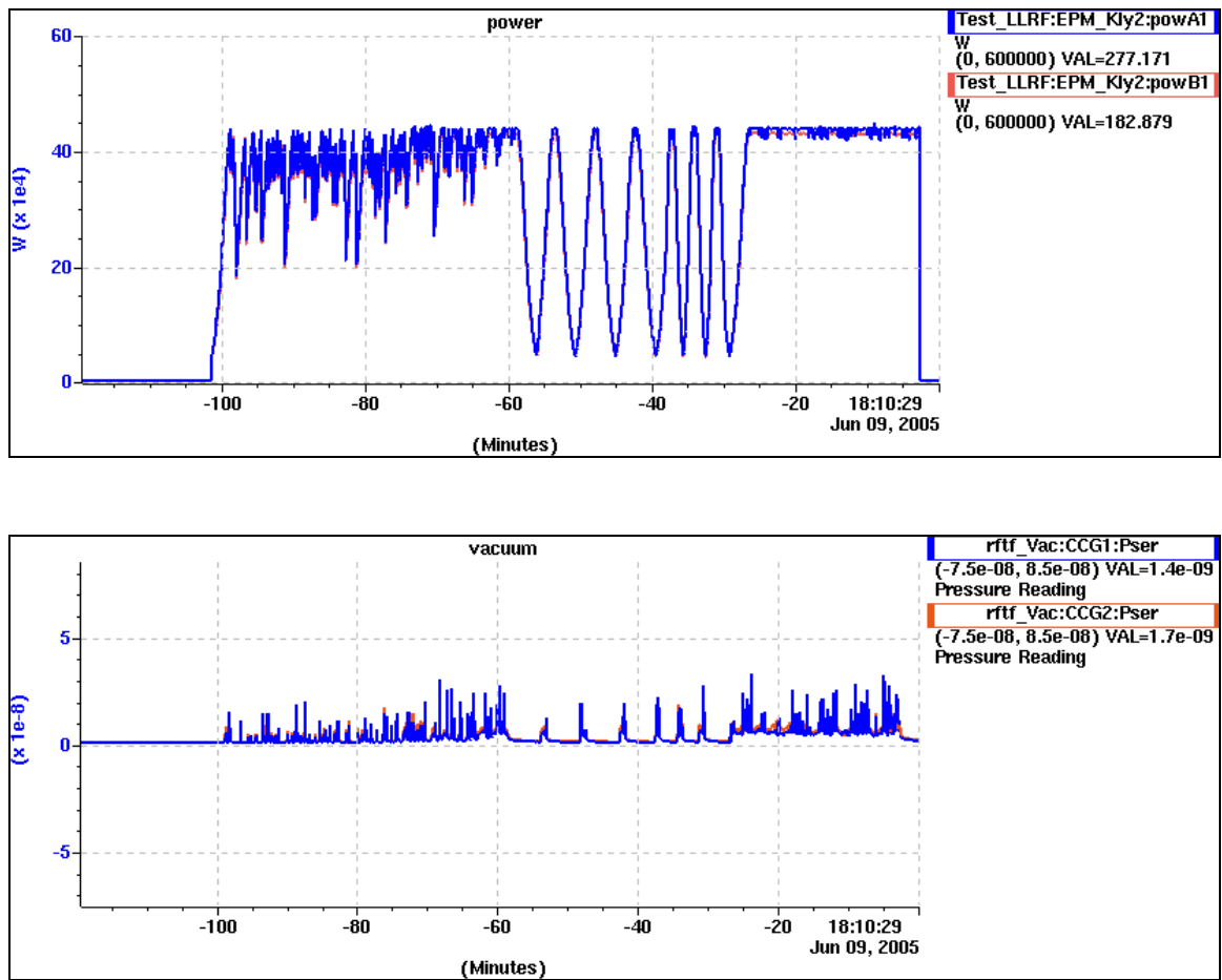
Figure 5.18: Auto cycle and constant power conditioning in traveling wave mode.
