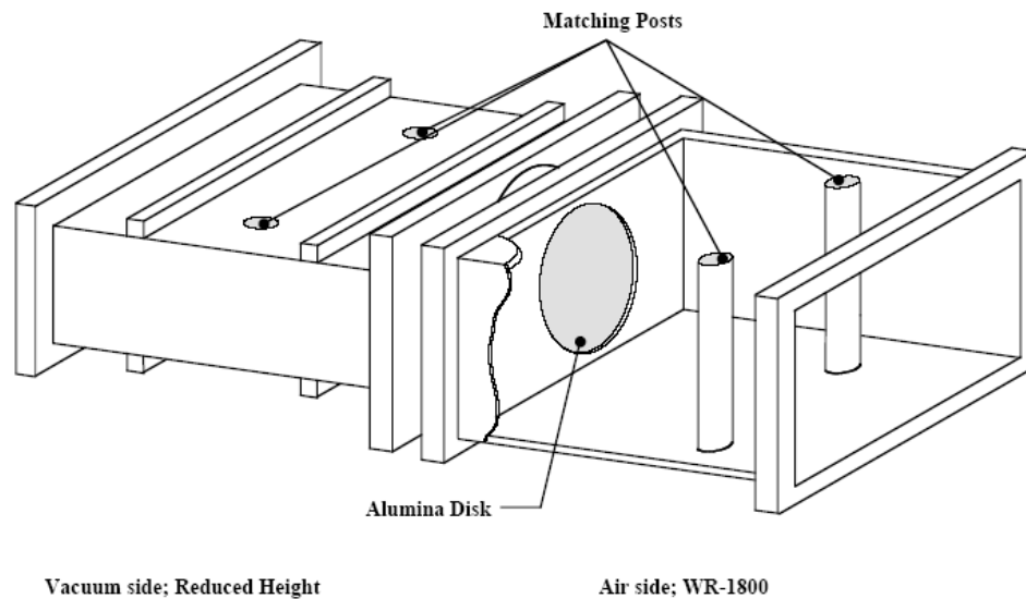
Figure 1.2: A schematic of a RF waveguide window [1].
