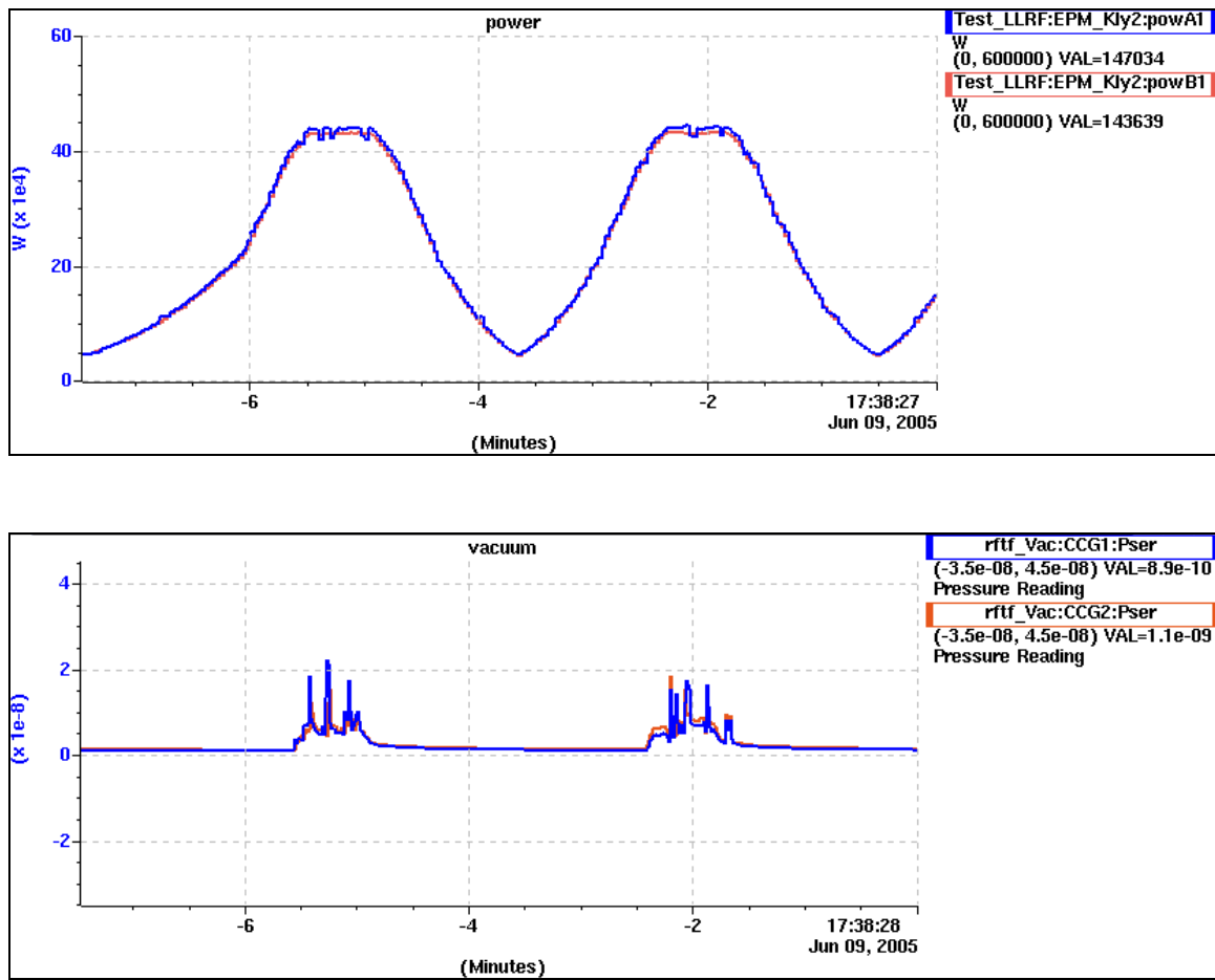
Figure 5.19: The effect in vacuum during the auto cycle conditioning.
