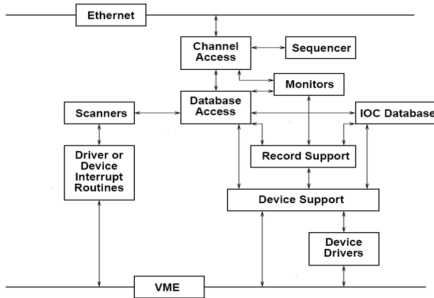
Figure 4.2: EPICS supplied software components for IOC [31].
