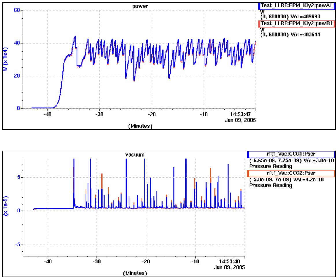
Figure 5.14: First one hour conditioning results in traveling wave mode.
