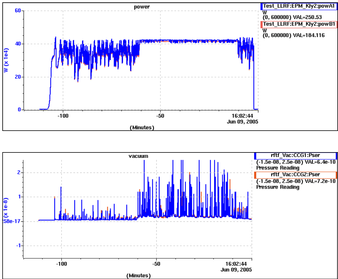
Figure 5.16: Two hour conditioning data in traveling wave mode.
