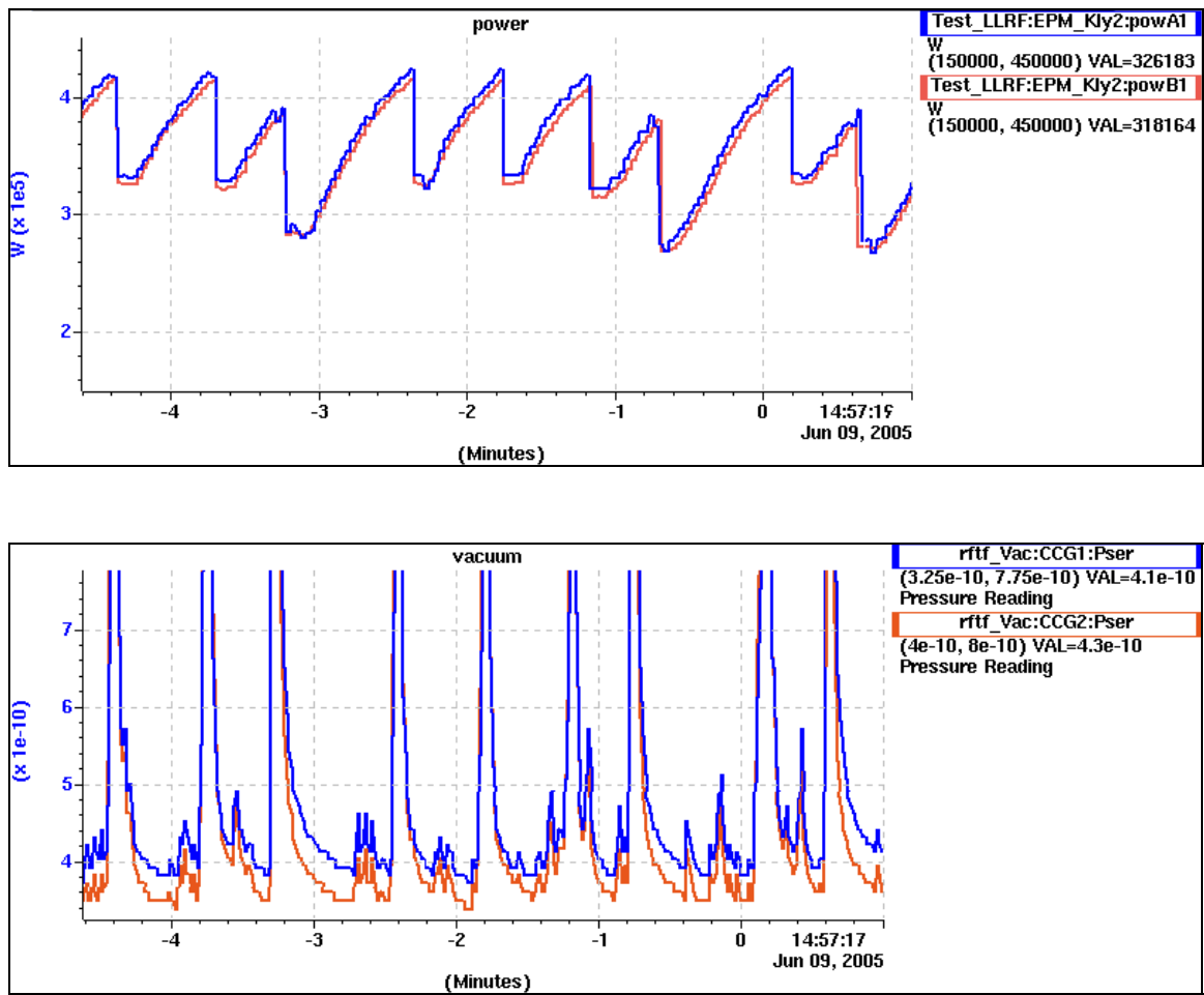
Figure 5.15: RF power backs off when vacuum crosses the predefined upper limit.
