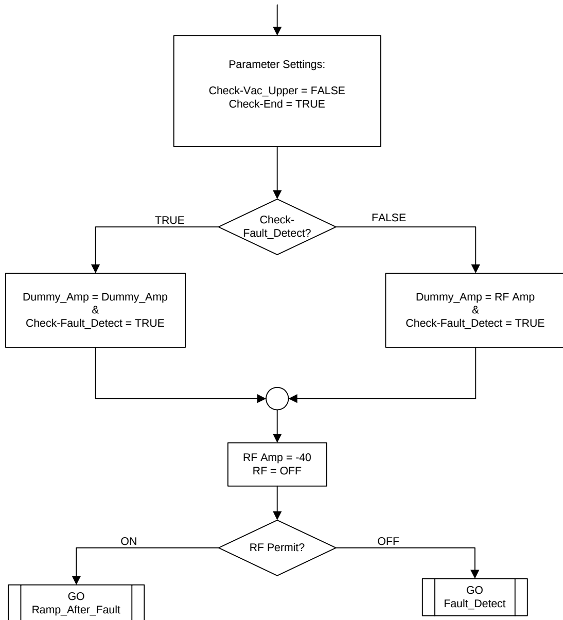
Figure 4.8: Fault detection state.
