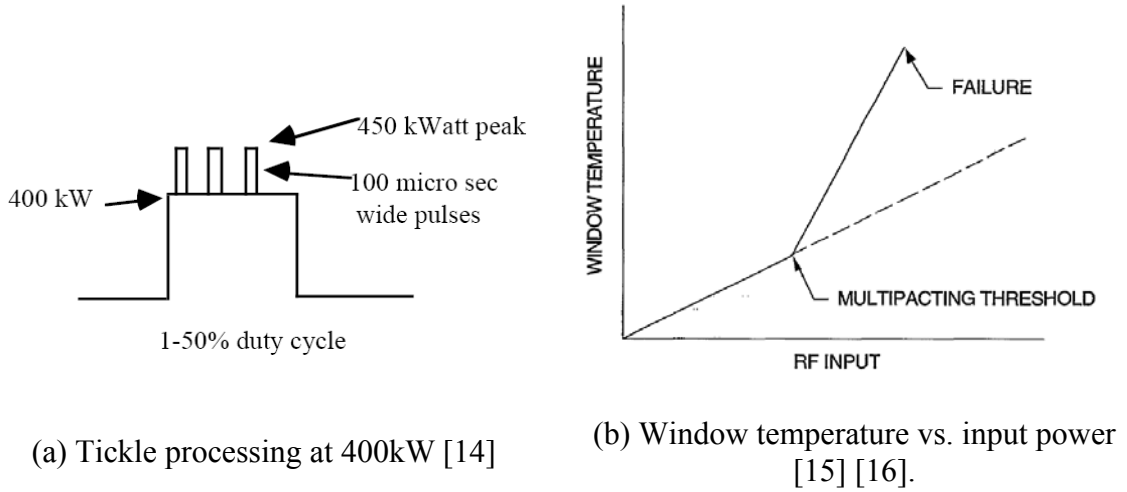
Figure 2.11: RF conditioning process in the literatures.
