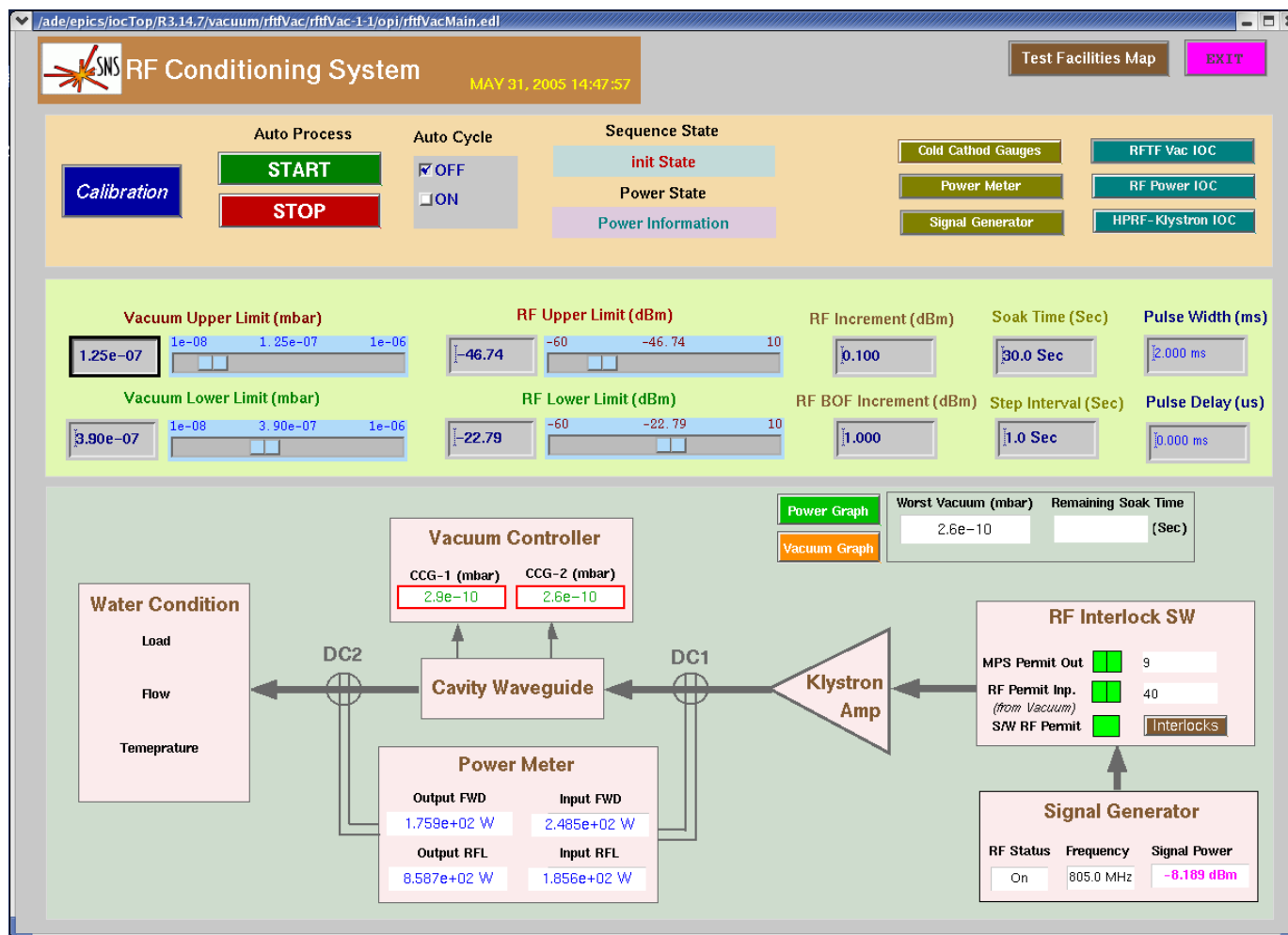
Figure 5.7: Main operator interface (OPI) screen for the RF conditioning system.
