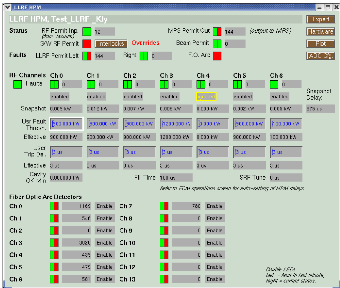
Figure 5.11: OPI screen for setting up and monitoring the instruments connected with the HPM in RF power IOC.
