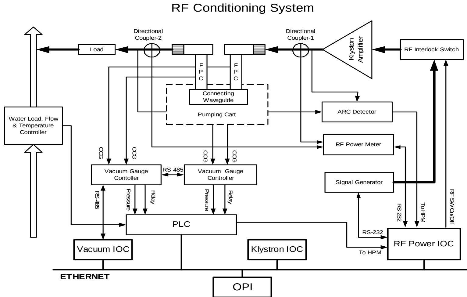
Figure 3.1: Block diagram of the RF conditioning system [19].
