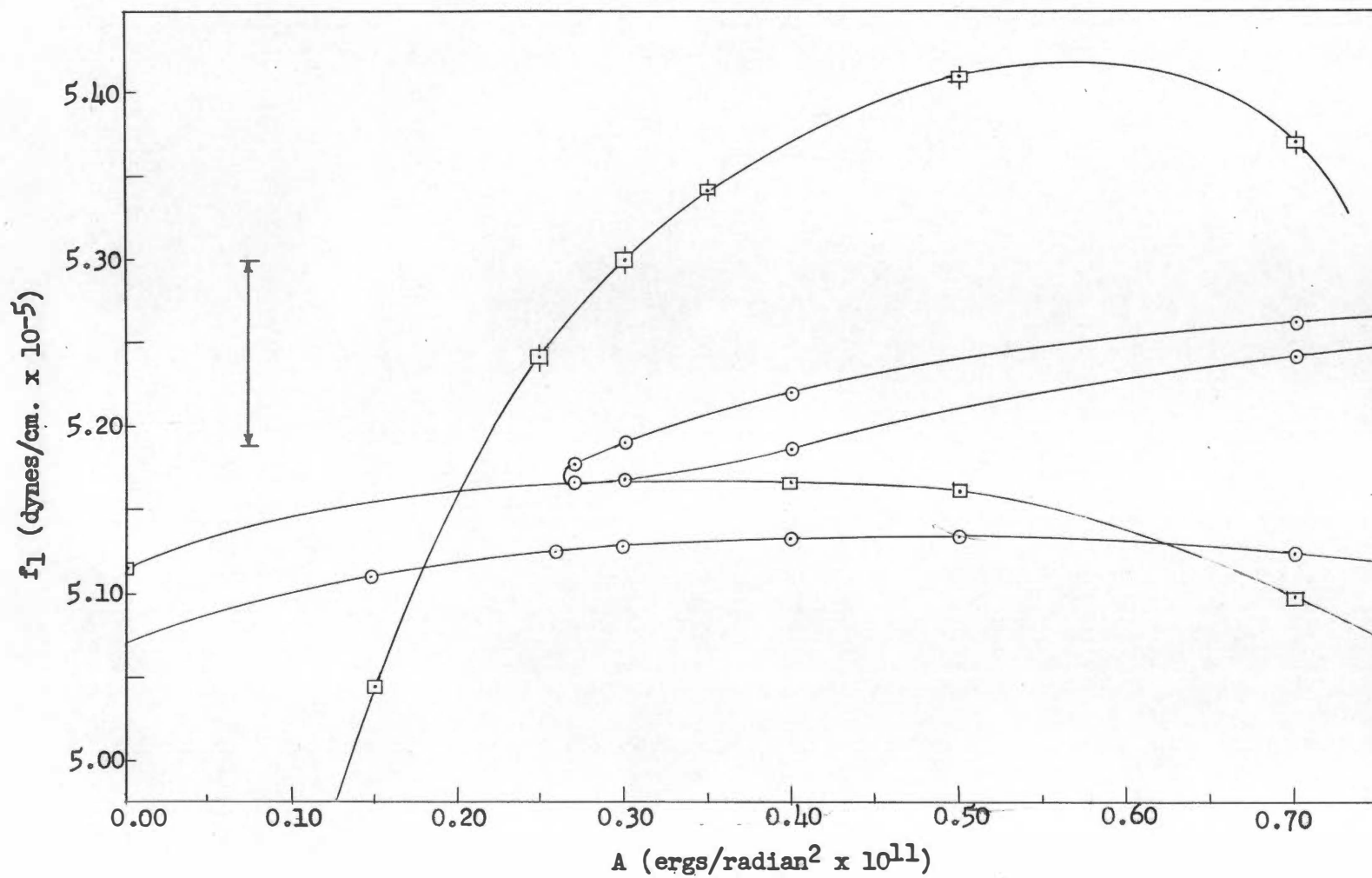
Figure 24. f_1 vs. A for Species A_1 and B_2 of C_3H_4 and C_3D_4 . \circ , A_1 , C_3H_4 ; \odot , A_1 , C_3D_4 ; \square , B_2 , C_3H_4 ; \boxdot , B_2 , C_3D_4 .
