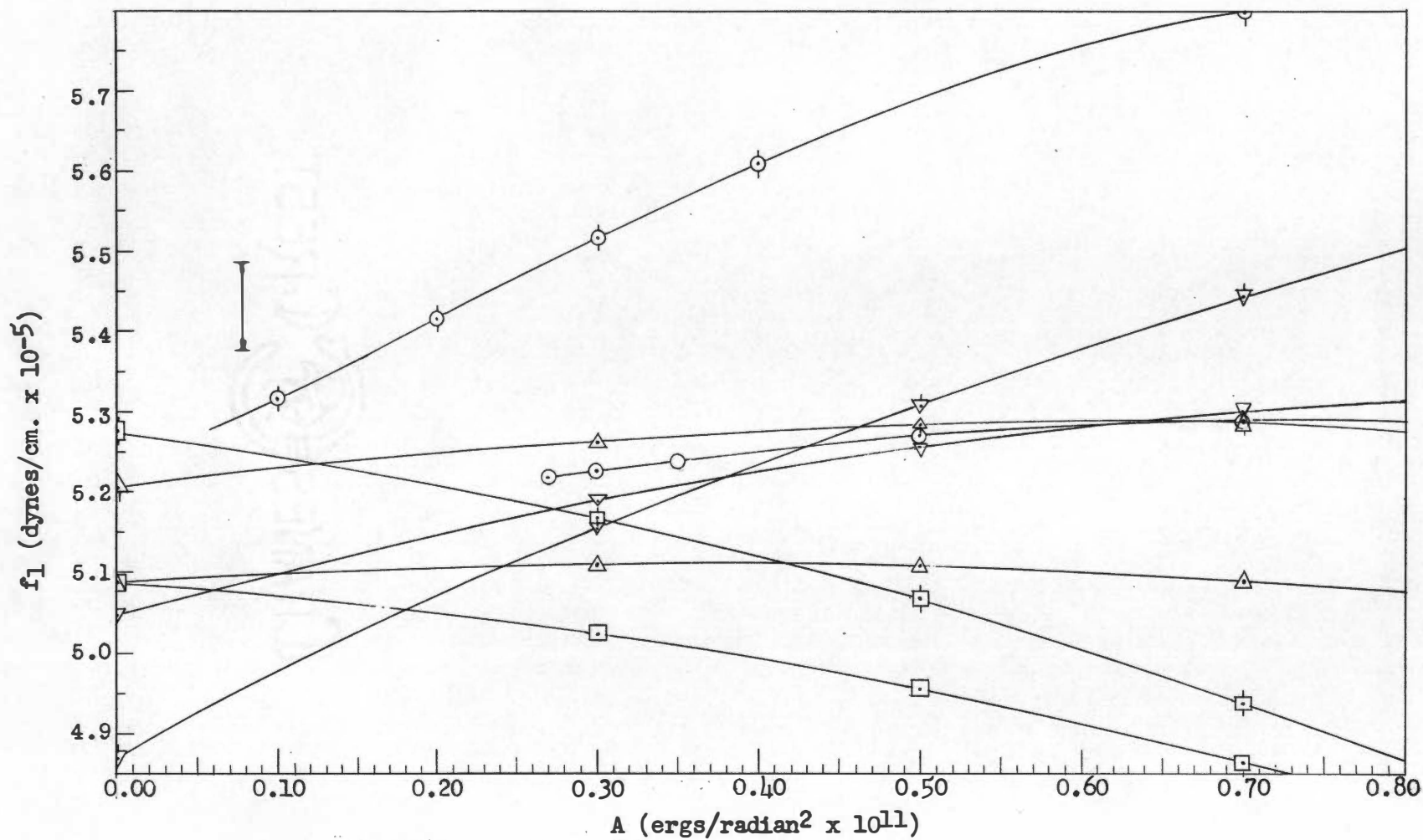
Figure 21. f_1 vs. A for Species A_g , B_{3u} , B_{2u} , and B_{1g} of C_2H_4 and C_2D_4 . o, A_g , C_2H_4 ; \phi , A_g , C_2D_4 ; \square , B_{3u} , C_2H_4 ; \square , B_{3u} , C_2D_4 ; \triangle , B_{2u} , C_2H_4 ; \triangle , B_{2u} , C_2D_4 ; \nabla , B_{1g} , C_2H_4 ; \nabla , B_{1g} , C_2D_4 .
