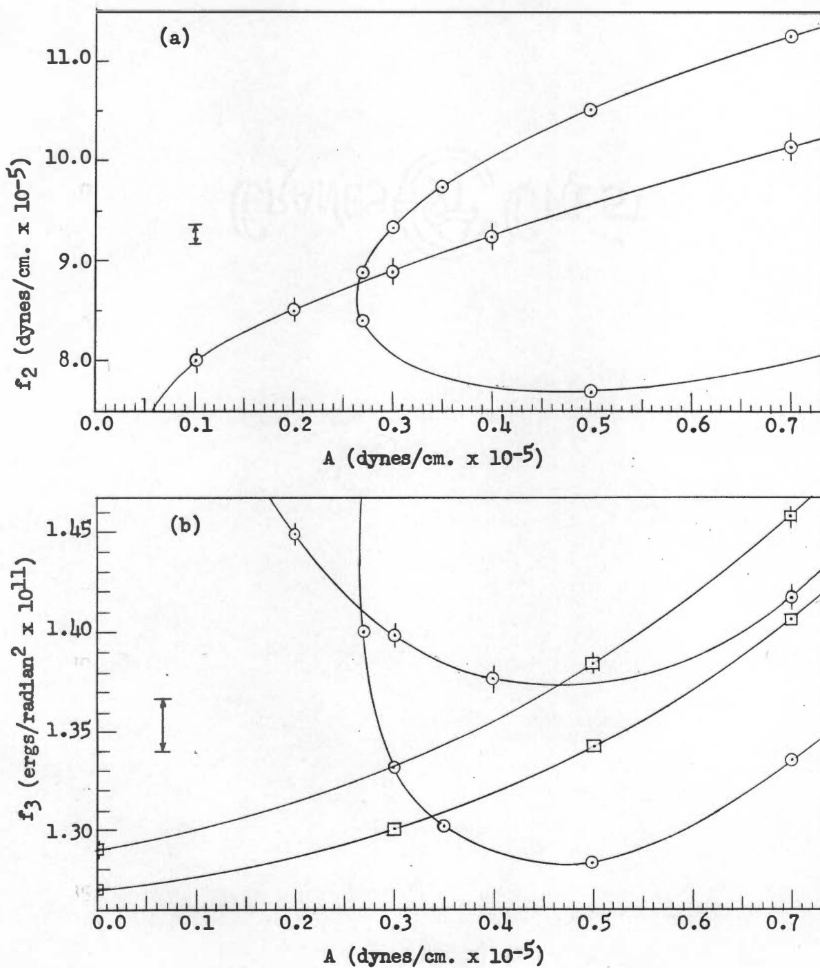
Figure 22. (a) f_2 vs. A for Species \text{Ag} of \text{C}_2\text{H}_4 and \text{C}_2\text{D}_4 . (b) f_3 vs. A for Species \text{Ag} and \text{B}_{3u} of \text{C}_2\text{H}_4 and \text{C}_2\text{D}_4 . \circ , \text{Ag} , \text{C}_2\text{H}_4 ; \phi , \text{Ag} , \text{C}_2\text{D}_4 ; \square , \text{B}_{3u} , \text{C}_2\text{H}_4 ; \boxplus , \text{B}_{3u} , \text{C}_2\text{D}_4 .
