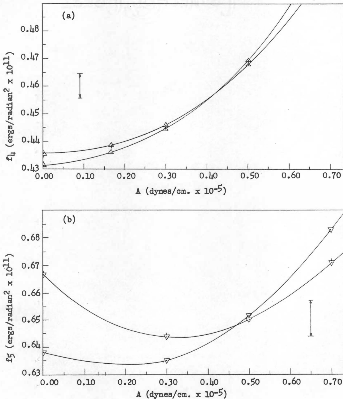
Figure 23. (a) f_4 vs. A for Species B_{2u} of C_2H_4 and C_2D_4 . (b) f_5 vs. A for Species B_{1g} of C_2H_4 and C_2D_4 . \triangle , B_{2u} , C_2H_4 ; \triangle , B_{2u} , C_2D_4 ; \nabla , B_{1g} , C_2H_4 ; \nabla , B_{1g} , C_2D_4 .
