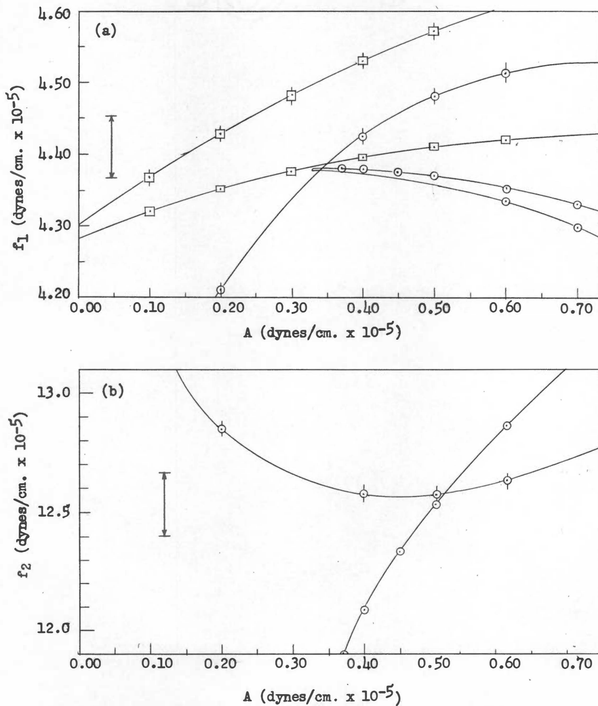
Figure 26. (a) f_1 vs. A for Species A_1 and B_1 of CH_2O and CD_2O .
