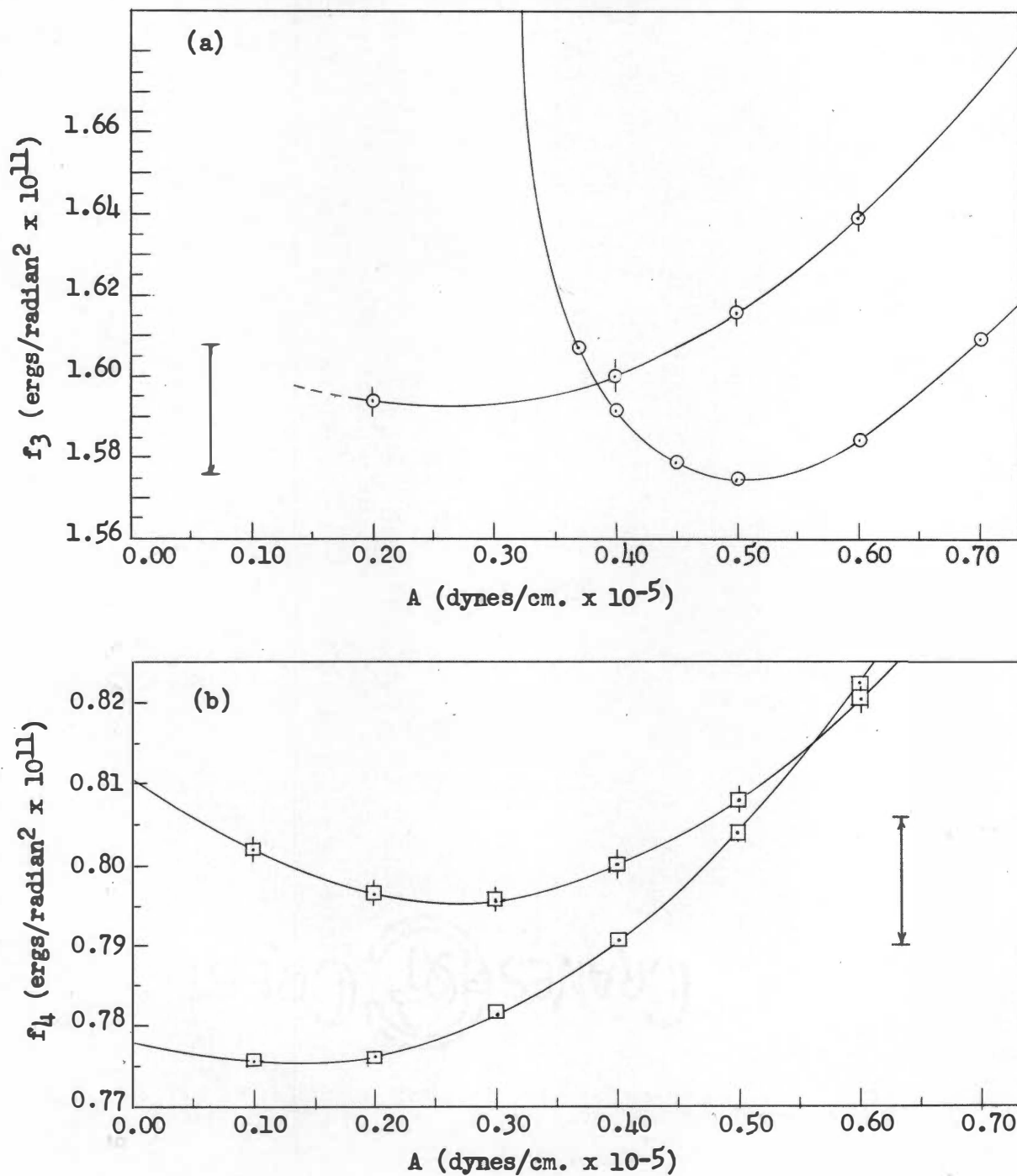
Figure 27. (a) f_3 vs. A for Species A 1 of CH 2 O and CD 2 O. (b) f_4 vs. A for Species B 1 of CH 2 O and CD 2 O. o, A 1 , CH 2 O; \odot , A 1 , CD 2 O; \square , B 1 , CH 2 O; \square , B 1 , CD 2 O.
