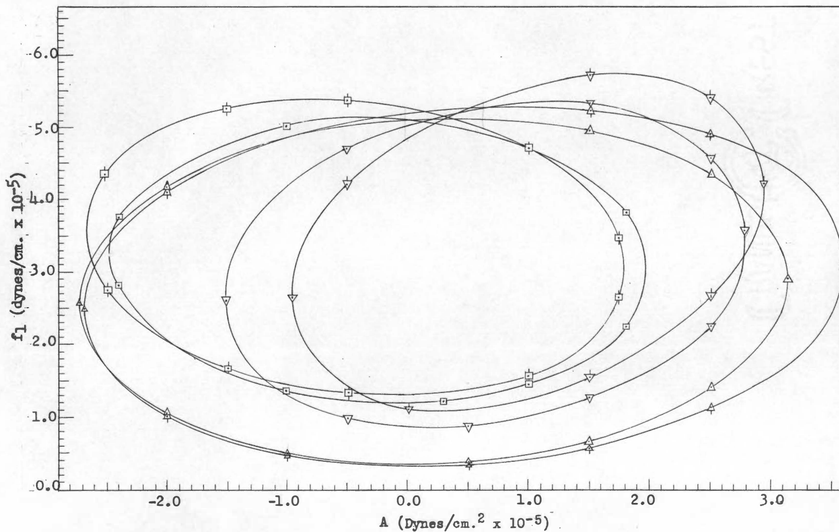
Figure 20. f_1 vs. A for Species B_{3u} , B_{2u} , and B_{1g} of C_2H_4 and C_2D_4 . \square , B_{3u} , C_2H_4 ; \blacksquare , B_{3u} , C_2D_4 ; \triangle , B_{2u} , C_2H_4 ; \blacktriangle , B_{2u} , C_2D_4 ; \nabla , B_{1g} , C_2H_4 ; \blacktriangledown , B_{1g} , C_2D_4 .
