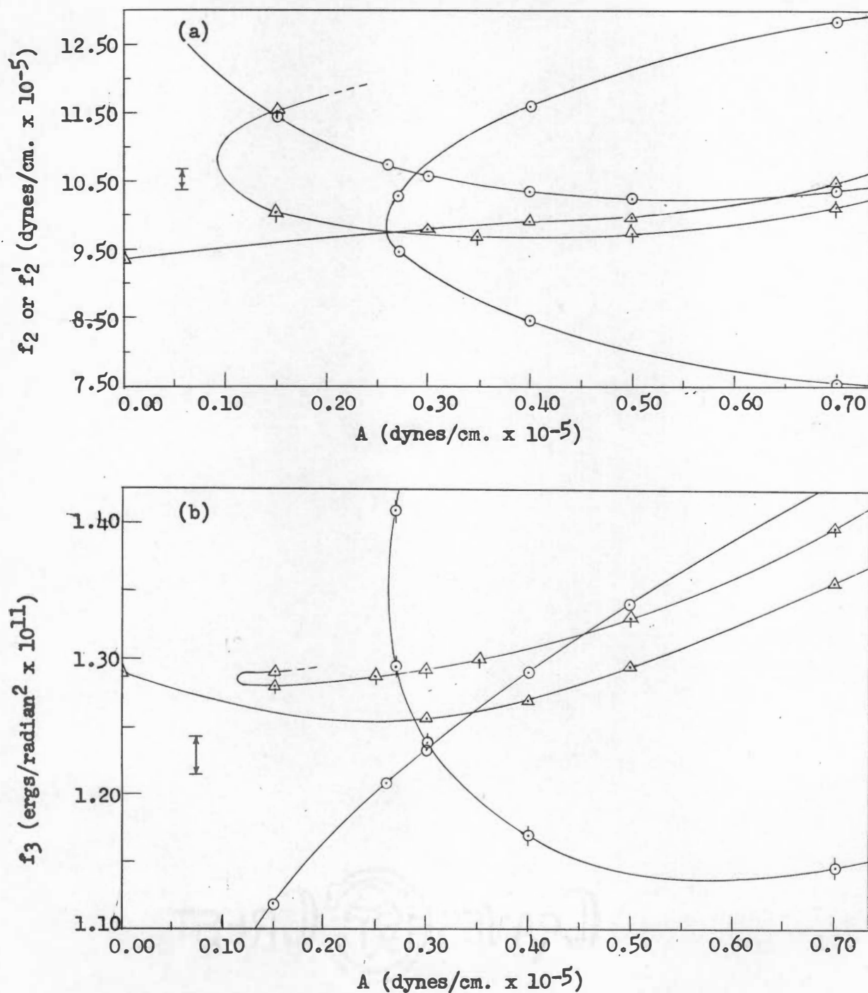
Figure 25. (a) f_2 or f_2' vs. A for Species A_1 and B_2 of C_3H_4 and C_3D_4 . (b) f_3 vs. A for Species A_1 and B_2 of C_3H_4 and C_3D_4 . \circ , A_1 , C_3H_4 ; \phi , A_1 , C_3D_4 ; \triangle , B_2 , C_3H_4 ; \nabla , B_2 , C_3D_4 .
