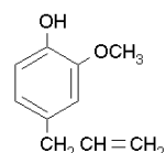
Eugenol
