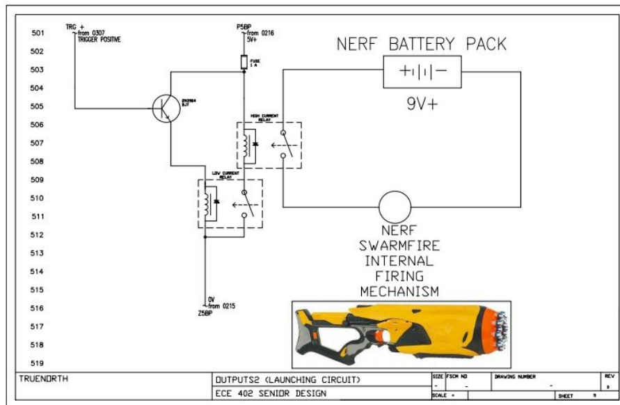
A few Images of the detailed hardware drawings created in AutoCAD Electrical. Details include wire color, fuse requirements, part details, available voltage, etc.
