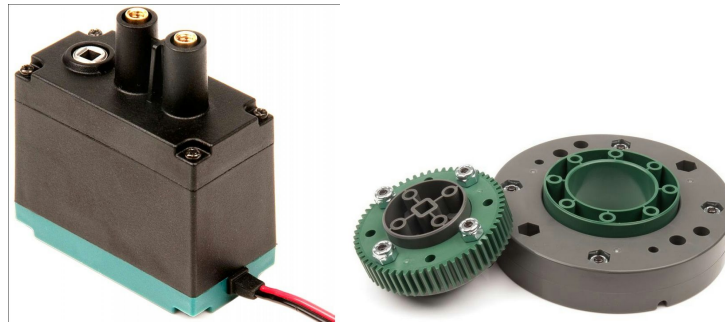
Left: Vex 393 motor Right: Vex turntable bearing kit Image Courtesy of www.vexrobotics.com
