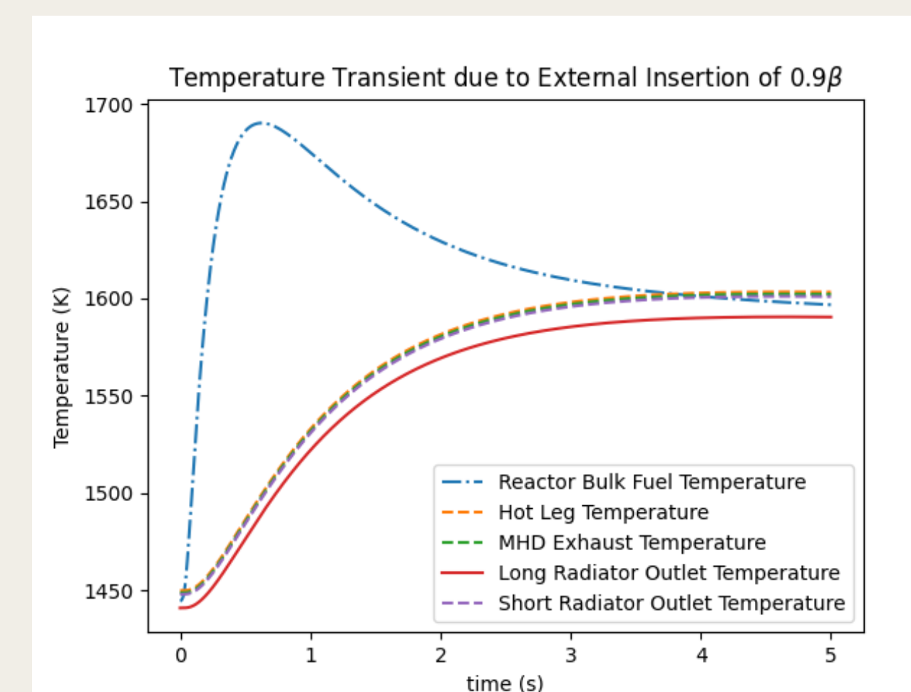
Figure 5. Temperature transient due to external reactivity insertion
