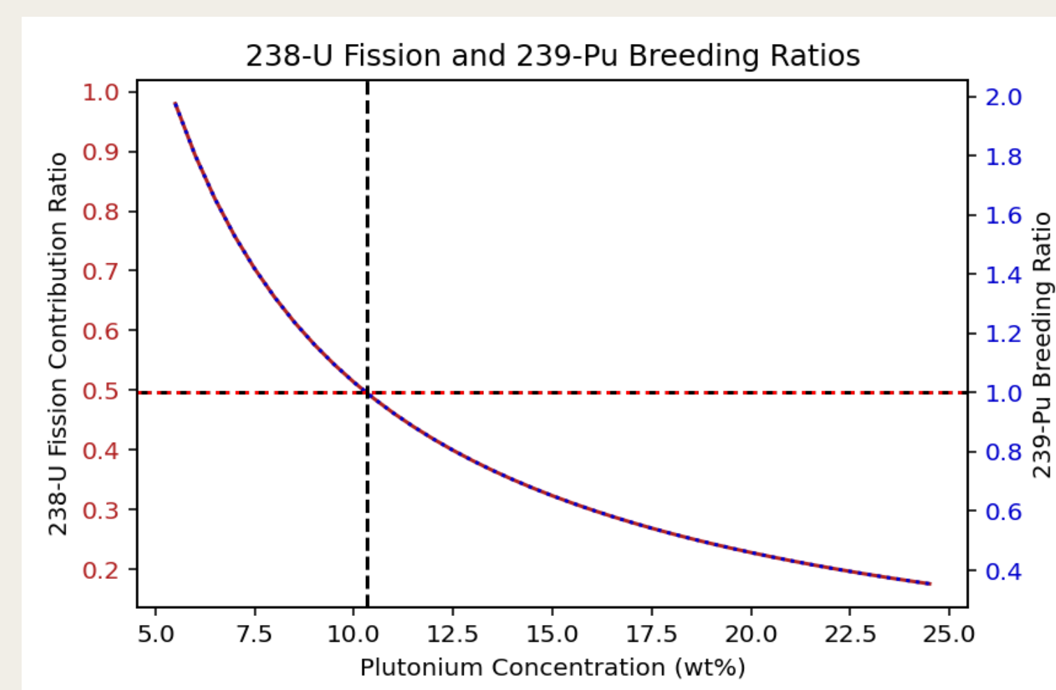
Figure 2. Fission and breeding ratios based on MCNP spectrum
