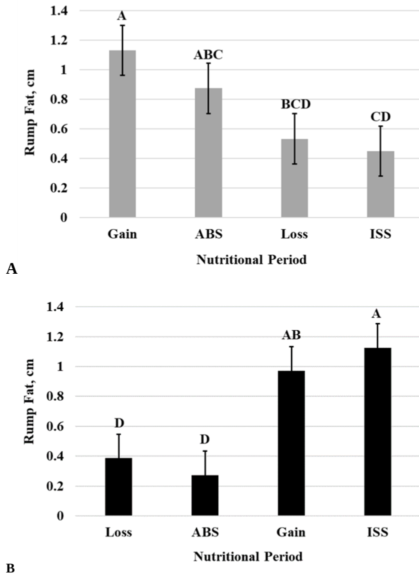
Figure 4. Rump fat measurements (Raw Mean \pm SEM; P < 0.005 ) for the OVER treatment pathway (a) included: the gain ( 1.13 \pm 0.17 ), ABS ( 0.88 \pm 0.17 ), loss ( 0.53 \pm 0.17 ) and ISS period ( 0.45 \pm 0.17 ). The RES pathway (b) included: the loss ( 0.39 \pm 0.16 ), ABS ( 0.27 \pm 0.16 ), gain ( 0.97 \pm 0.16 ) and ISS ( 1.13 \pm 0.16 ).
