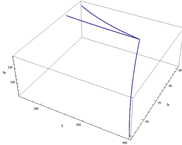
Figure 17 This figure demonstrates our new bifurcation diagram after changing g to a piecewise linear function, rescaling with respect to T , and then changing h to a linear function.
