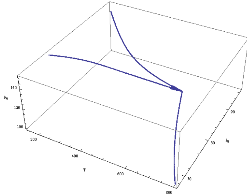
Figure 15 This figure demonstrates our new bifurcation diagram after changing g to a piecewise linear function.
