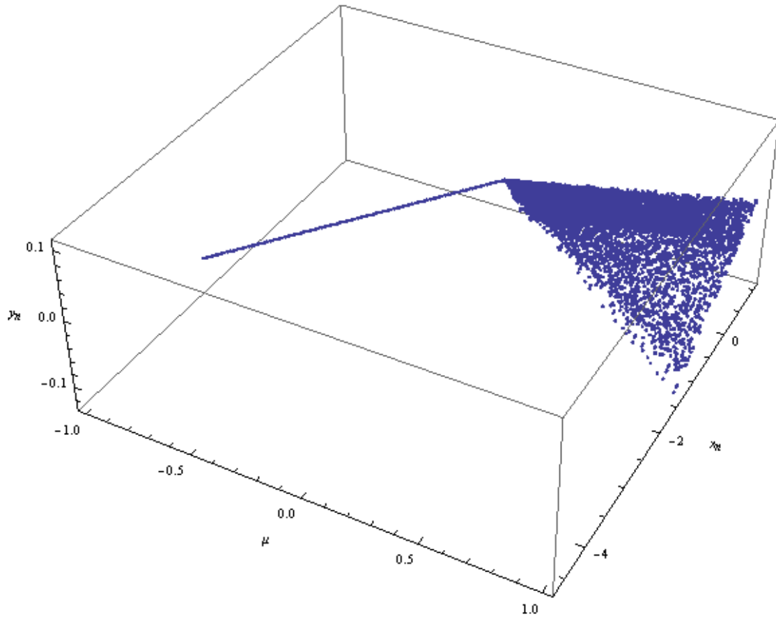
Figure 23 This bifurcation diagram occurs when \tau_L = 0.5534 , \tau_R = -5.4934 , \delta_L = -0.02825 , and \delta_R = -0.25165 . As expected, when conditions (4.29) and (4.30) are not met, we result in chaos.
