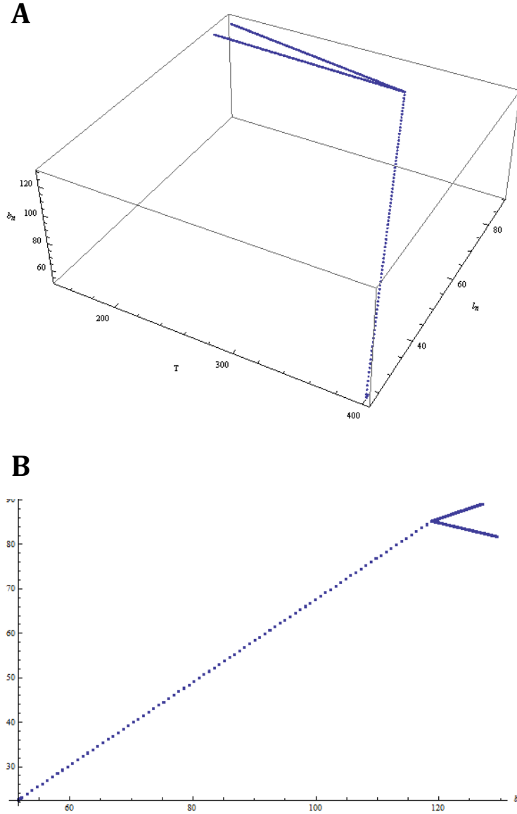
Figure 20 This figure demonstrates our new bifurcation diagrams of our two-dimensional piecewise linear map. This is what occurs after changing g to a piecewise linear function, rescaling with respect to T , changing h to a linear function, and rescaling with respect to T once more, then finally changing c(T) to a linear function as well. (A) Bifurcation diagram showing bifurcation with respect to varying parameter T ; (B) Bifurcation diagram showing b_n vs. l_n .
