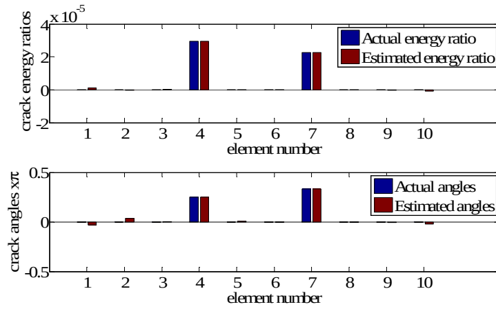
Fig. 4.10 Converged shaft crack damage energy ratio estimates: Case VI
