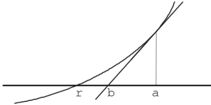
Fig. 4.7 Newton method [155]
