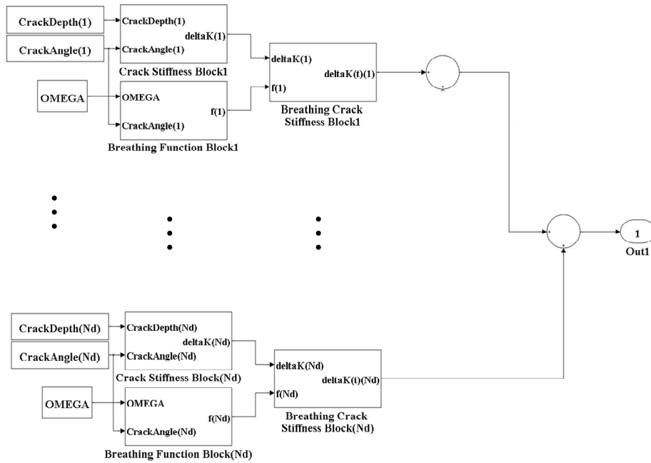
Fig. 6.19 Cosine Crack Model Block
