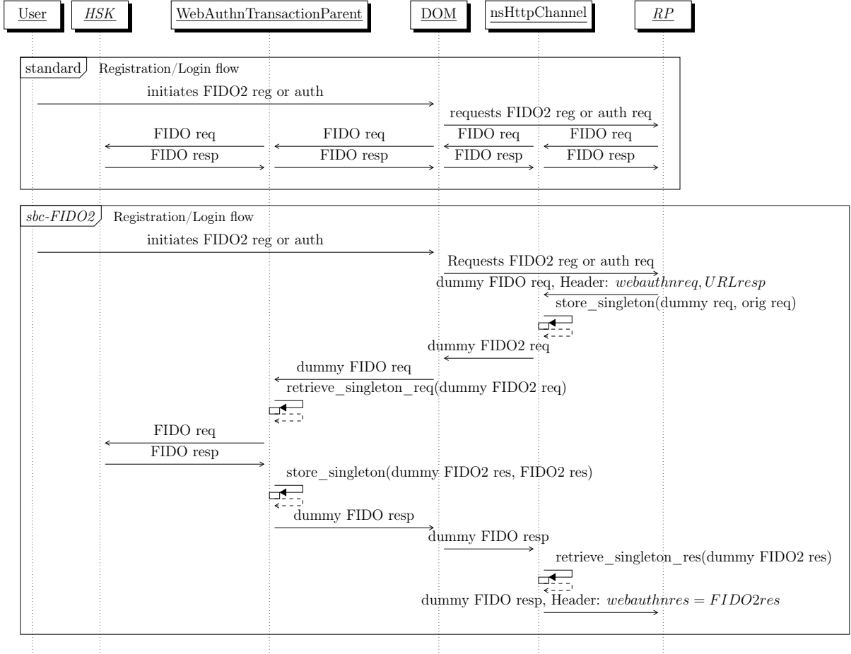
Figure 5.3: sbc-FIDO2 sequence diagram
