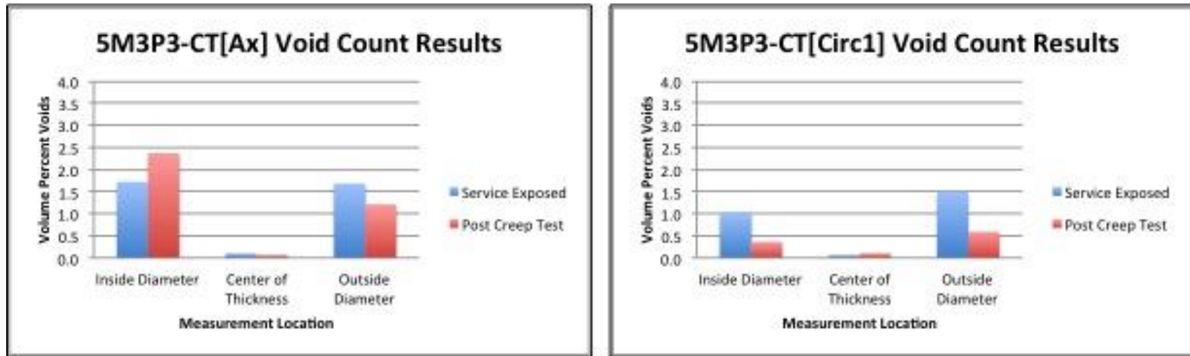
Figure 19. Void count results for the creep samples from the ex-service HP tube 5M3P3 compared to the service-exposed sample of the same orientation. Measurements were taken from areas of the samples corresponding to just inside the inside diameter, the center of thickness, and just inside the outside diameter of the tube. The axially tested creep sample is compared to the longitudinal ex-service sample and the circumferentially creep tested sample is compared to the transverse ex-service sample.
