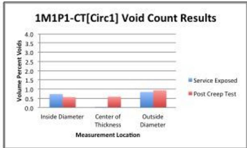
Figure 15. Void count results for the creep samples from the ex-service HP tube 1M1P1 compared to the service-exposed sample of the same orientation. Measurements were taken at areas of the samples corresponding to just inside the inside diameter, the center of thickness, and just inside the outside diameter of the tube. The axially tested creep sample is compared to the longitudinal ex-service sample and the circumferentially creep tested sample is compared to the transverse ex-service sample.
