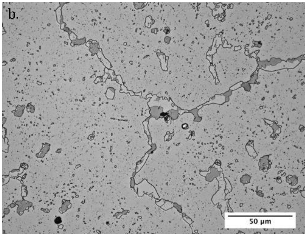
Figure 11. HP tube sample 4M3P3-SE OLM micrographs at a) 27.5X and b) 275X printed magnification.
