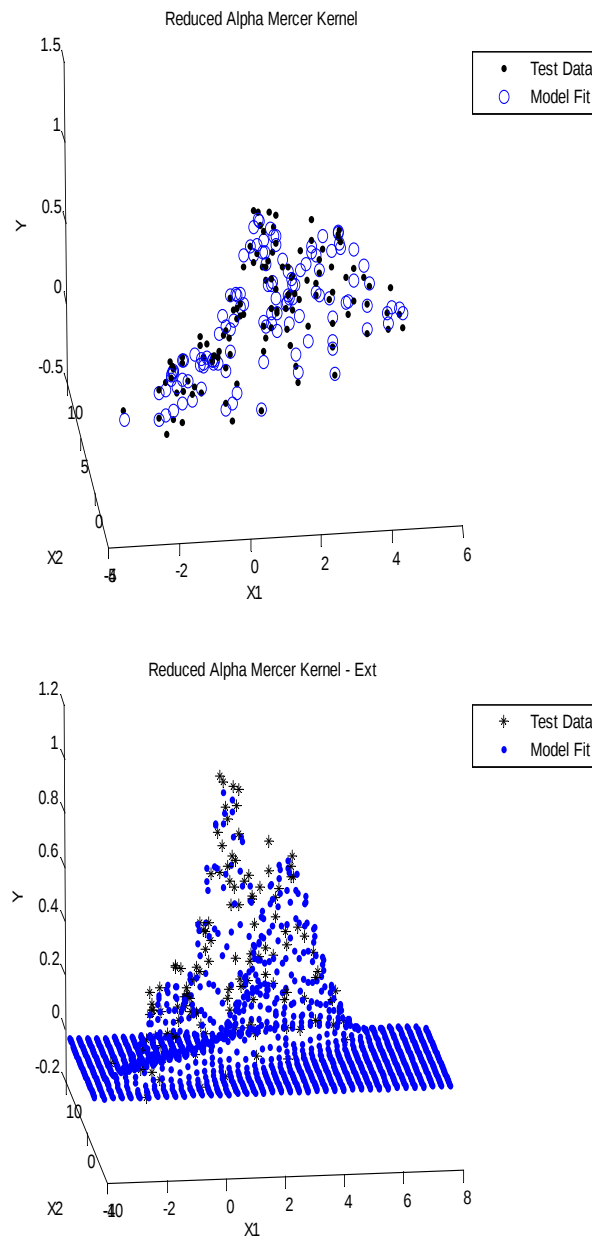
Figure 2.6: Kernel Trick Demonstration Model Fit
