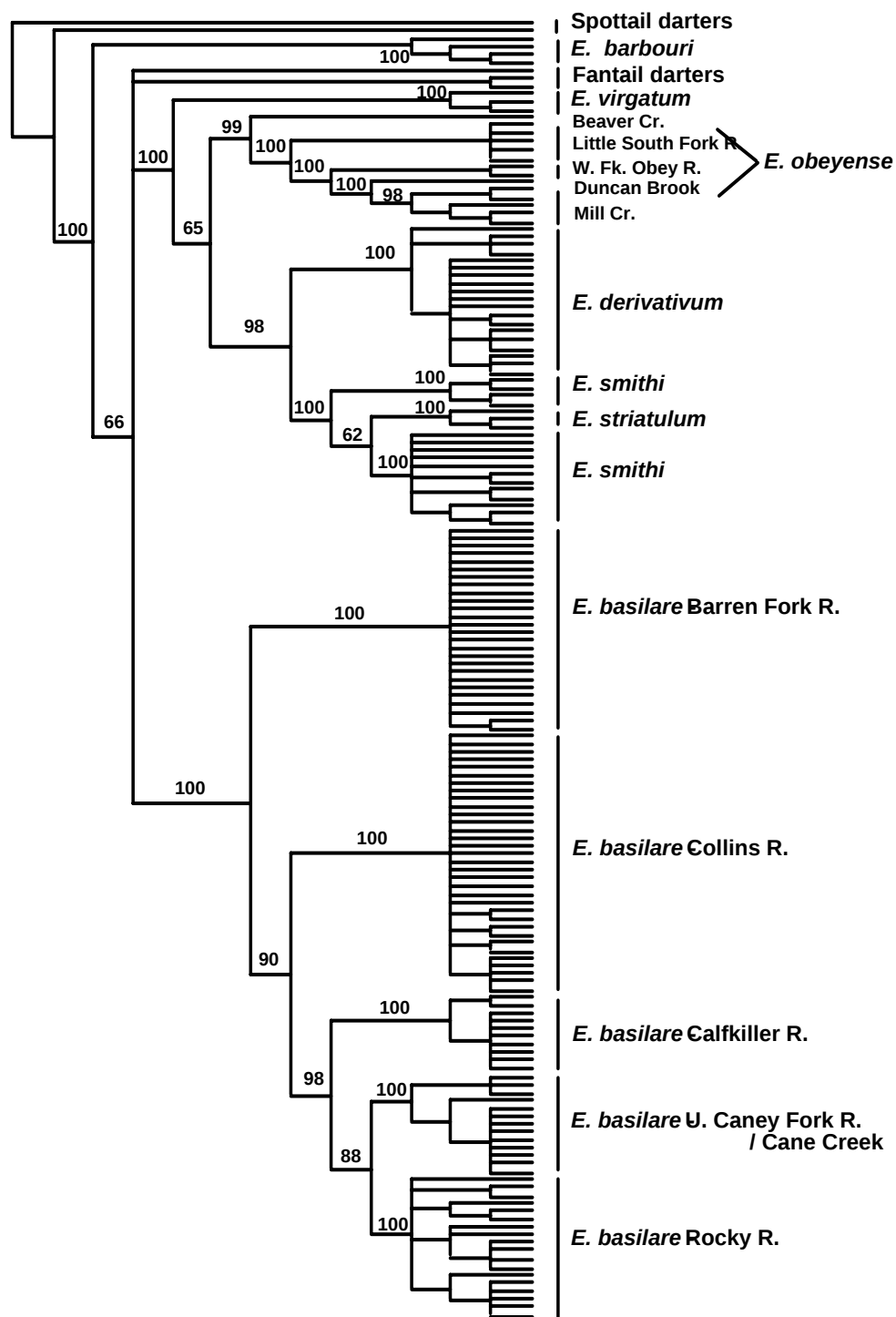
Figure 6. Strict consensus tree resulting from maximum parsimony analysis of 2956 base pairs of mtDNA + nDNA from 159 barcheek darter individuals. The outgroup for this analysis was 5 individuals representing the other two species groups in Catnotus . Numbers above the trees represent bootstrap support values. Nodes receiving a bootstrap score of less than 50 have been collapsed.
