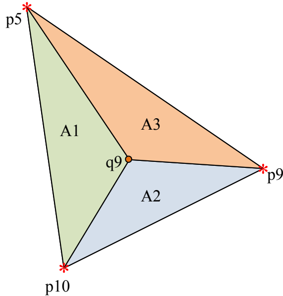
Figure 3-3. Barycentric interpolation.
