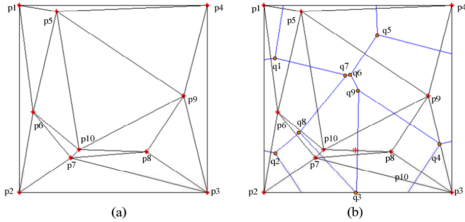
Figure 3-2. Voronoi diagram.
