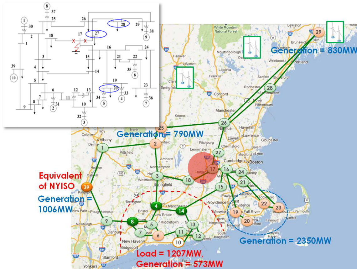
Figure 4-7. IEEE 39-bus system and the most severe N-2 contingency and three candidate buses for dynamic var supports.
