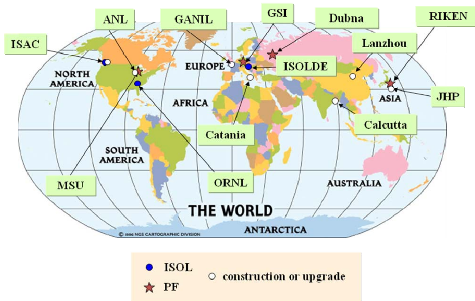
Figure 3.1. Major radioactive beam facilities around the world. In addition to these facilities, plans for a new generation of facilities are under way in the U.S.A (FRIB) and in Europe (EURISOL).
