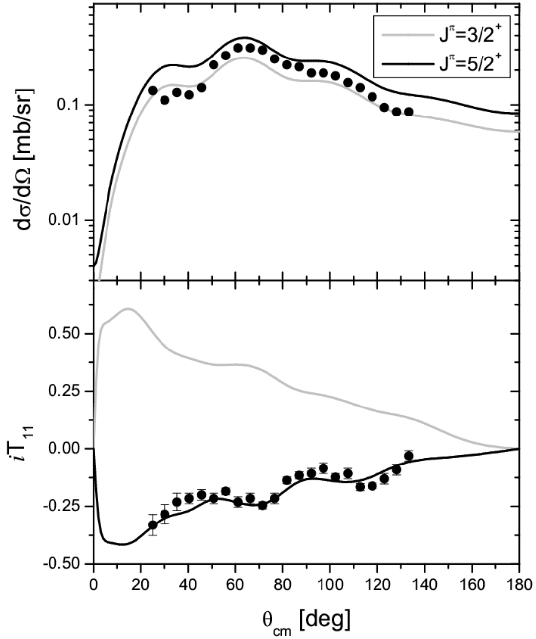
Figure 3.8. Spin dependent observables in a transfer reaction involving a fission fragment-like nucleus. The top panel shows the differential cross section for an excited state ( E_x=1.18 MeV) populated in the reaction ^{118}\text{Sn}(\bar{d},t)^{117}\text{Sn} , while the bottom panel shows the vector analyzing power (in spherical representation). The dots represent experimental data extracted from [Vig 75], while the lines correspond to DWBA calculations for two allowed values in spin for the residual nucleus. The parameters associated with the potentials were extracted from [Vig 75].
