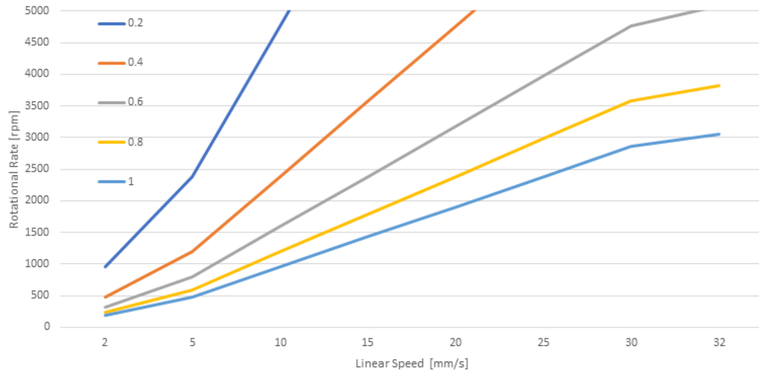
Figure 2.10: Maximum rotational rate vs linear speed for different nozzles sizes
