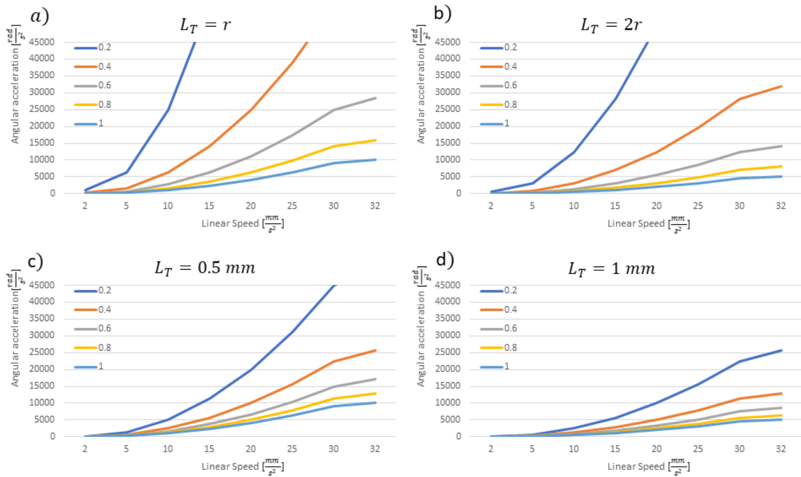
Figure 2.11: Maximum angular acceleration vs linear speeds for different nozzle sizes, at different transition length
