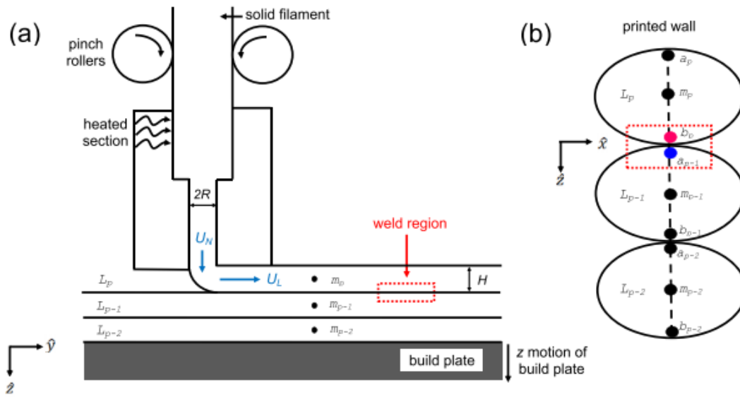
Figure 1.5: Weld formation of deposited material during FFF 3D printing Source: [43]
