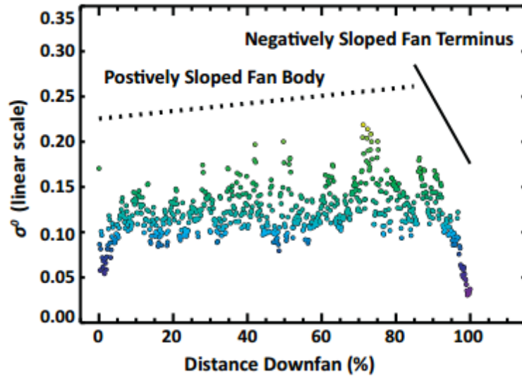
Figure 2.5. Downfan \sigma^0 profile line for Panamint Range fan 2, with the line fits to the fan body (0 to 85% downfan distance, black dashed line) and fan terminus (86 to 100% downfan distance, black solid line). In this example, \sigma^0 of the fan body region increases with downfan distance (positive slope), whereas \sigma^0 of the fan terminus decreases with downfan distance (negative slope), as summarized in Table 2.7.
