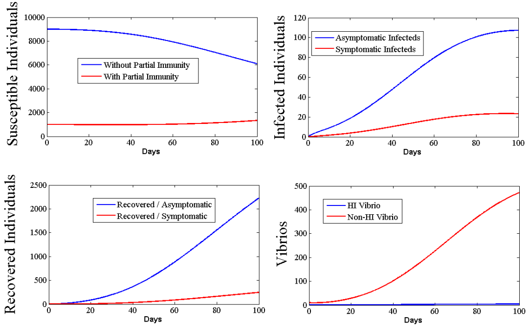
Figure 6.2: Outbreak Simulation
