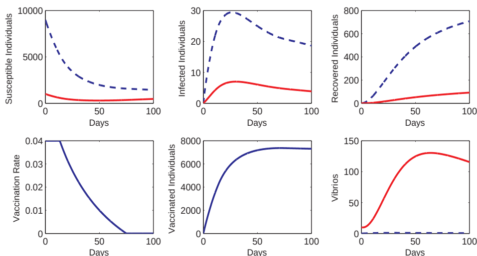
Figure 6.10: \beta_L changed into 0.04. Case 1
