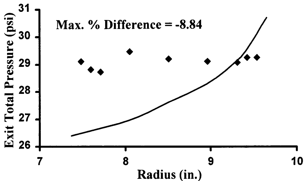
Figure 5.11. Radial Distribution of Exit Total Pressure for Stage 35 Rotor.
