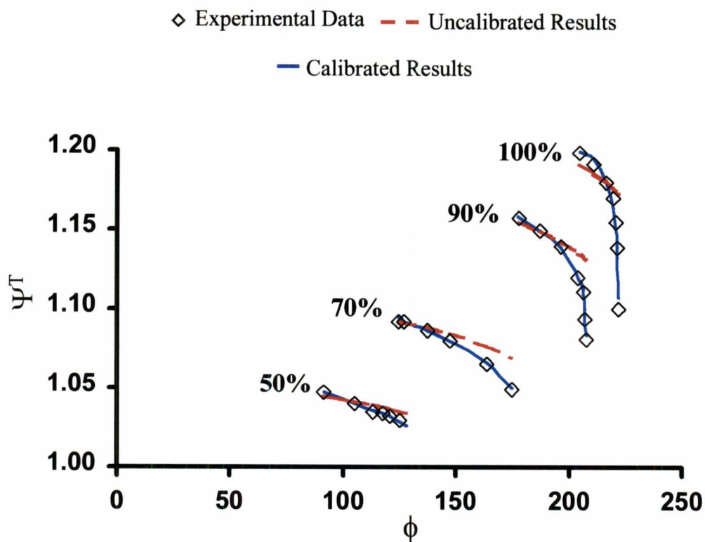
Figure 4.22. 1-D Temperature Characteristic Map for Rotor 1B.
