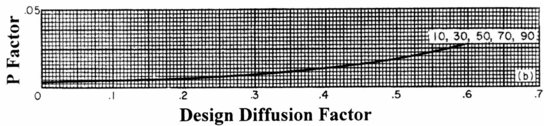
Figure 3.5. P Factor for Minimum Loss Calculation
