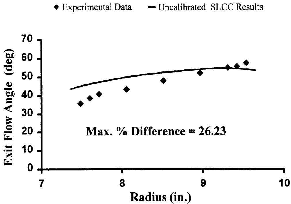
Figure 5.6. Radial Distribution of Exit Flow Angle for Stage 35 Rotor.
