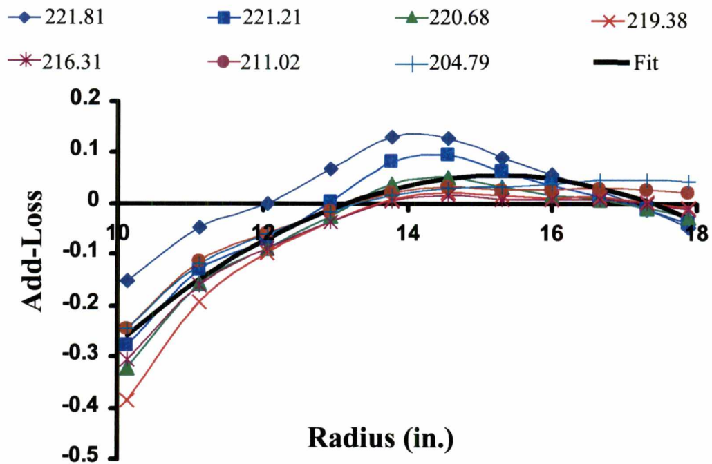
Figure 4.13. Radial Distribution of Add-Loss at 100-Percent Speed for Various Mass Flows for Rotor1B.
