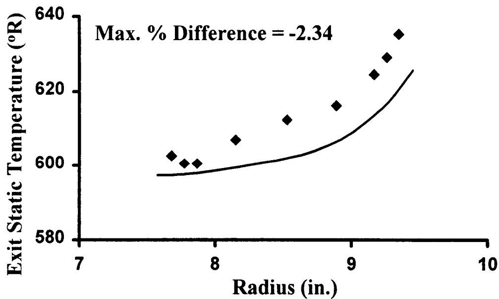
Figure 5.22. Radial Distribution of Exit Static Temperature for Stage 35 Stator.
