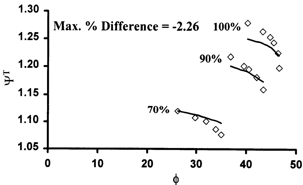
Figure 5.24. 1-D Temperature Characteristic Map for Stage 35.
