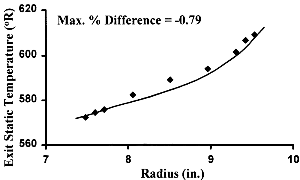
Figure 5.14. Radial Distribution of Exit Static Temperature for Stage 35 Rotor.
