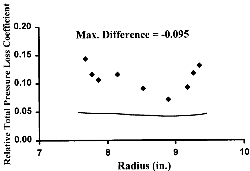
Figure 5.15. Radial Distribution of Relative Total Pressure Loss Coefficient for Stage 35 Stator.
