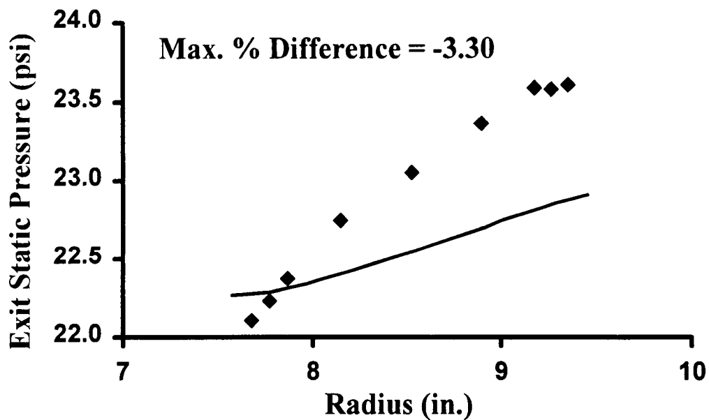
Figure 5.20. Radial Distribution of Exit Static Pressure for Stage 35 Stator.
