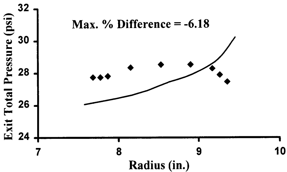
Figure 5.19. Radial Distribution of Exit Total Pressure for Stage 35 Stator.
