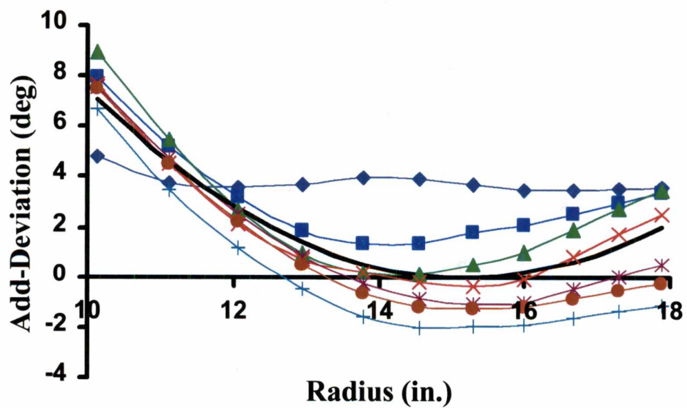
Figure 4.14. Radial Distribution of Add-Deviation at 100-Percent Speed for Various Mass Flows for Rotor1B.
