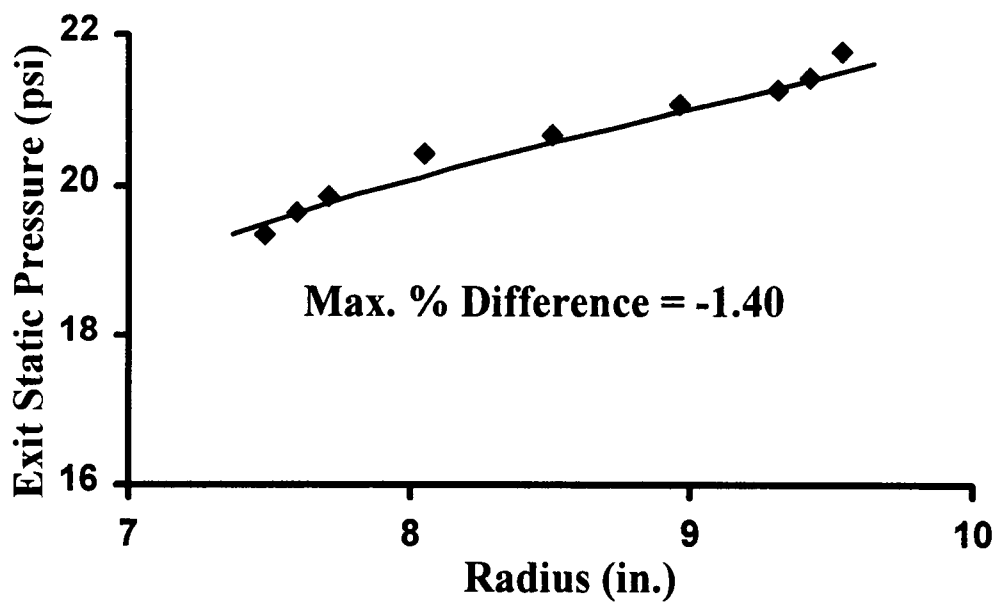
Figure 5.12. Radial Distribution of Exit Static Pressure for Stage 35 Rotor.
