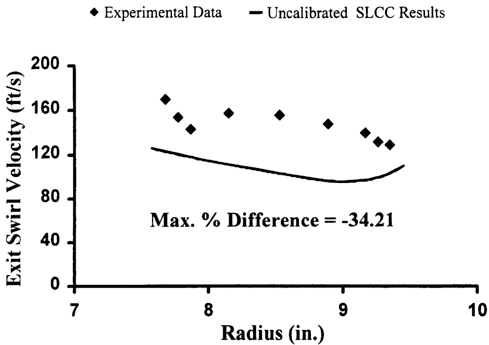
Figure 5.18. Radial Distribution of Exit Swirl Velocity for Stage 35 Stator.
