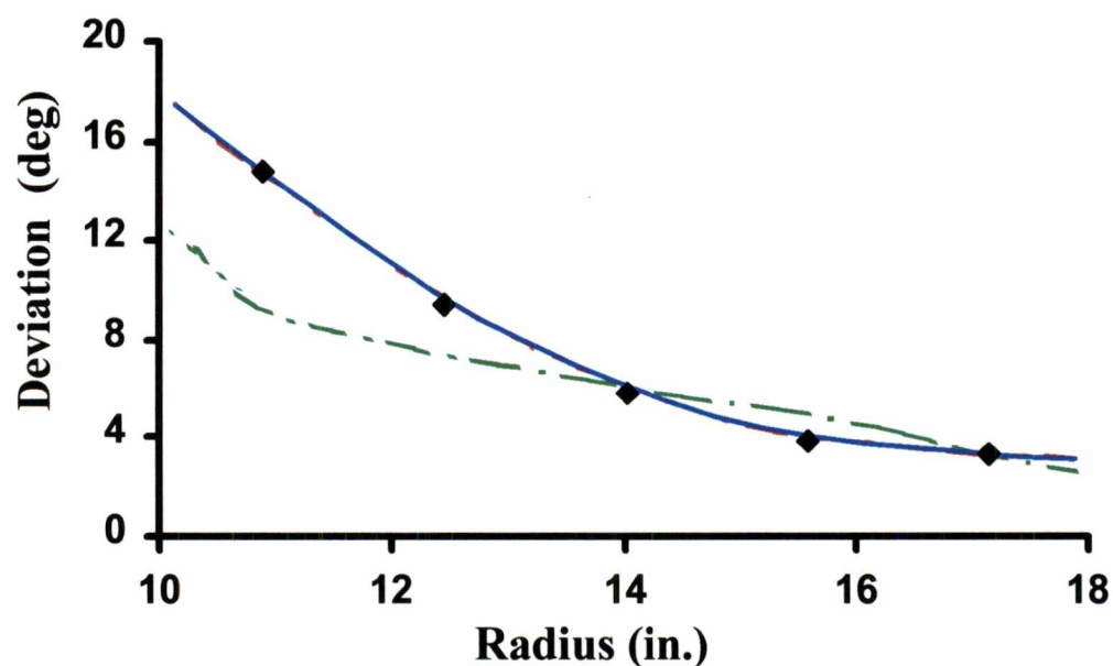
Figure 4.4. Radial Distribution of Deviation including Experimental Data, Uncalibrated Data, Partially Calibrated Data and Calibrated Data for Rotor 1B.
