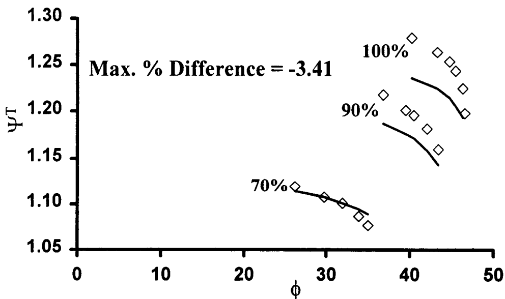
Figure 5. 4. 1-D Temperature Characteristic Map for Stage 35 with Rotor 1B Calibration Trends Included.
