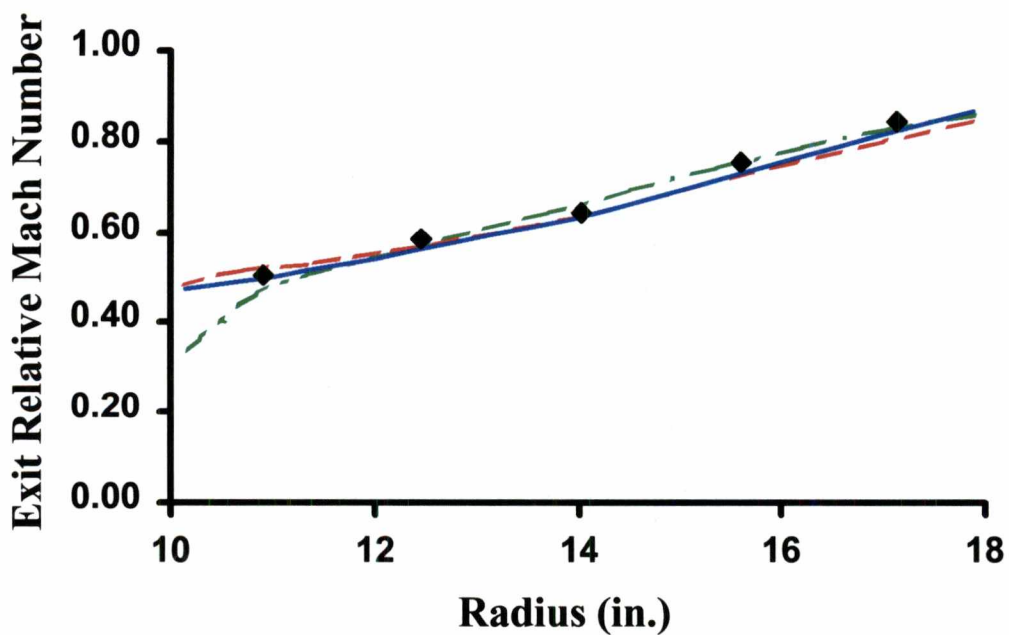
Figure 4.6. Radial Distribution of Exit Relative Mach Number including Experimental Data, Uncalibrated Data, Partially Calibrated Data and Calibrated Data for Rotor 1B.
