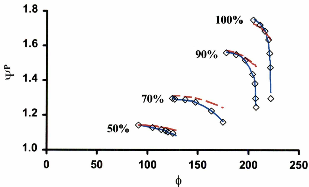
Figure 4.21. 1-D Pressure Characteristic Map for Rotor 1B.
