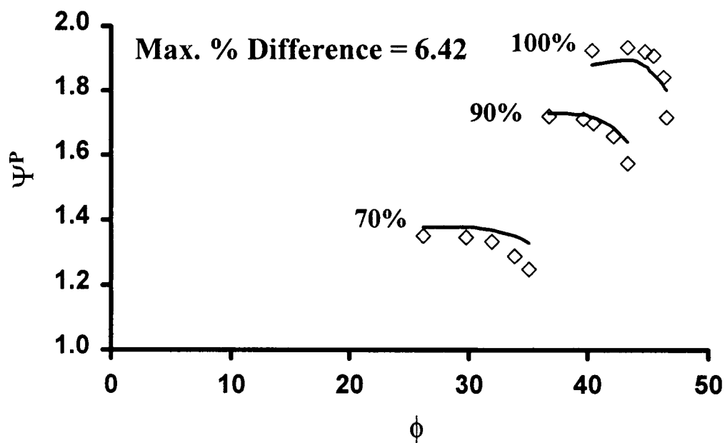
Figure 5.23. 1-D Pressure Characteristic Map for Stage 35.
