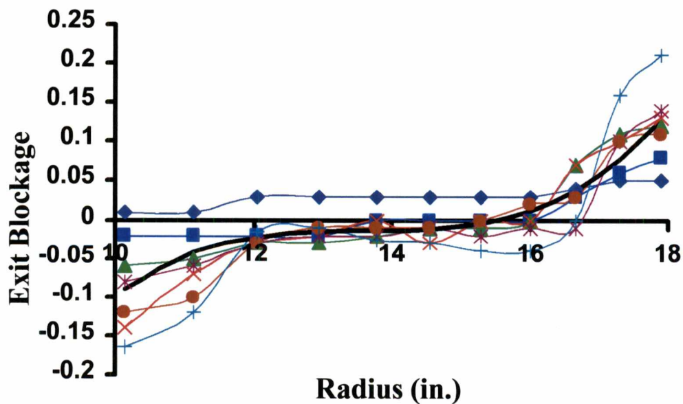
Figure 4.16. Radial Distribution of Exit Blockage at 100-Percent Speed for Various Mass Flows for Rotor1B.
