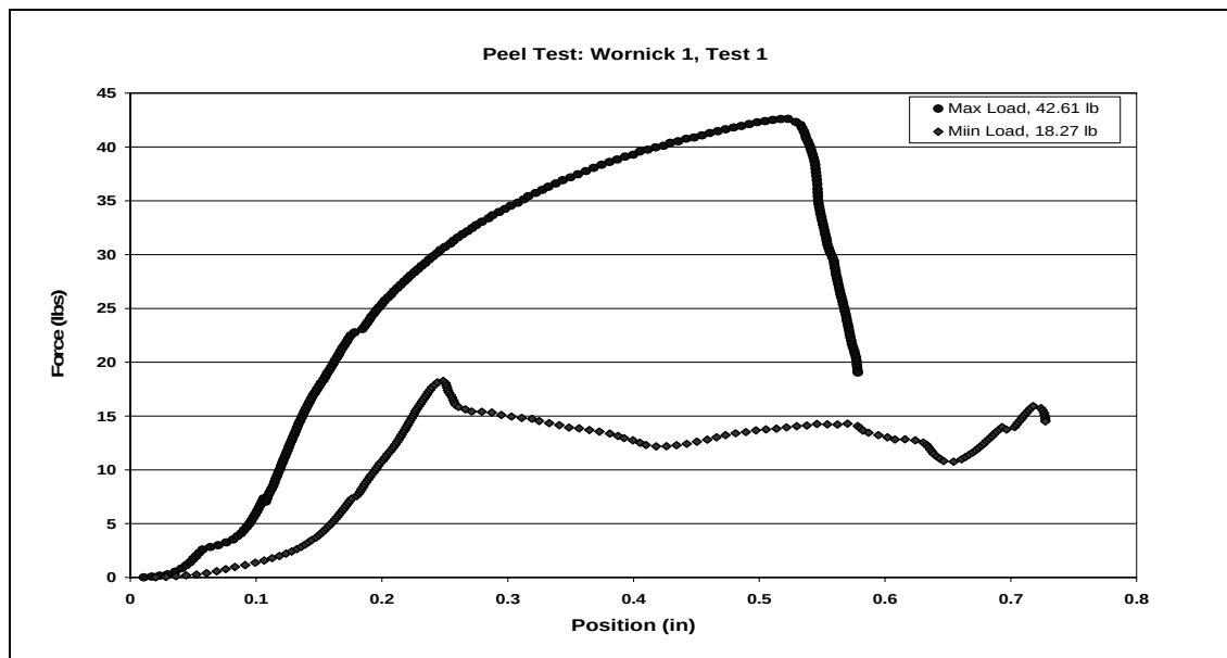
Figure 4.1: Plot of peel test data for Wornick 1 polytrays, Test 1; seals in good condition.
