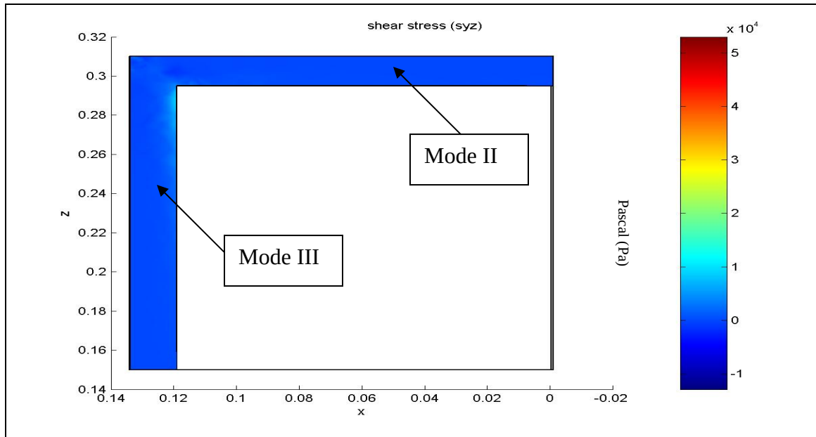
Figure 4.31: Cross-section plot of corner force simulation at 200 N load showing stress, \sigma_{yz} , in xz plane.
