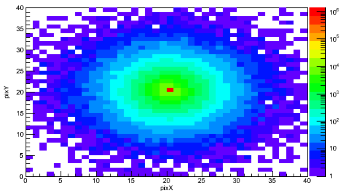
Figure 61. Spatial distribution of Geant4 simulated recoil nuclei after the first scattering event of 2 \times 10^6 Cf-252 energy spectrum neutrons with a pencil beam angular distribution centered on the center detector pixel in a detector pixel array.
