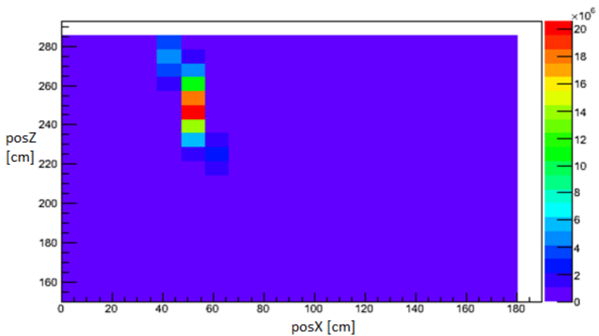
Figure 75. MLEM reconstruction of a single source at 250 cm distance with three detector positions separated by 56 cm.
