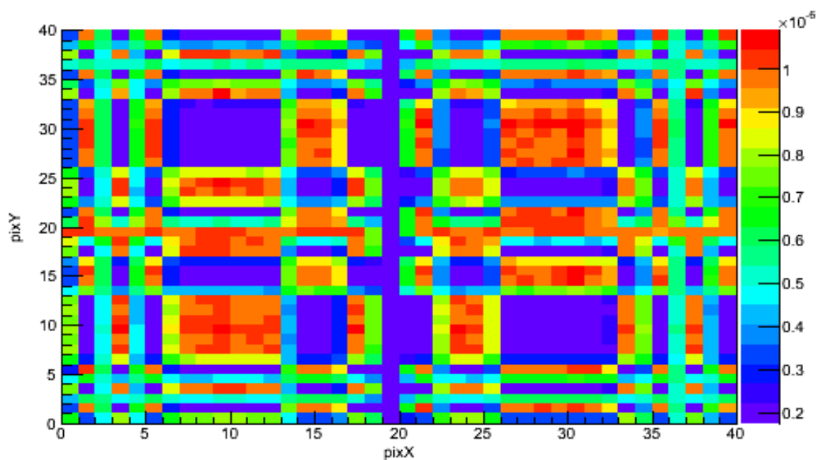
Figure 54. Normalized simulated projected mask data with no mask scattering. Simulation consisted of 4\text{E}9 Cf-252 spontaneous fission spectrum neutrons emitted isotropically and transported through a rank-19 mask. Simulation performed in Geant4.
