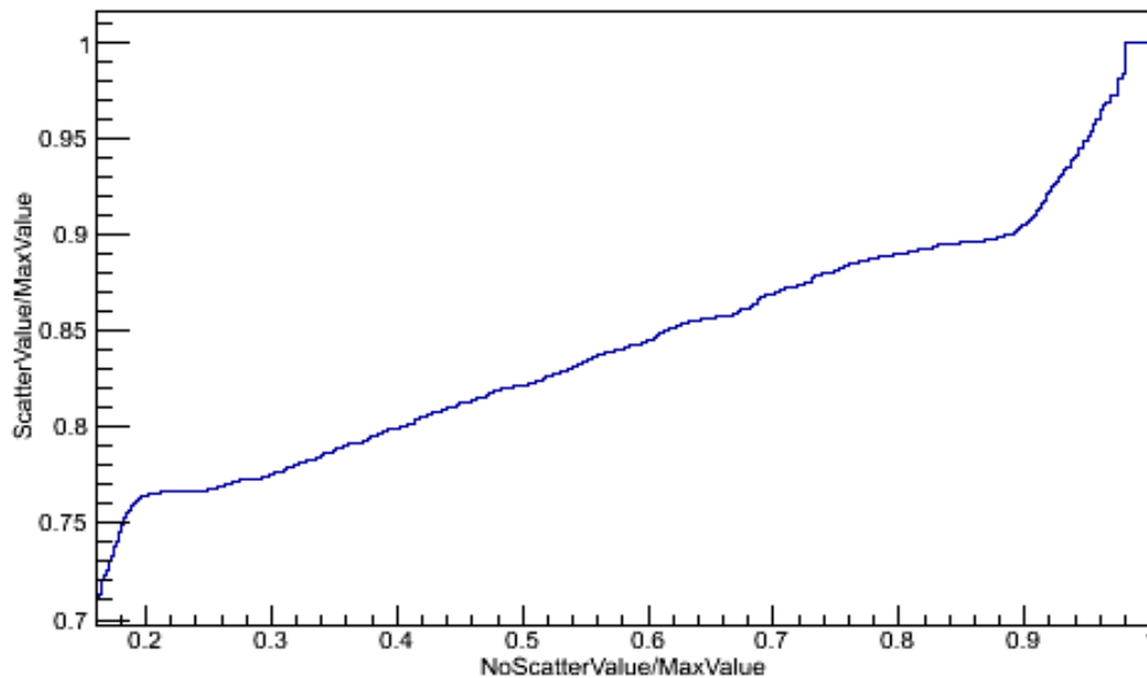
Figure 57. Transfer Function from simulation excluding scattering within the mask to simulation including scattering within the mask
