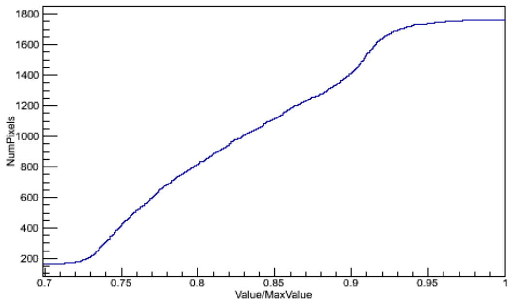
Figure 56. Cumulative histogram of simulated data with scattering in the mask
