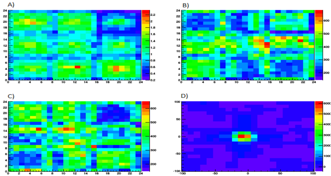
Figure 16. Measured data and reconstructed in focus source using cross-correlation reconstruction. A) No-mask (void) measured data. B) Mask measured data. C) Anti-Mask measured data. D) Reconstructed Image. Data is intentionally reconstructed at the correct distance.
