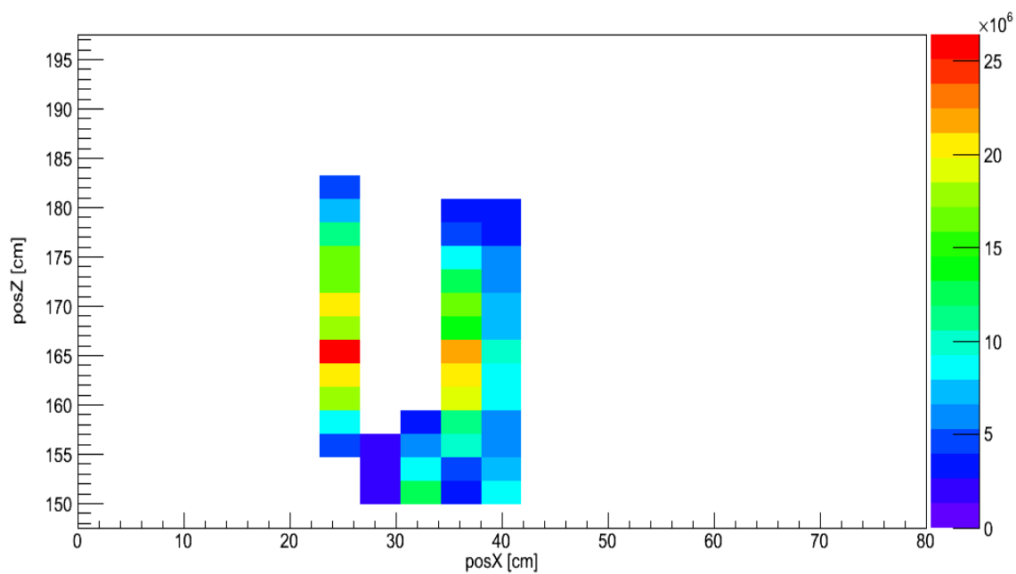
Figure 108. MLEM Reconstruction of two 11.1 \mu\text{Ci} Cf-252 point sources, one at (22.8,165), the other at (33.8,165) from 90 minute measurements with a shift between measurements on the orthogonal axis of 69 cm.
