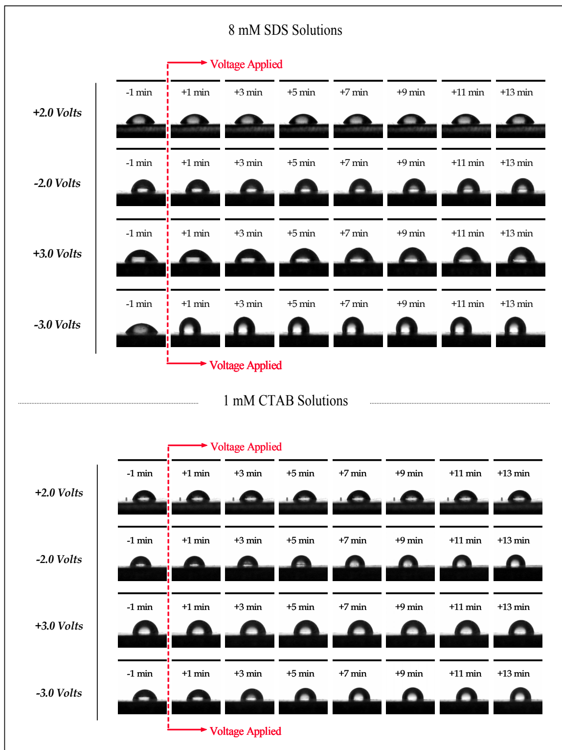
Figure 3. Selected Droplet Images for PMPS in SDS and CTAB Solutions
