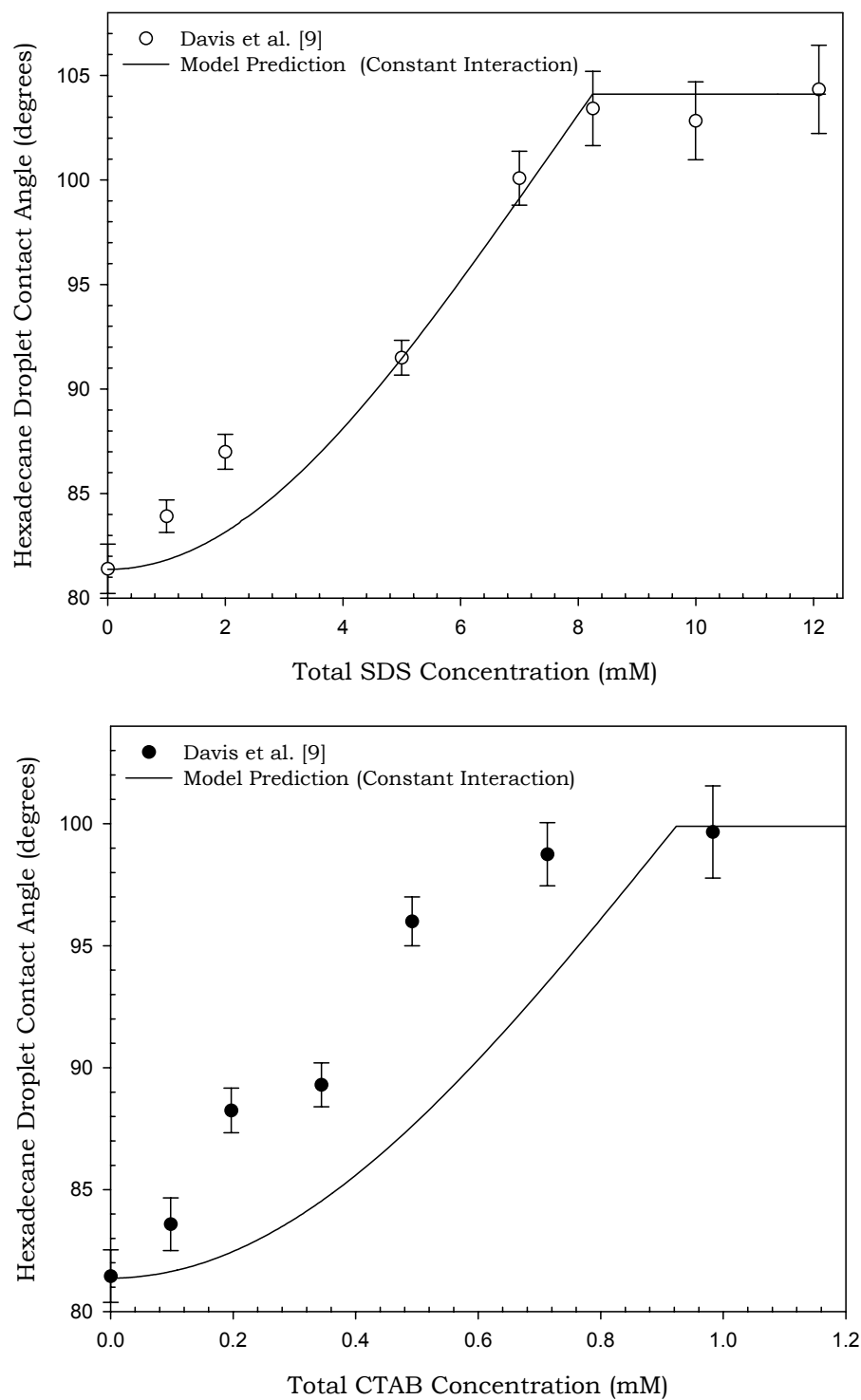
Figure 6. Contact Angle Prediction Based on the Quasi-Chemical Approximation with Constant Lateral Interactions
