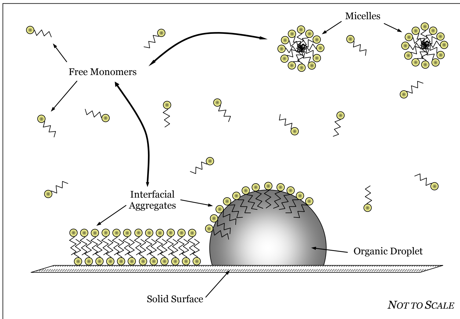
Figure 1. Simplified Surfactant Solution Cleaning System
