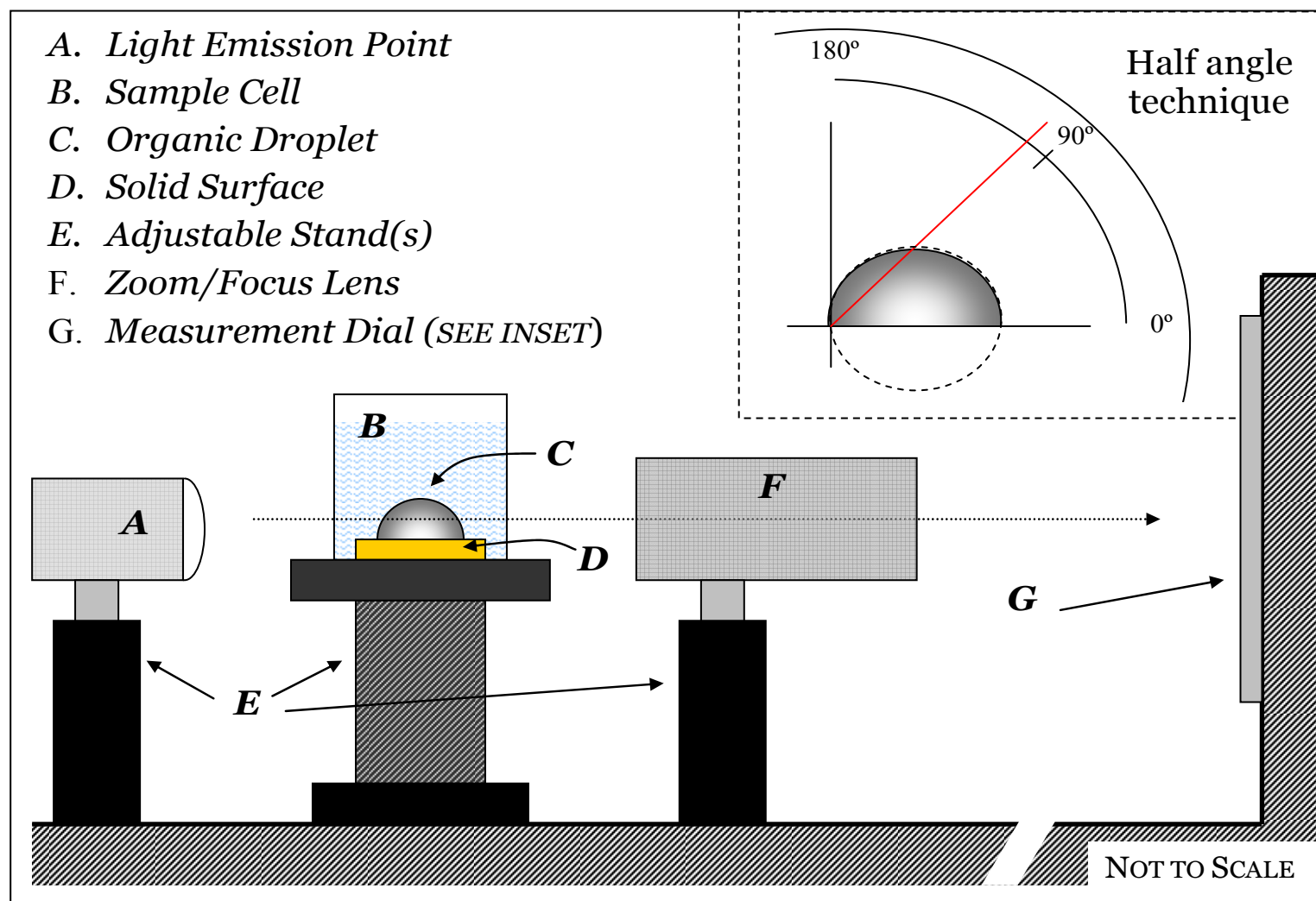
Figure 4. Contact Angle Measurement Apparatus
