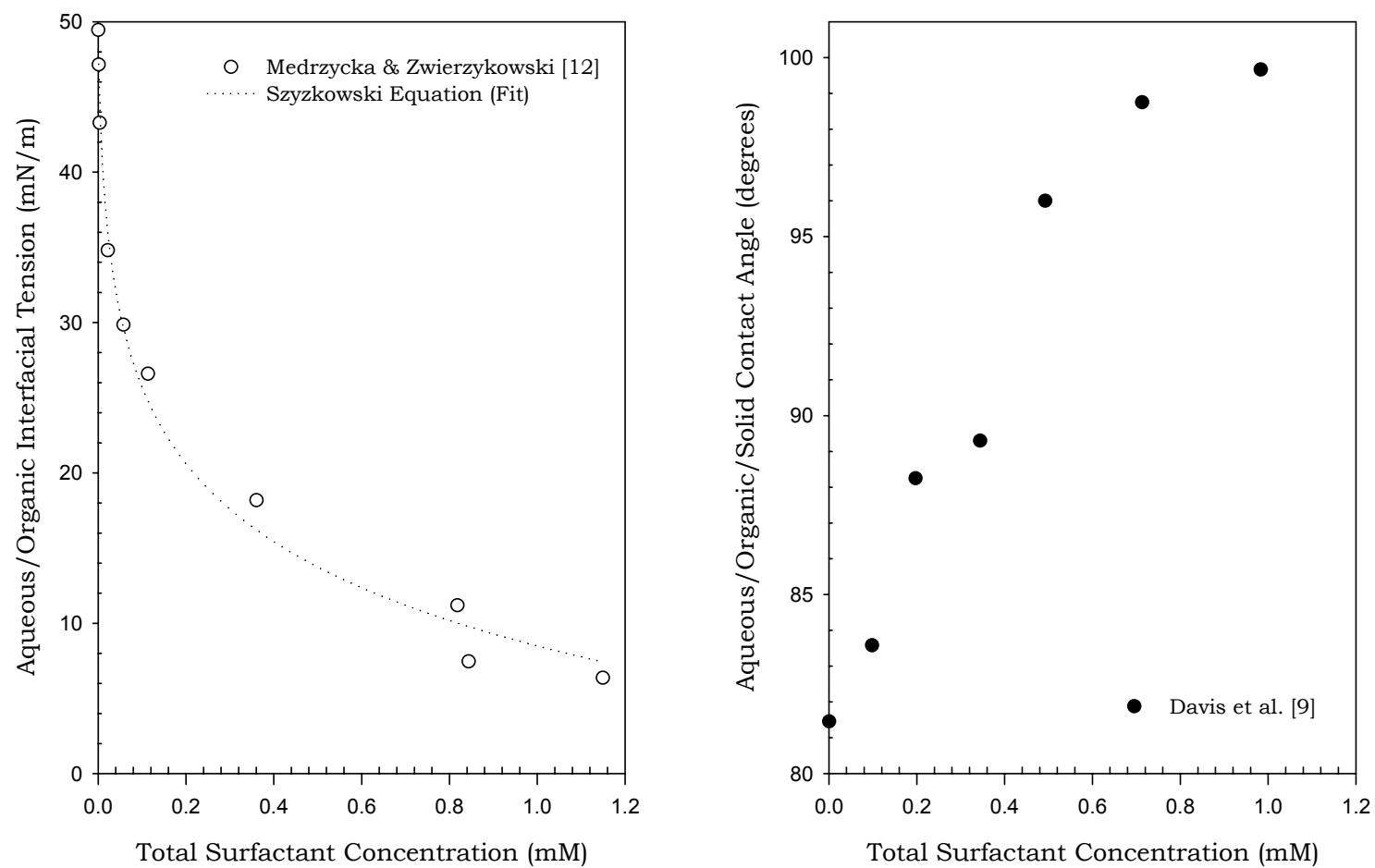
Figure 2. Interfacial Tension and Contact Angle Data for Hexadecane/CTAB Solution
