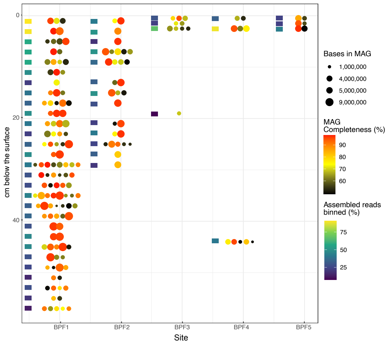
Figure 4-2: MAG size, completeness and assembled reads binned per sample depth.
