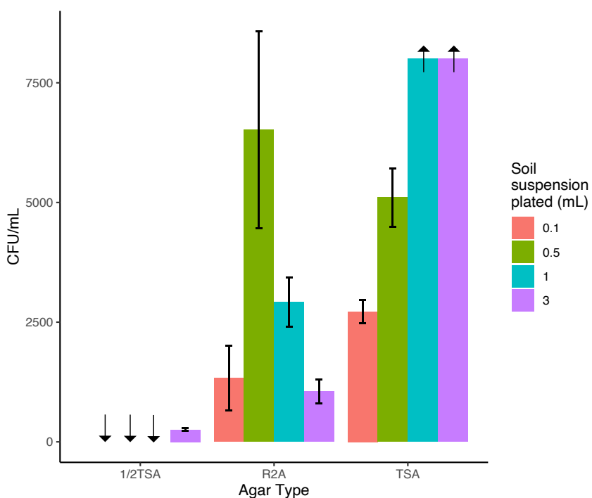
Supplemental Figure 3-1: Preliminary testing for mean CFU/mL from agars \frac{1}{2} TSA, R2A, and TSA with surface soil from BPF2.
