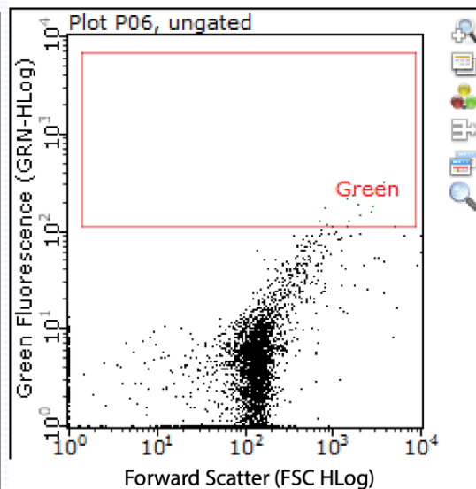
Supplemental Figure 2-4: Cell staining and flow cytometer.
