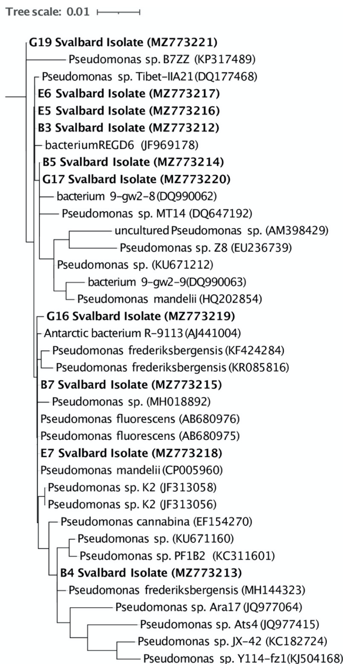
Figure 3-4: Full length 16S rRNA from Svalbard isolates phylogenetically compared to other Pseudomonas isolates
