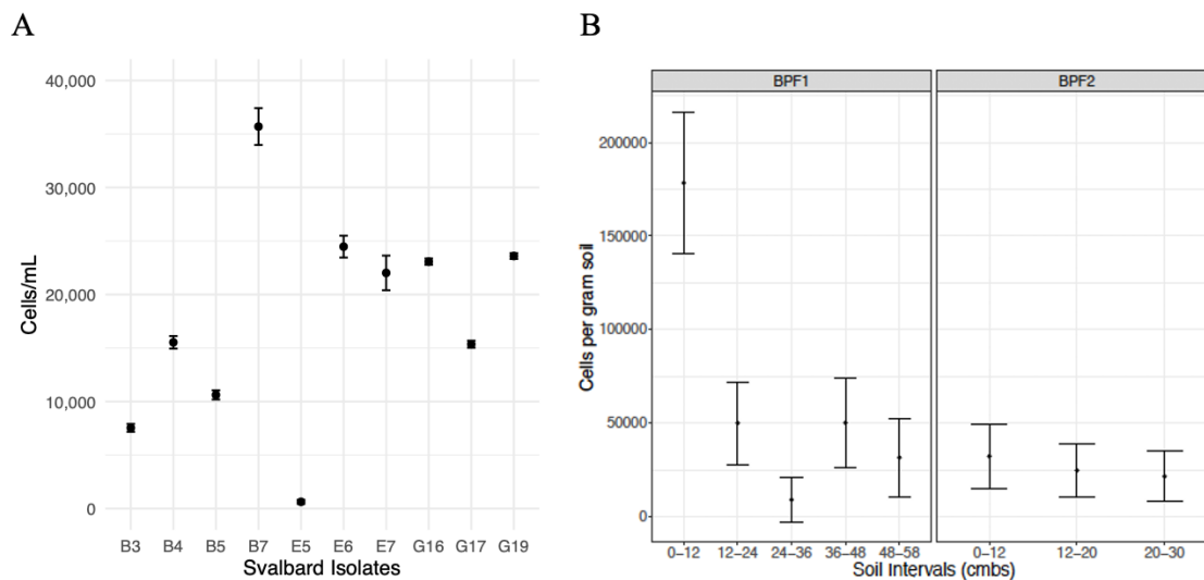
Supplemental Figure 3-5: Direct microscopic cell counts in A) 1mL of culture broth of Svalbard isolates, and B) Bulk soil. Cells were stained with SYBR Gold and 30 random fields of view were averaged for each sample. Error bars show one standard deviation about the mean.
