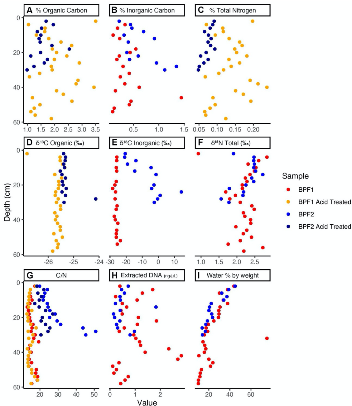
Figure 3-2: Elemental Analysis of acidified and non-acidified soil.
