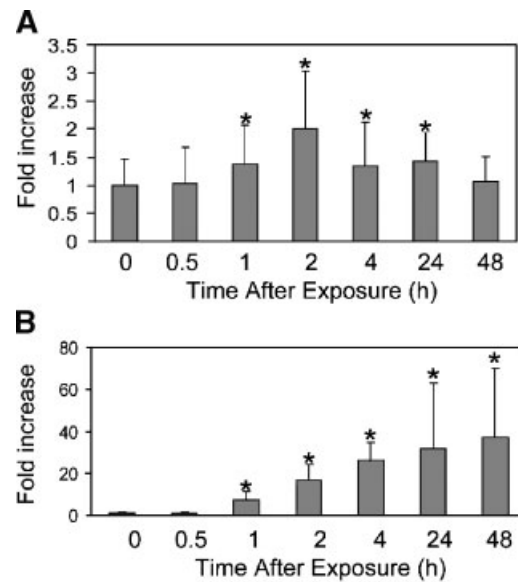
Figure 2. Time course of Slug and Snail mRNA induction. RNA from SCC 12F cells was collected at the indicated times after exposure to 300 J/m 2 and Slug (A) and Snail (B) mRNA levels were measured as described in Materials and Methods. For each experiment, three independent samples were included in each treatment group. Values for each sample were normalized to GAPDH levels. In each experiment, the baseline level of Slug or Snail in untreated cells was defined as 1.0 and other values were expressed as fold induction. Data shown represent the mean of nine independent samples \pm standard deviation examined in three separate experiments. * P \leq 0.05 compared to unexposed cells.
