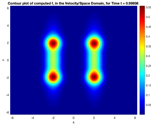
Figure 6: Numerical Solution
