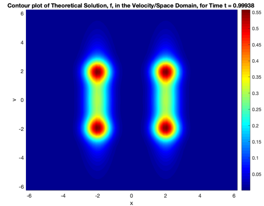
Figure 7: Theoretical Solution
