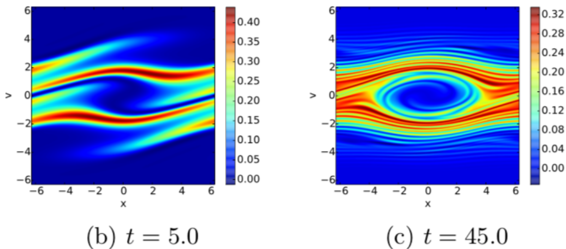
Figure 12: Two Stream Instability test case. Figure taken from Garrett & Hauck paper.
