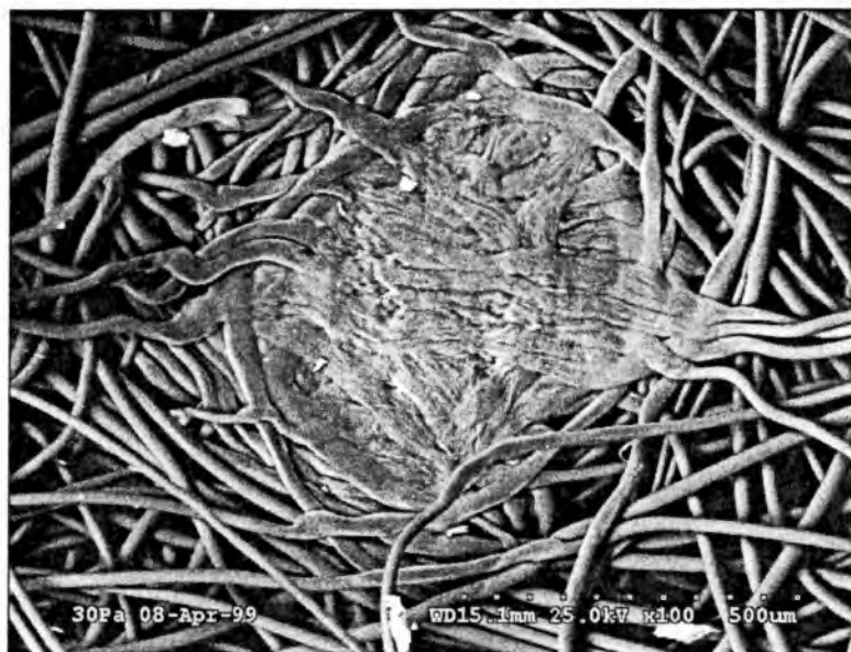
Figure 4.18 SEM Image of a Bond for Drawn 1 Fibers at 145 °C Bonding Temperature
