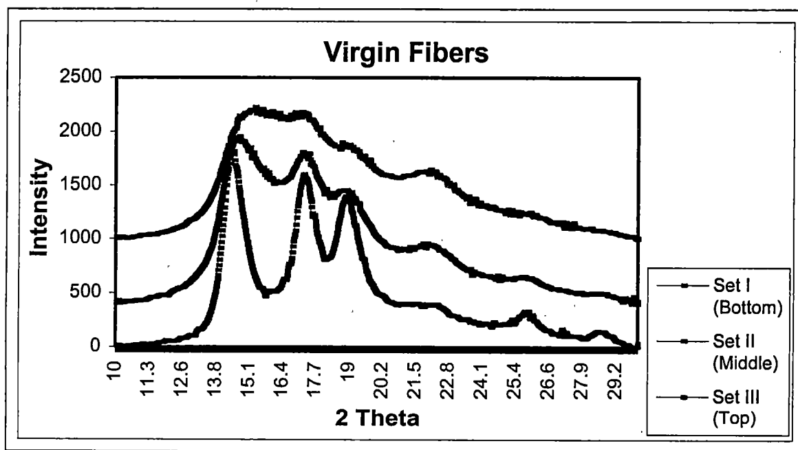
Figure 4.31 WAXD Equatorial Scans of Virgin Spunbond Fibers
