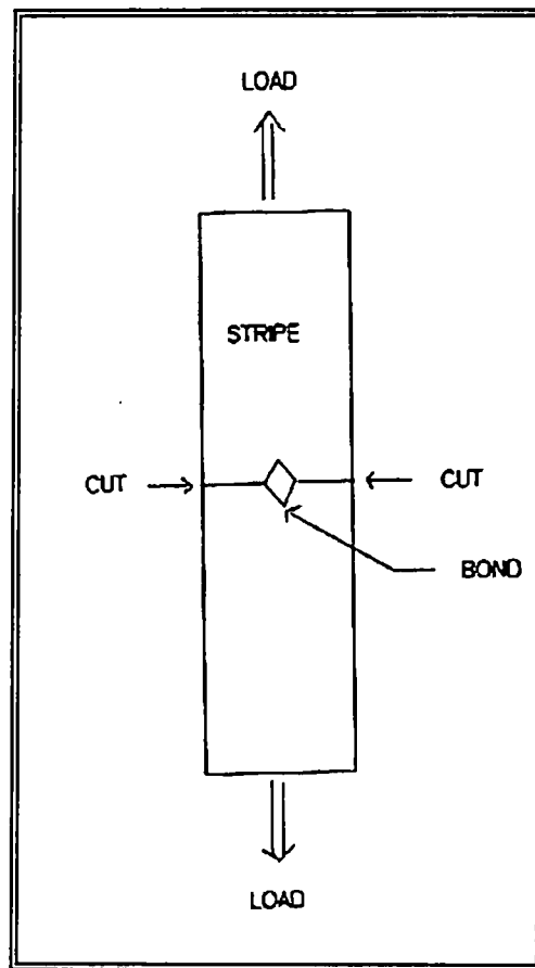
Figure 3.3 Schematic of Single-Bond Strip Tensile Test
