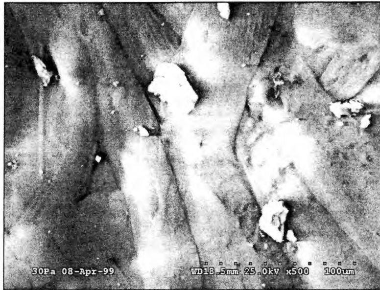
Figure 4.15 SEM Image of a Bond for As-spun 1 Fibers at Higher Magnification (x500)
