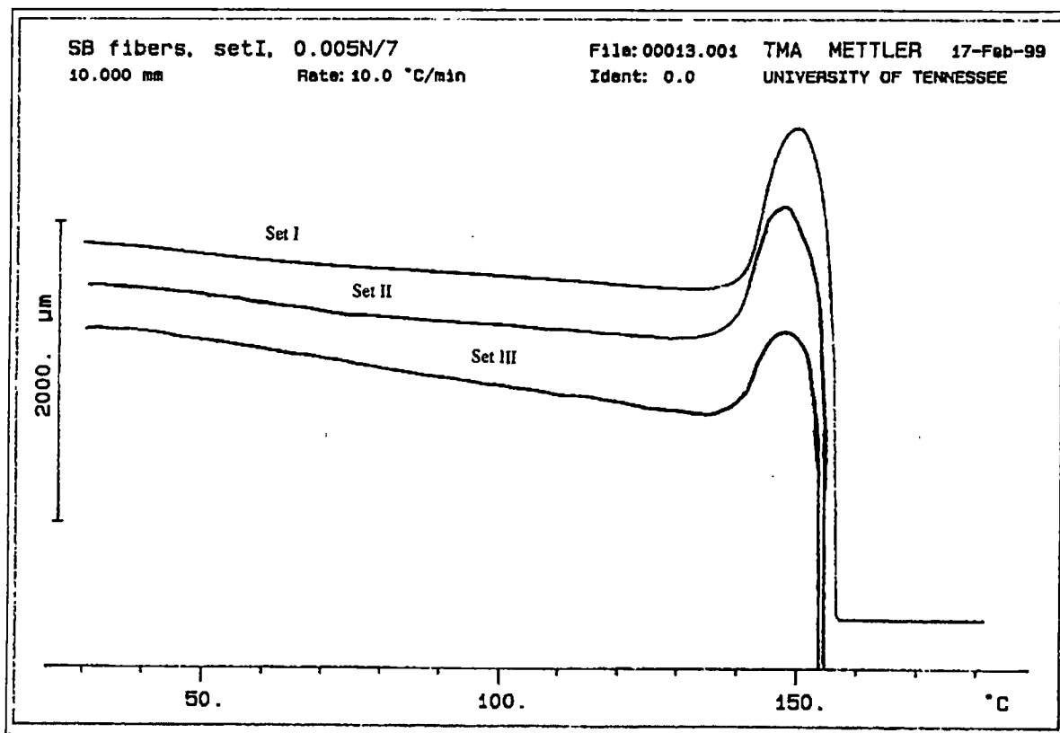
Figure 4.21 Thermo-mechanical Responses of Spunbond Fibers at Low (a) and High (b) Tension
