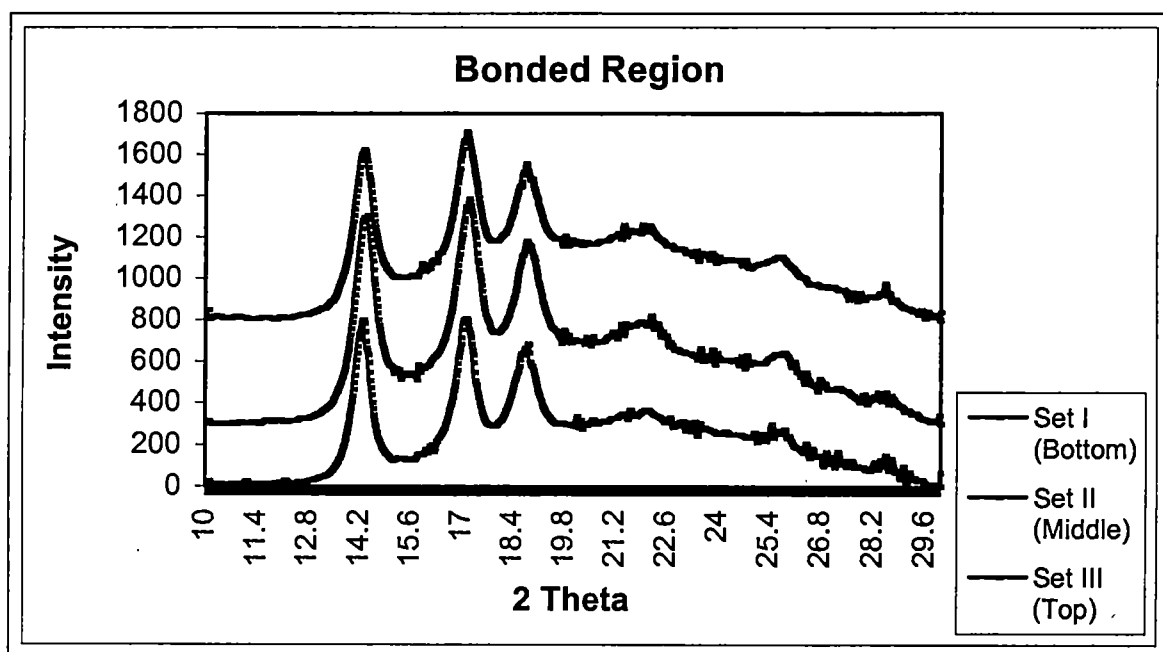
Figure 4.33 WAXD Equatorial Scans of Bonded Regions (Spunbond)
