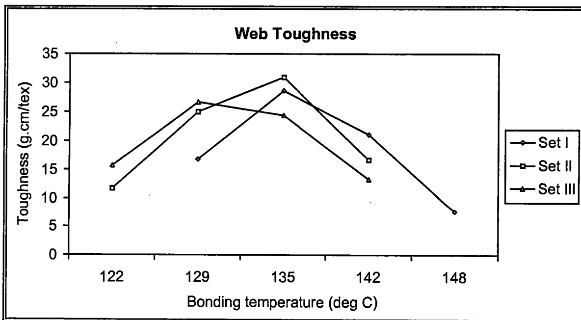
Figure 4.27 Toughness vs Bonding Temperature for Spunbond Webs
