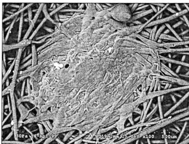
Figure 4.19 SEM Image of a Bond for Drawn 1 Fibers at 155 °C Bonding Temperature
