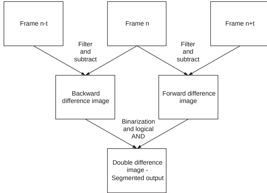
Figure 3.3: Double difference image – Motion based segmentation
