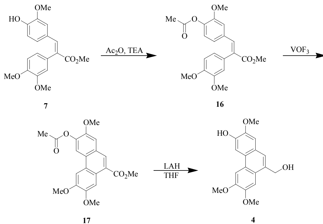
Scheme 7. Alternative route for free hydroxy tylophorinine synthesis
