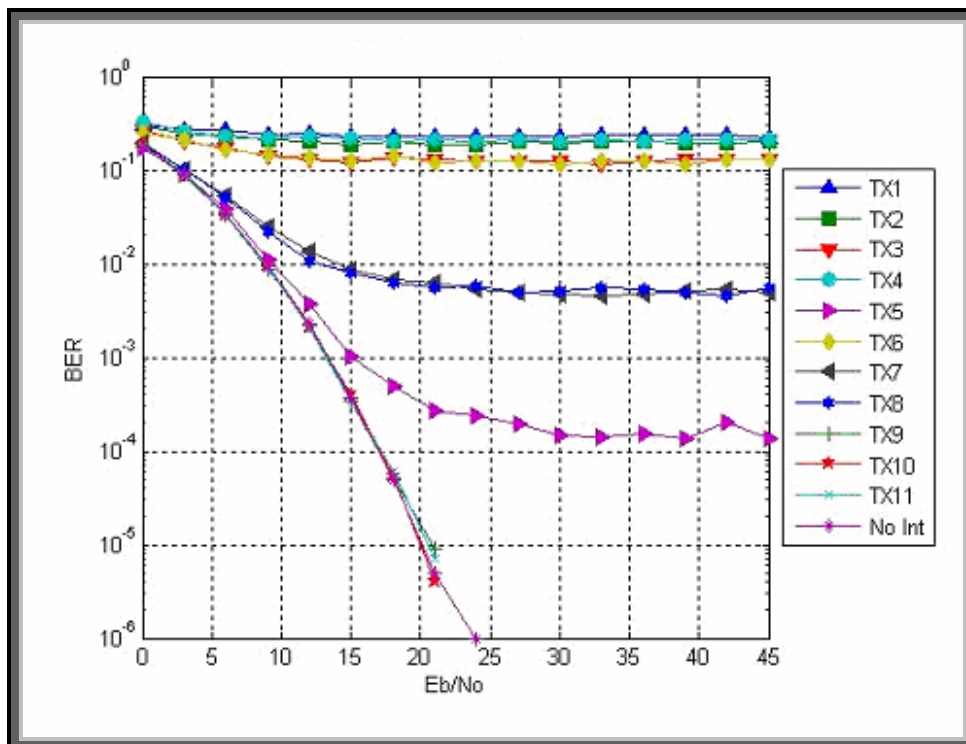
Figure 5.12 – Zigbee Transmitter #7 with Wifi Interferers
