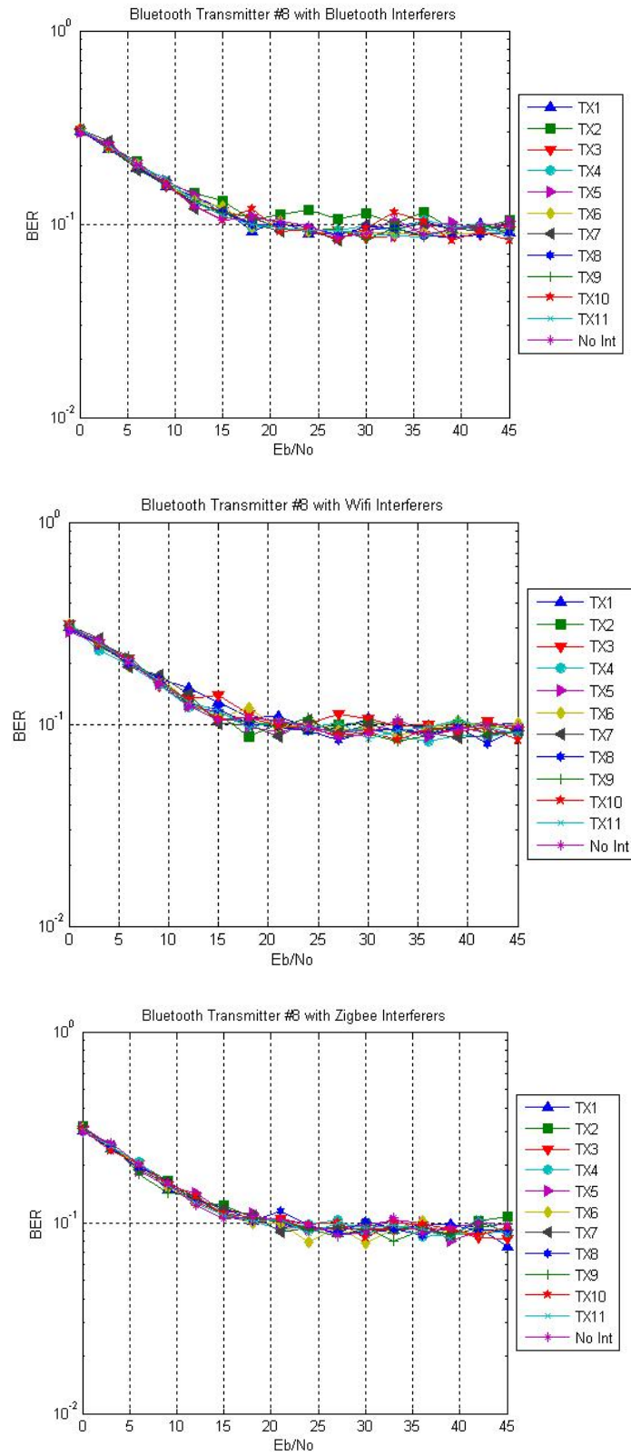
Figure A.8 - Bluetooth Tx #8
