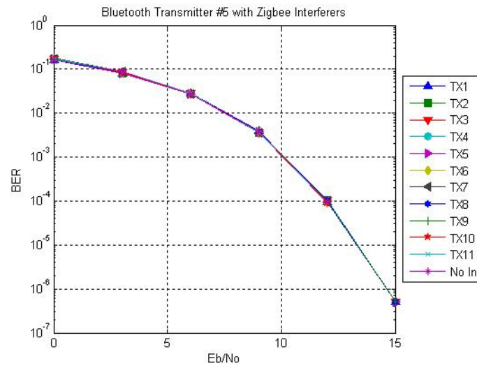
Figure A.5 - Bluetooth Tx #5
