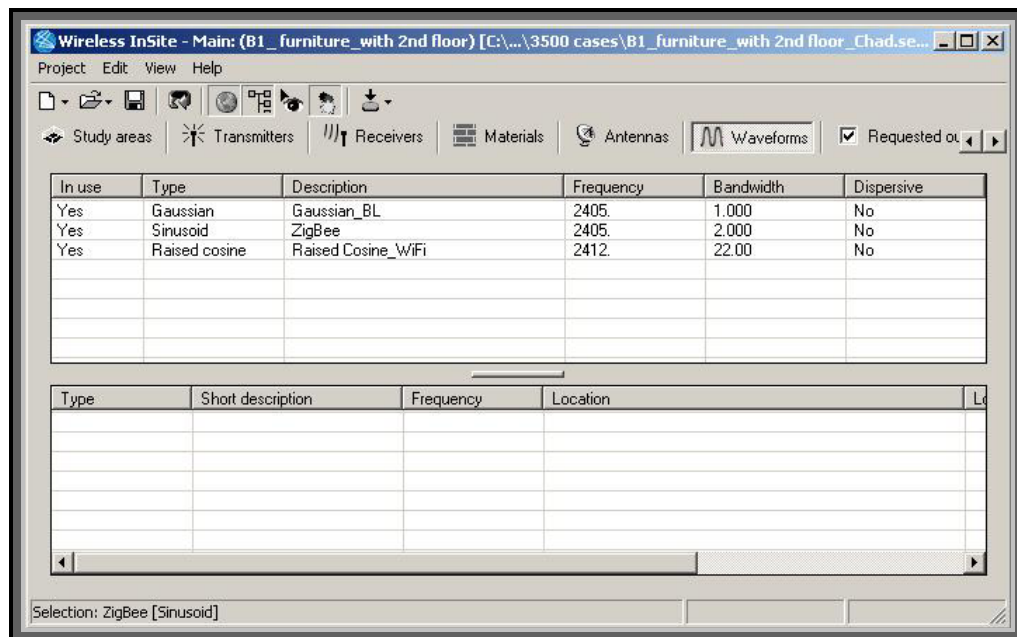
Figure 5.2 – Waveform Properties
