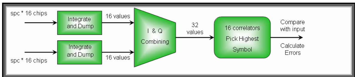
Figure 3.3 - Zigbee Receiver
