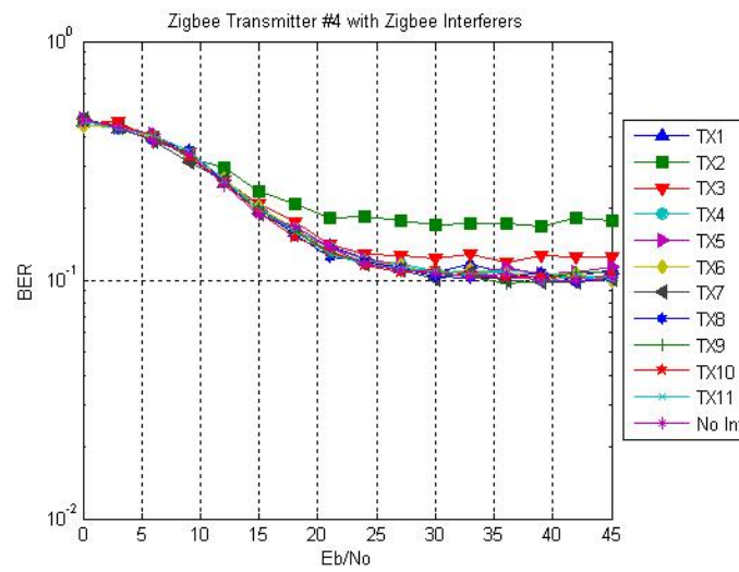
Figure A.26 - Zigbee Tx #4
