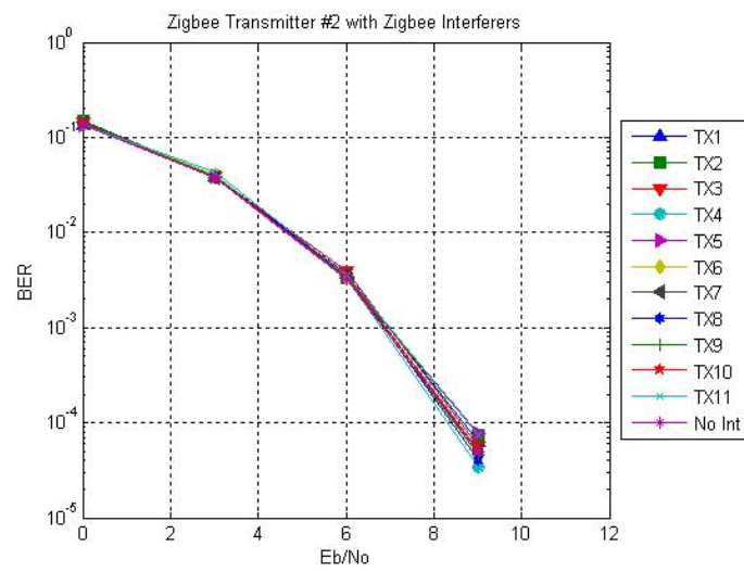
Figure A.24 - Zigbee Tx #2
