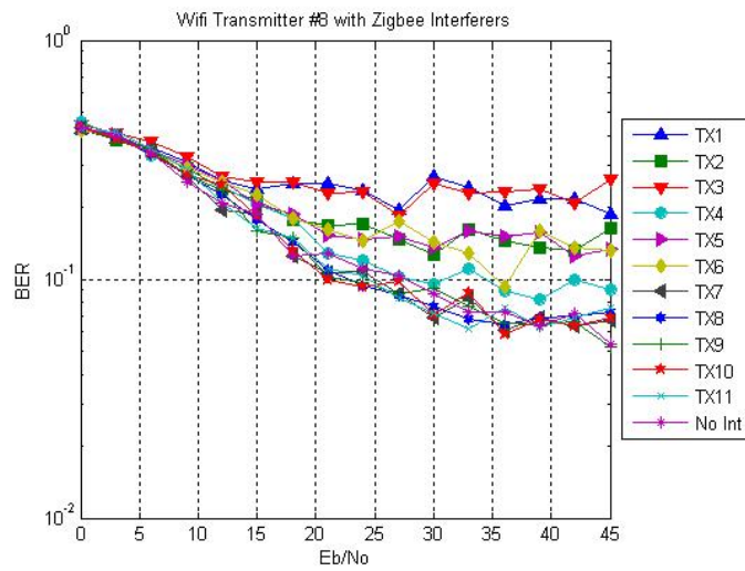
Figure A.19 - Wifi Tx #8
