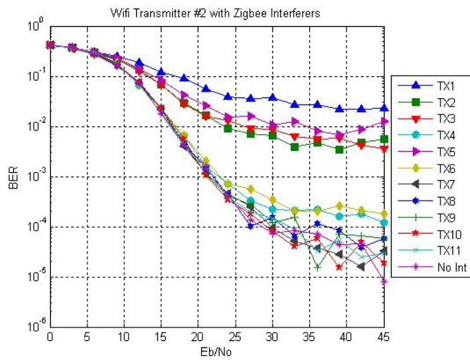
Figure A.13 - Wifi Tx #2
