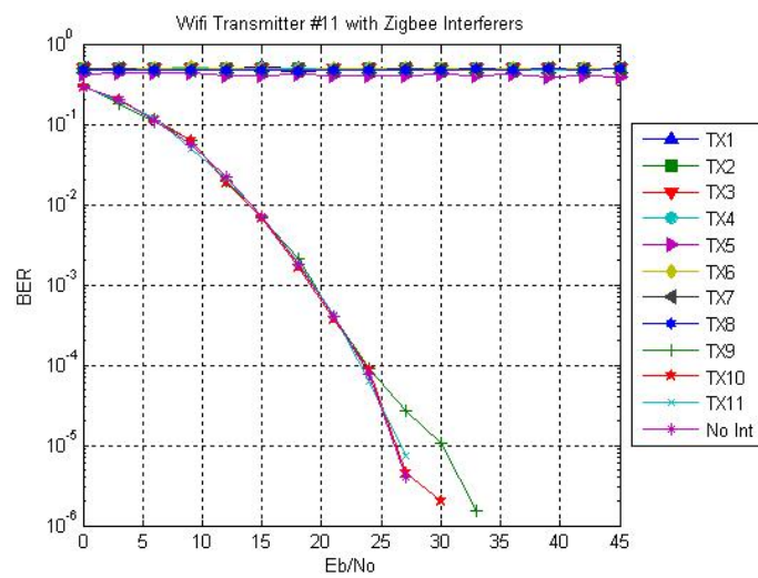
Figure A.22 - Wifi Tx #11
