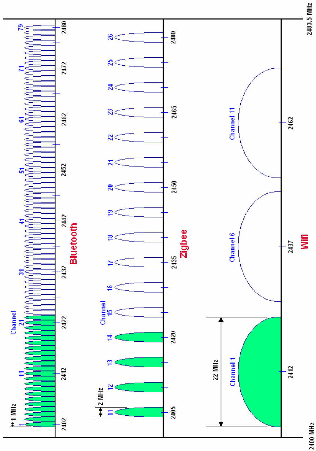
Figure 3.14 - Channel Assignments
