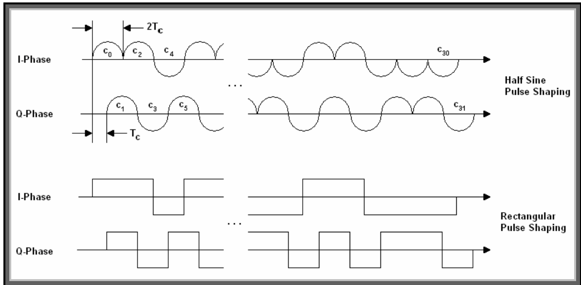
Figure 3.2 – Chip Sequence Separation with Half-Sine Pulse Shaping
