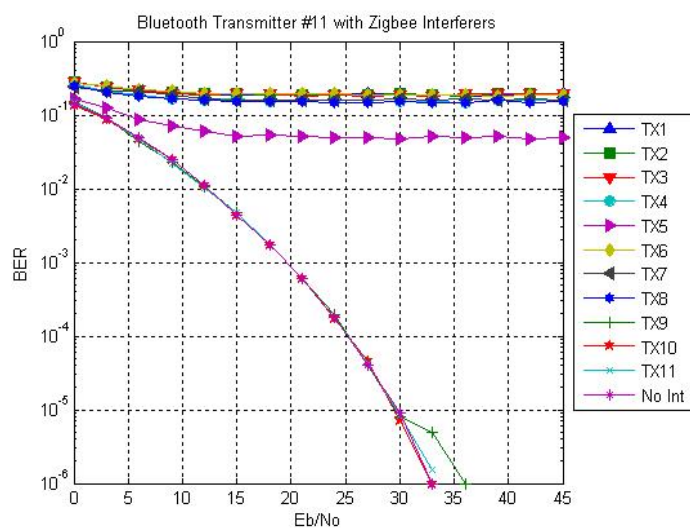
Figure A.11 - Bluetooth Tx #11
