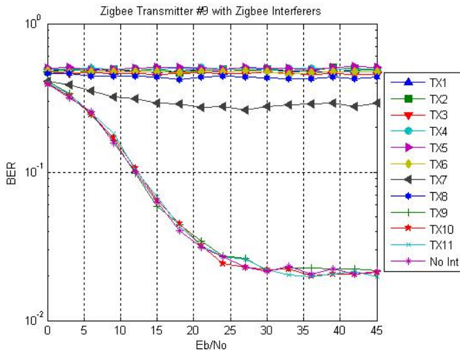
Figure A.31 - Zigbee Tx #9
