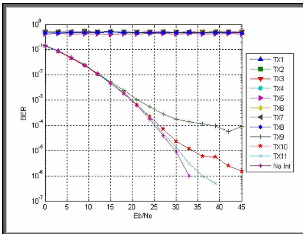
Figure 5.25 – Bluetooth Transmitter #11 with Bluetooth Interferers
