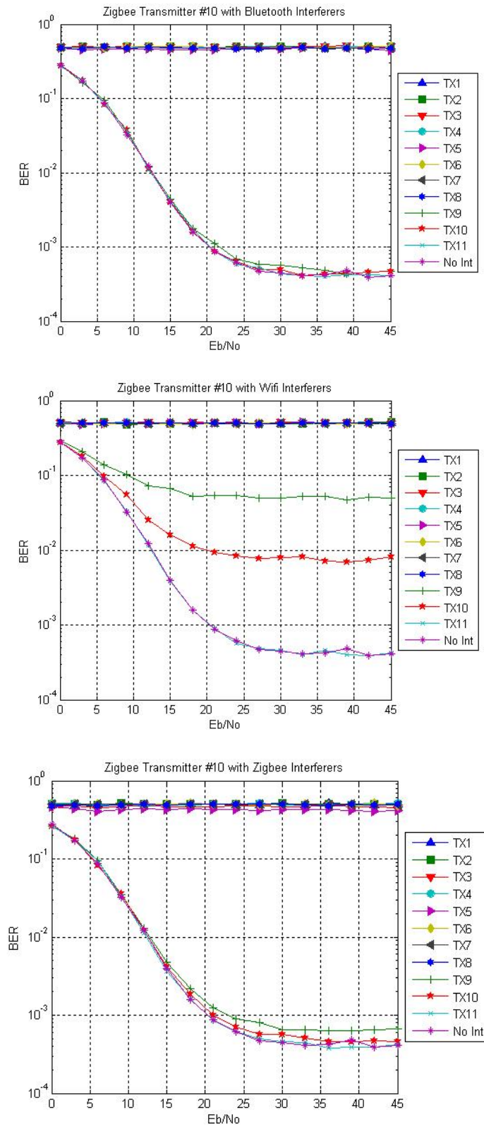
Figure A.32 - Zigbee Tx #10
