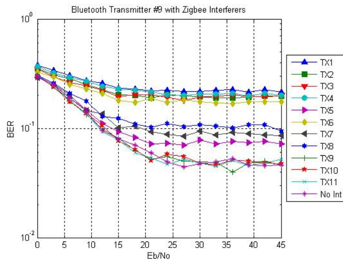
Figure A.9 - Bluetooth Tx #9
