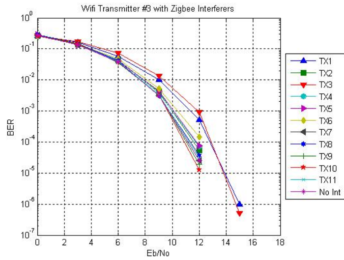
Figure A.14 - Wifi Tx #3
