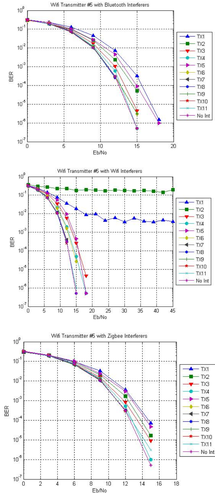
Figure A.16 - Wifi Tx #5
