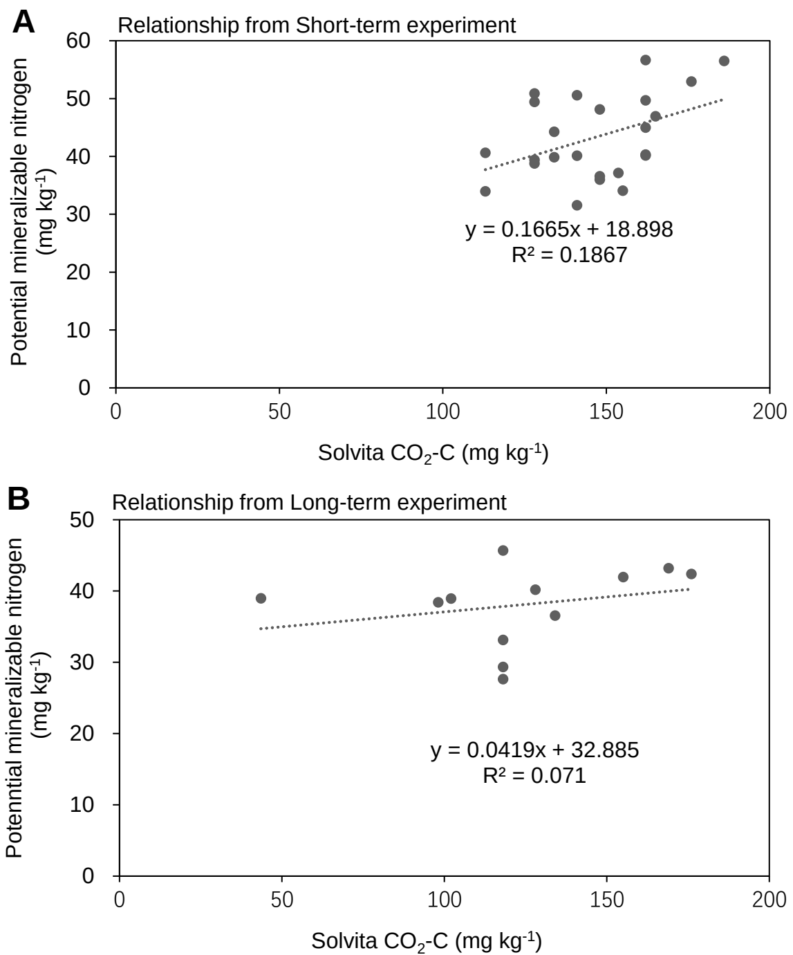
Figure C-5 Relationship between Solvita 1-day CO 2 -C and 7-day potential mineralizable nitrogen. (A) Relationship from the short-term experiment. (B) Relationship from the long-term experiment.
