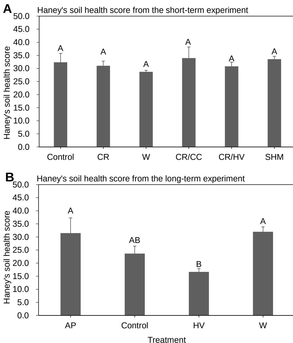
Figure C-6 Haney's soil health score under different CC treatment in the short-term and long-term experiments. (A) Haney's soil health score from short-term experiment. CR-Cereal Rye, W-Wheat, CC-Crimson Clover, HV-Hairy Vetch, SHM-Soil Health Mix. (B) Haney's soil health score from long-term experiment. AP-Austrian Winter Pea. Different letters denote statistically different means at P < 0.05 and error bars represent standard error of the mean.
