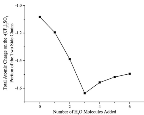
Fig. 8. Total atomic charge as computed with the CHelpG routine residing on the -(CF_2)_2SO_3 terminal portions of the side chains in the EW 590 system as a function of the number of added water molecules. The charge becomes significantly more negative after the addition of two water molecules where first proton dissociation was observed and undergoes an additional considerable decrease after second proton dissociation occurs upon addition of three water molecules.
