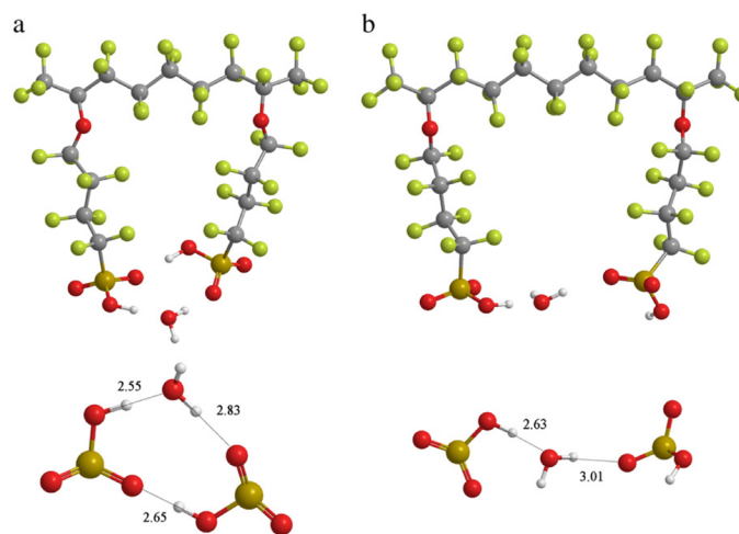
Fig. 2. Optimized (B3LYP/6-311G**) global minimum energy structures of two side chain oligomeric fragments of 3M PFSA polymer with fully extended PTFE backbones upon addition of one water molecule with the hydrogen bonding between hydrophilic groups and water molecules illustrated in the bottom panels: (a) the EW 590 system which maintains a single direct hydrogen bond between the sulfonic acid groups as well as a hydrogen bond 'bridge' between sulfonic acid groups via the additional water molecule; (b) the EW 690 system where the water molecule draws the side chain hydrophilic groups closer together via hydrogen bond connectivity but no direct hydrogen bonding between sulfonic acid groups occurs.
