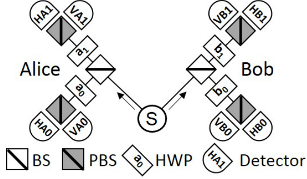
Figure 1.1: A typical Bell test. An entangled photon pair is shared between Alice and Bob whose local measurement settings or local realities a_0, a_1, b_0 , and b_1 are randomly chosen by a symmetric beamsplitter (BS). HWP \equiv half-wave plate, PBS \equiv polarizing beamsplitter
