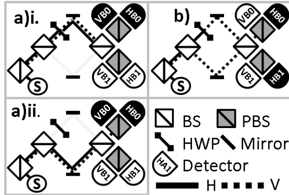
Figure 2.13: a) Indistinguishable cases (i) and (ii) lead to de Broglie Interference observed in Bob's interferometer by detectors VB0 and HB0. b) Indistinguishable photons incident on different ports of a beamsplitter lead to Hong-Ou-Mandel interference observed as a dip in different port coincidences.
