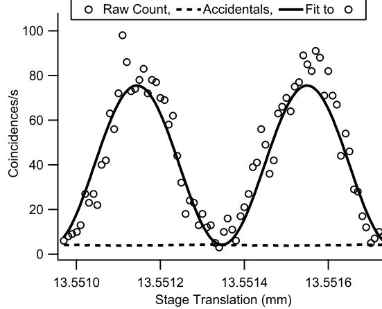
Figure 2.2: Non-Local Franson Interference for detectors HA0 and HB1 with 99.6 \pm 2.6\% corrected visibility and a 89.5 \pm 2.3\% raw visibility. This data was collected using a preliminary Mach-Zehnder experiment.
