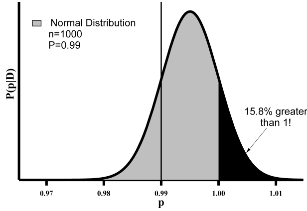
Figure 4.2: The Normal distribution does not conform to the probability upper bound of 1. This distribution suggests that there is a 15.8% chance the probability is greater than 1! This behavior is undesirable.
