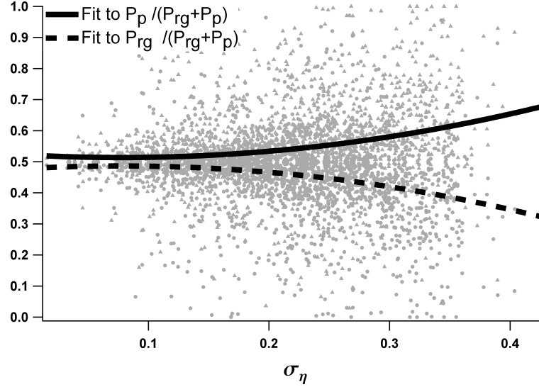
Figure 4.6: Given the efficiencies, the proposed distribution outperforms the ratio-Gaussian distribution, on average, as asymmetries in the efficiencies increase, as measured by the efficiency standard deviation \sigma_\eta .
