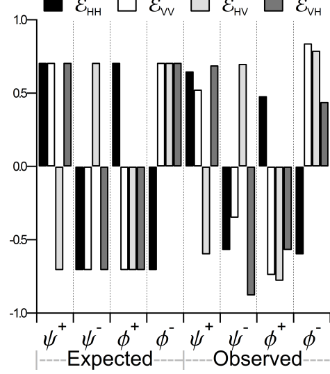
Figure 2.11: Expected and observed values for the correlation coefficients \mathcal{E}_{HH} , \mathcal{E}_{VV} , \mathcal{E}_{HV} , and \mathcal{E}_{VH} in the CHSH configuration for each Bell state. Standard deviations for these coefficients are \leq 0.06 .
