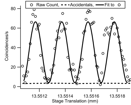
Figure 2.15: Local de Broglie Interference observed in Bob's interferometer by detectors VB0 and HB1 with 98 \pm 4\% corrected visibility and a 88.8 \pm 3.5\% raw visibility.
