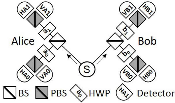
Figure 2.9: A typical Bell test. An entangled photon pair is shared between Alice and Bob whose local measurement settings or local realities a_0, a_1, b_0 , and b_1 are randomly chosen by a symmetric beamsplitter.
