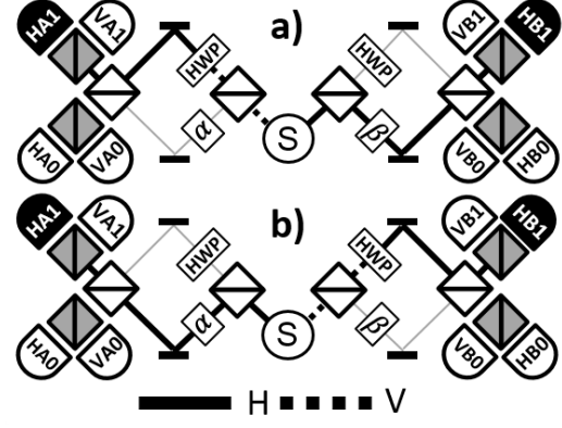
Figure 2.4: Nonlocal interference observed for an identical polarization event HA1HB1 is due to indistinguishable cases a) and b).
