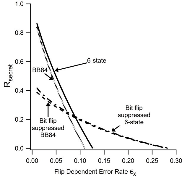
Figure 3.3: Secret key rates in the limit of perfect error correction versus the flip dependent error rate \epsilon_x for the 6-state and BB84 protocols given the depolarizing channel or with bit flip suppression. A fixed accidental error rate \epsilon = 0.01 has been assumed.
