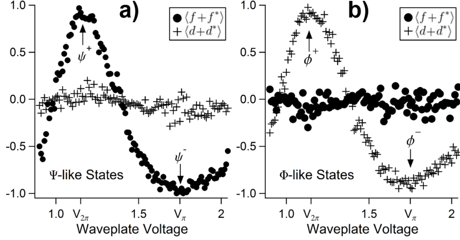
Figure 2.8: a) Variation of phase \theta in state \psi(\theta) \propto HV + e^{i\theta}VH using a liquid crystal waveplate. b) Variation of phase \gamma in state \phi(\gamma) \propto HH + e^{i\gamma}VV using a liquid crystal waveplate.
