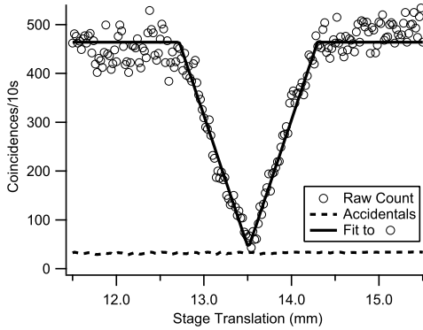
Figure 2.14: Hong-Ou-Mandel Dip in Bob's Interferometer with 97.8 \pm 0.5\% corrected visibility and a 91 \pm 0.5\% raw visibility.
