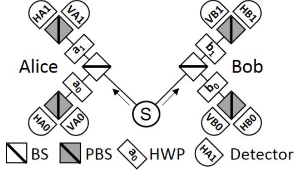
Figure 4.1: A typical Bell test. An entangled photon pair is shared between Alice and Bob whose local measurement settings or local realities a_0, a_1, b_0 , and b_1 are randomly chosen by a symmetric beamsplitter (BS). HWP \equiv half-wave plate, PBS \equiv polarizing beamsplitter
