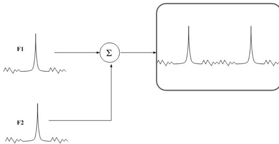
Figure 3.7 Spectrum of adder output [Carr]
