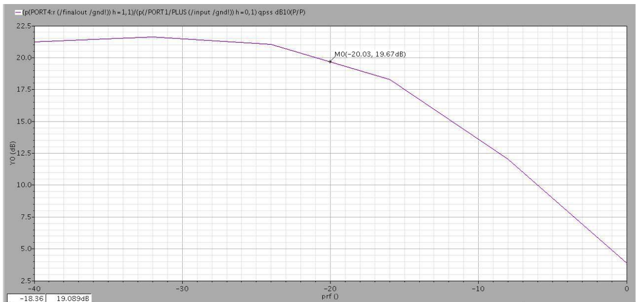
Figure 4.14 Power gain of the complete circuit
