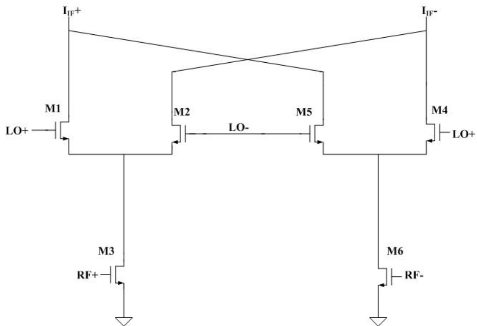
Figure 3.13 Double balanced Gilbert cell mixer [Ding]
