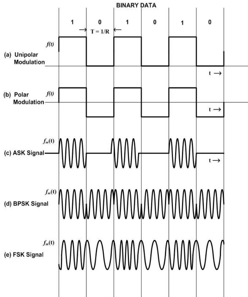
Figure 2.3 Bandpass digitally modulated signals [Couch]
