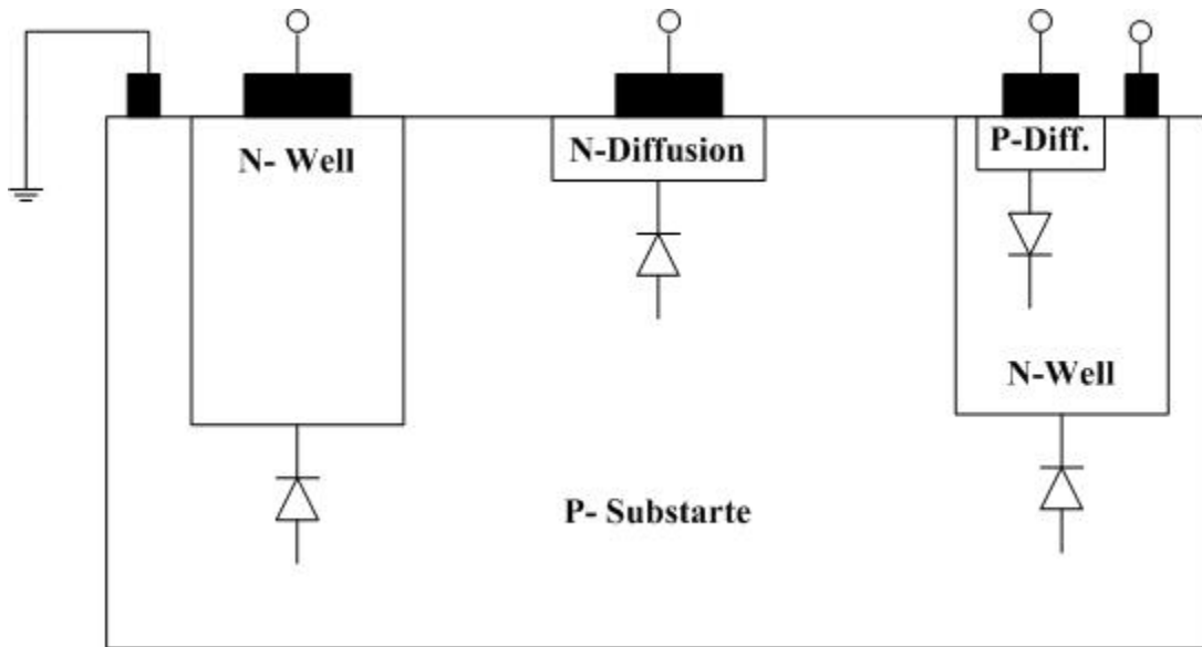
Figure 1.4 Available CMOS photodetectors [Bolton]
