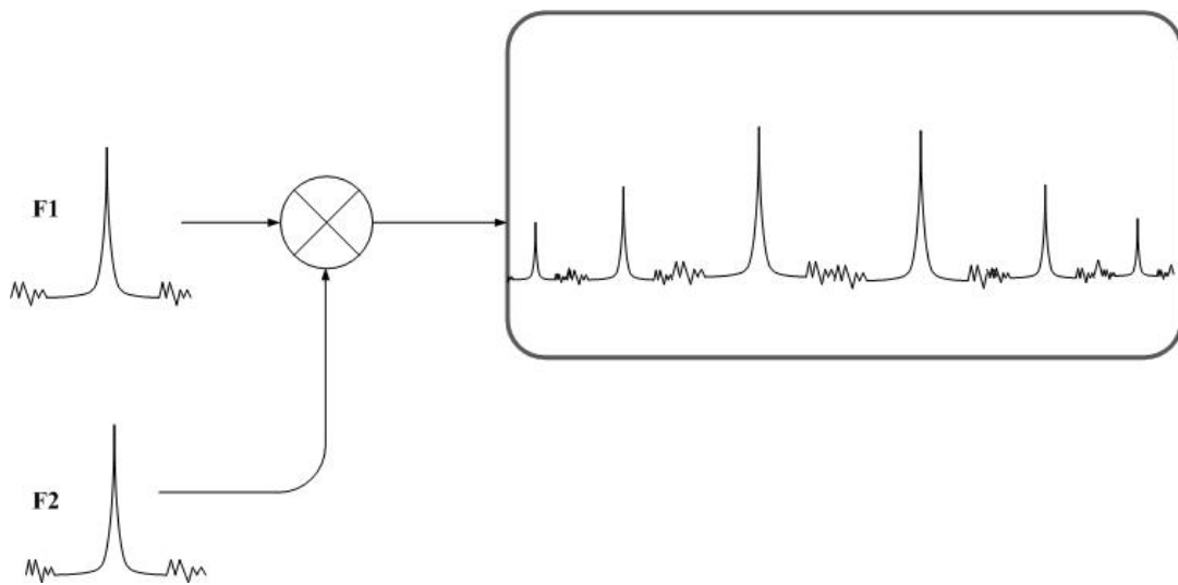
Figure 3.9 Spectrum of mixer output [Carr]
