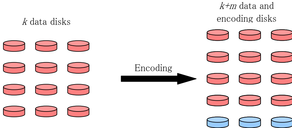
Figure 1: Encoding using an erasure code.
