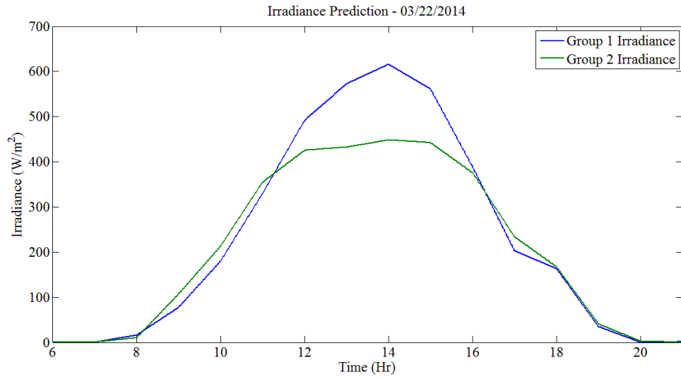
Figure 4.7: Irradiance prediction
