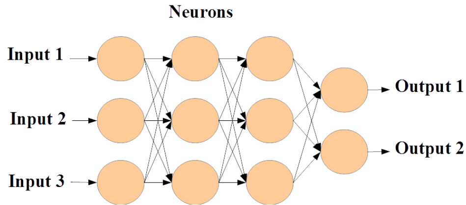
Figure 2.12: Neural networks
