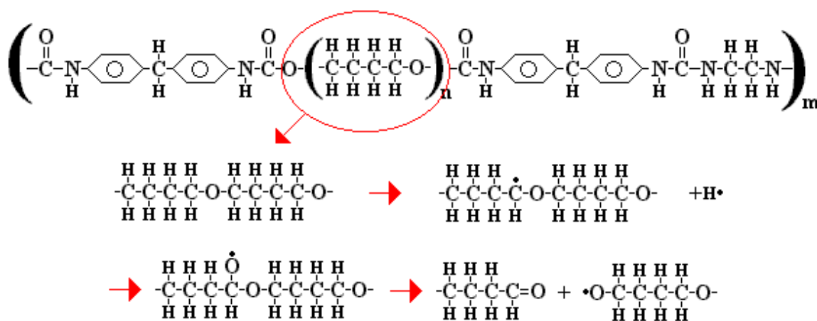
Figure 4.5.1.2. Suggested degradation mechanism for PTMG based polymers.
