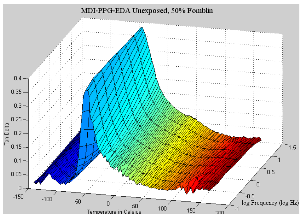
Figure C.24. PPG based PU, 50% fluorinated, unexposed, \text{Tan}\delta versus temperature.
