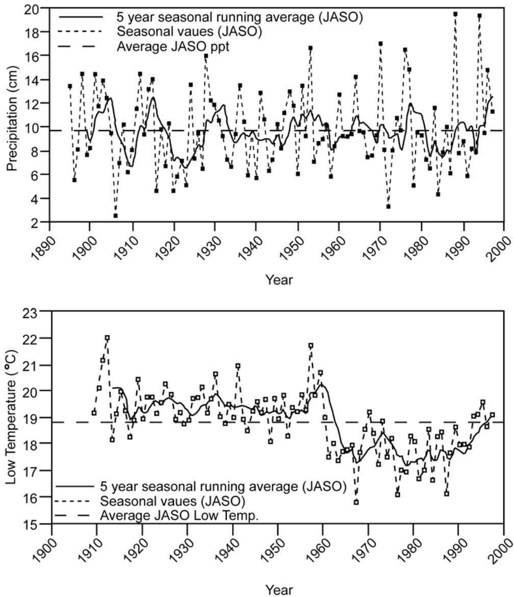
Figure 12. Local yearly averaged precipitation and low temperature values for the latewood growing season.
