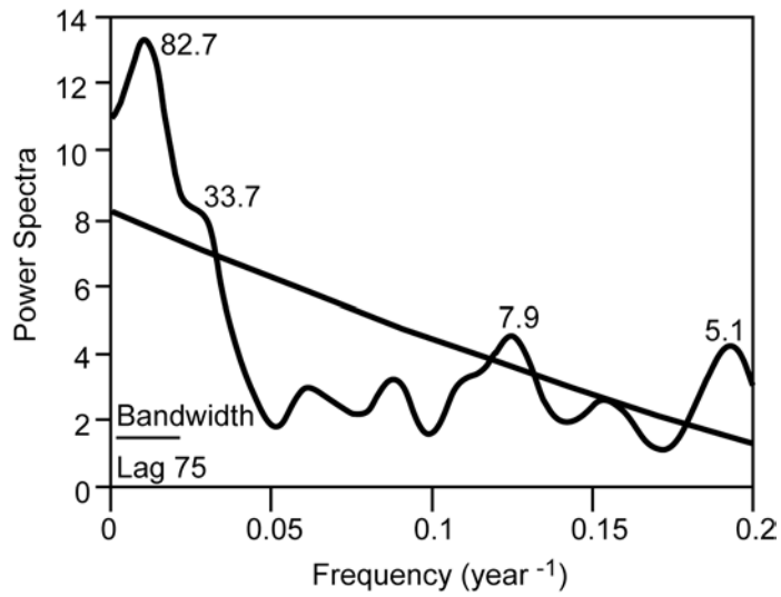
Figure 13. Spectral analysis of LW oxygen isotopes from 1770–1997. Significant periodicities occur at \sim 82.7 , 33.7, 7.9, and 5.1 years.
