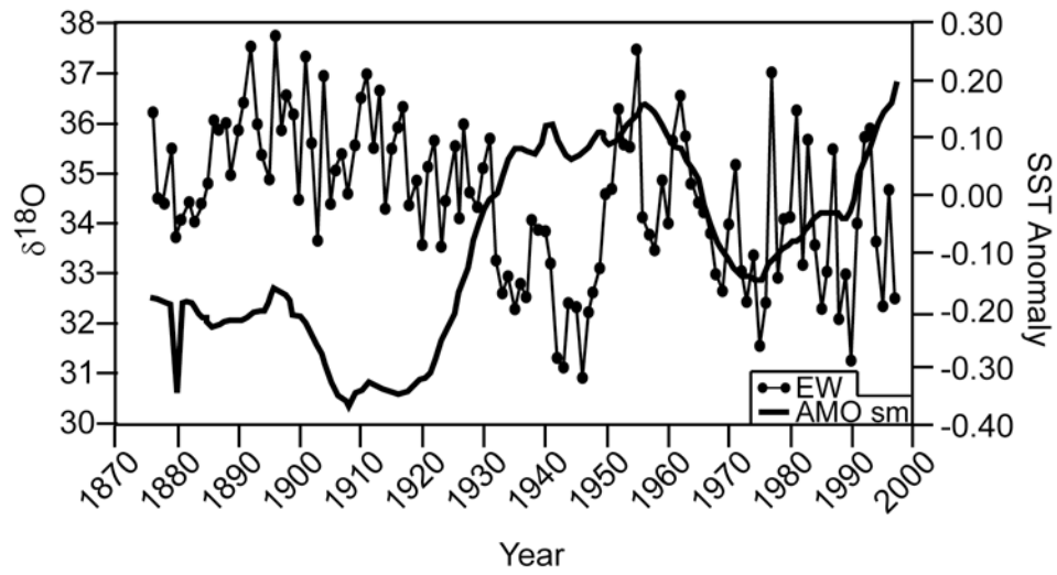
Figure 8. Tree-ring \delta^{18}\text{O} (vs. V-SMOW) EW values compared with SST anomalies in the North Atlantic (AMO indices smoothed with a 10 year running average). A strong negative correlation is consistent until \sim 1950 .
