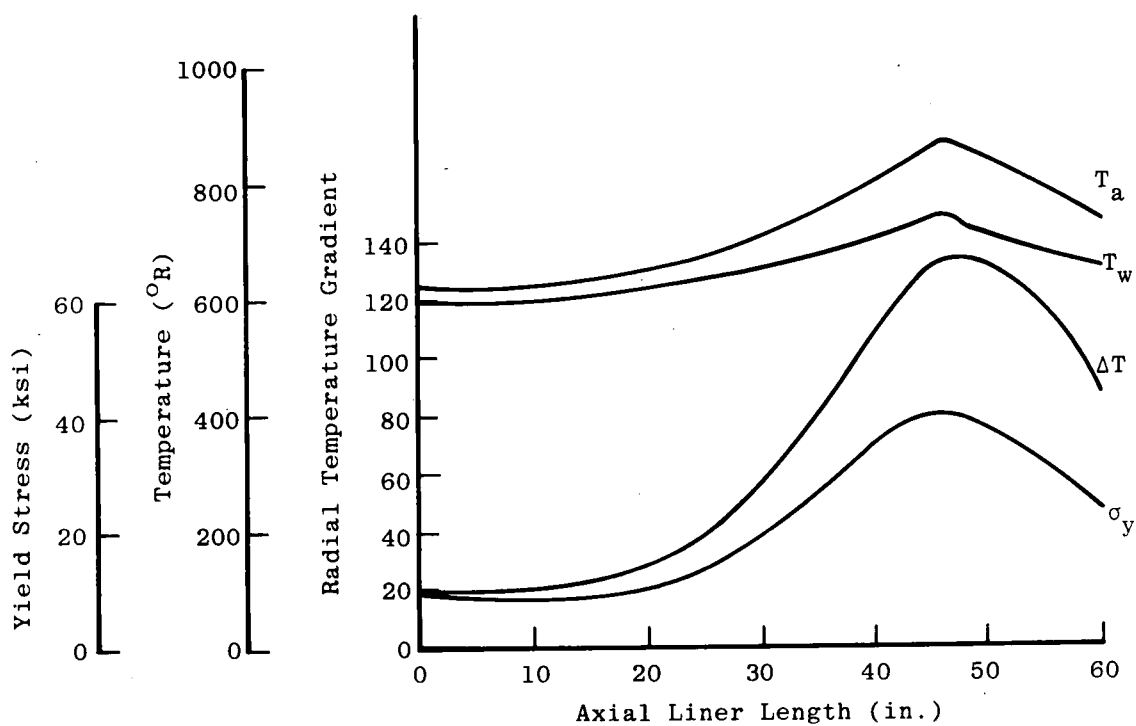
Figure 4. Example problem results.
