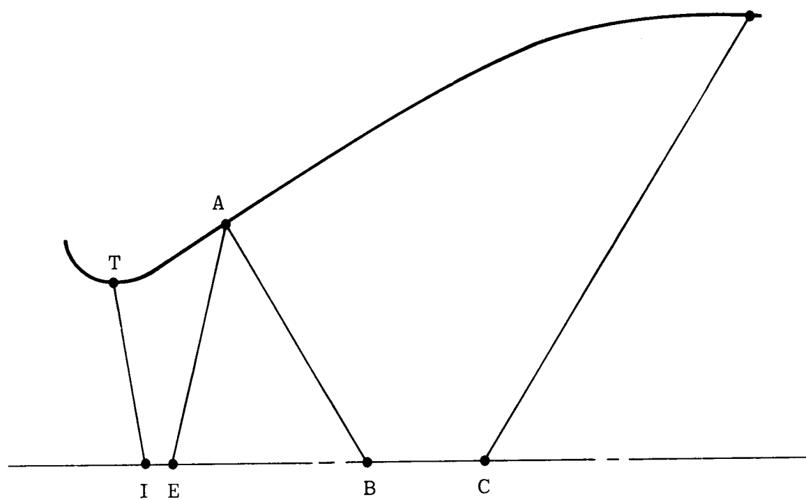
Figure 3. Characteristic diagram for inviscid supersonic contour.
