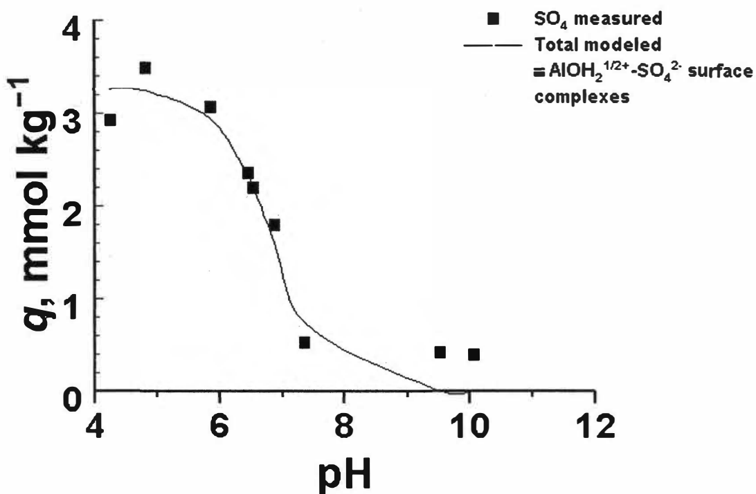
Figure 26. The predicted and experimentally-determined adsorption of sulfate ( \text{SO}_4 ) by gibbsite in 0.01 M NaCl. The closed squares represent the experimental data; the solid line represent the predicted formation of \equiv\text{AlOH}_2^{1/2+}\text{-SO}_4^{2-} . Error bars represent the standard error (Eq. [22]) of q . Where error bars cannot be seen, they are within the range of the marker.
