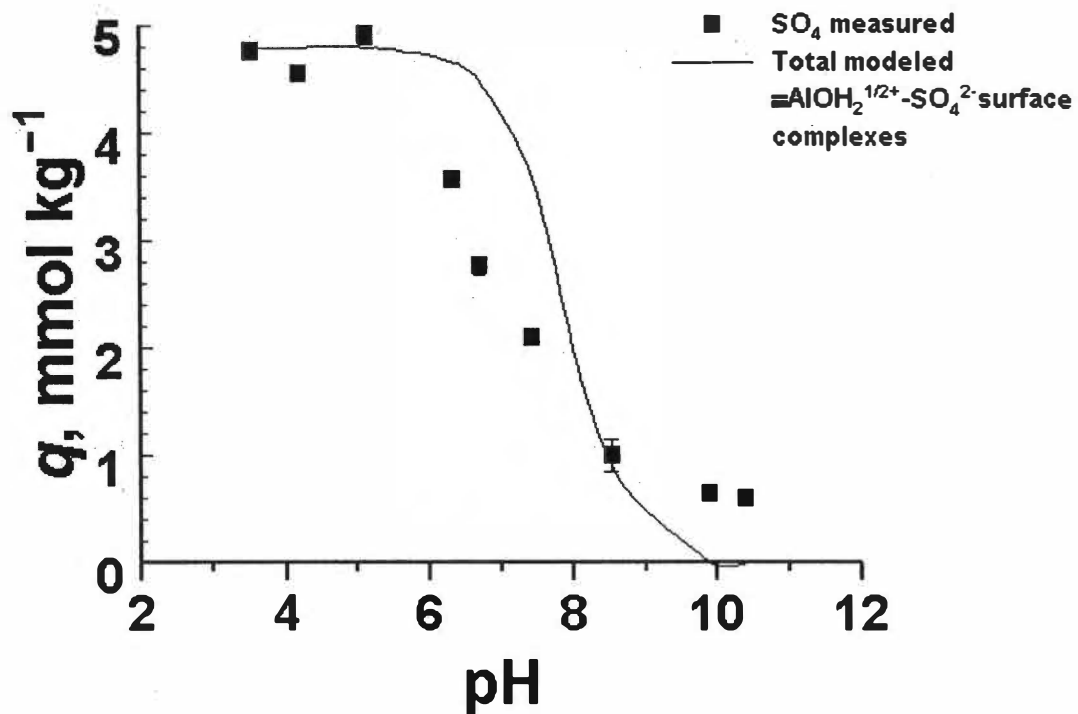
Figure 25. The predicted and experimentally-determined adsorption of sulfate ( \text{SO}_4 ) by gibbsite in 0.001 M NaCl. The closed squares represent the experimental data; the solid line represent the predicted formation of \equiv\text{AlOH}_2^{1/2+}\text{-SO}_4^{2-} . Error bars represent the standard error (Eq. [22]) of q . Where error bars cannot be seen, they are within the range of the marker.
