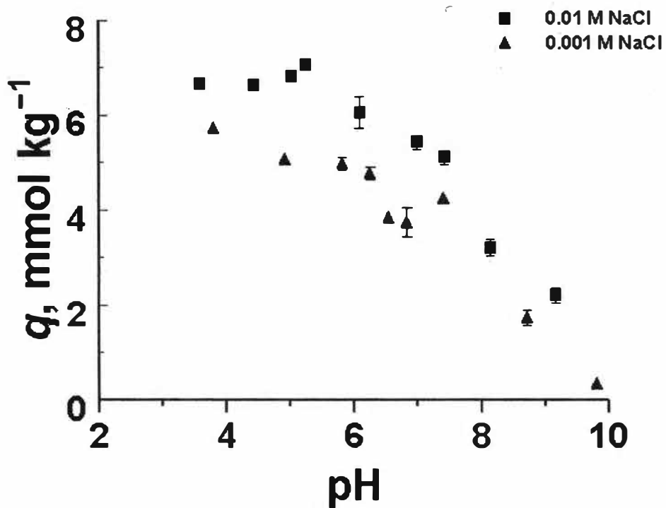
Figure 32. The adsorption edge of phosphate ( \text{PO}_4 ) on kaolinite in 0.01 and 0.001 M NaCl. Error bars represent the standard error (Eq. [22]) of q . Where error bars cannot be seen, they are within the range of the marker.
