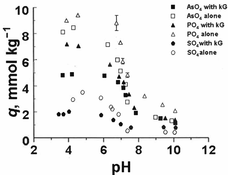
Figure 13. The effect of ketogluconate (kG) on the adsorption of AsO 4 , PO 4 , and SO 4 to gibbsite in 0.01 M NaCl. Error bars represent the standard error (Eq. [22]) of q . Where error bars cannot be seen, they are within the range of the marker.
