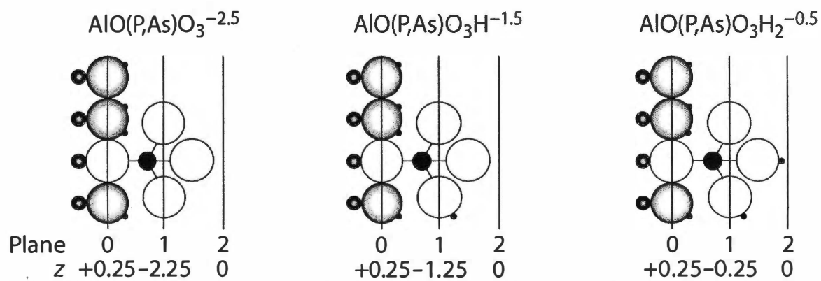
Figure 21. Phosphate, arsenate, and sulfate modeled surface complexes and charge
