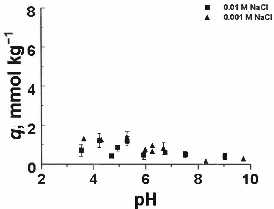
Figure 34. The adsorption edge of sulfate ( \text{SO}_4 ) on kaolinite in 0.01 and 0.001 M NaCl. Error bars represent the standard error (Eq. [22]) of q . Where error bars cannot be seen, they are within the range of the marker.
