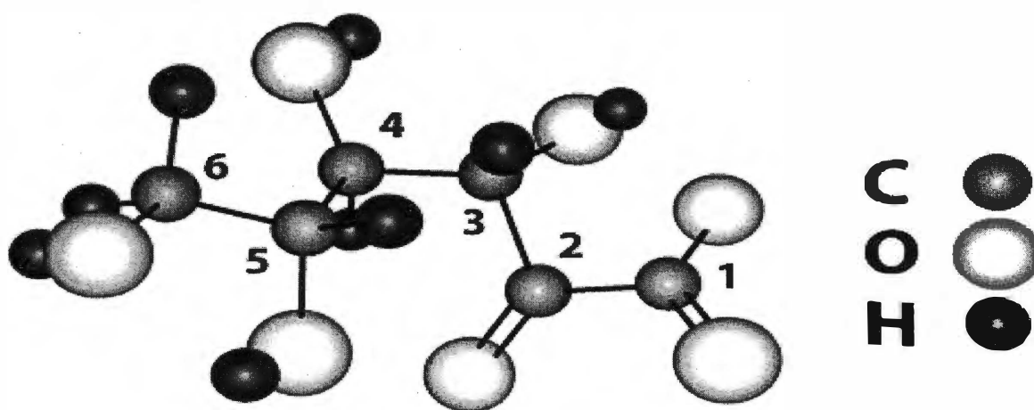
Figure 1. Molecular structure of 2-keto-D-gluconate with numbered carbon atoms.
