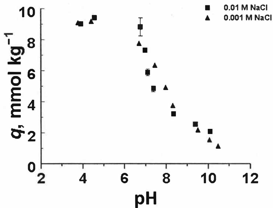
Figure 8. The adsorption edge of phosphate ( \text{PO}_4 ) on gibbsite in 0.01 and 0.001 M NaCl. Error bars represent the standard error (Eq. [22]) of q . Where error bars cannot be seen, they are within the range of the marker.
