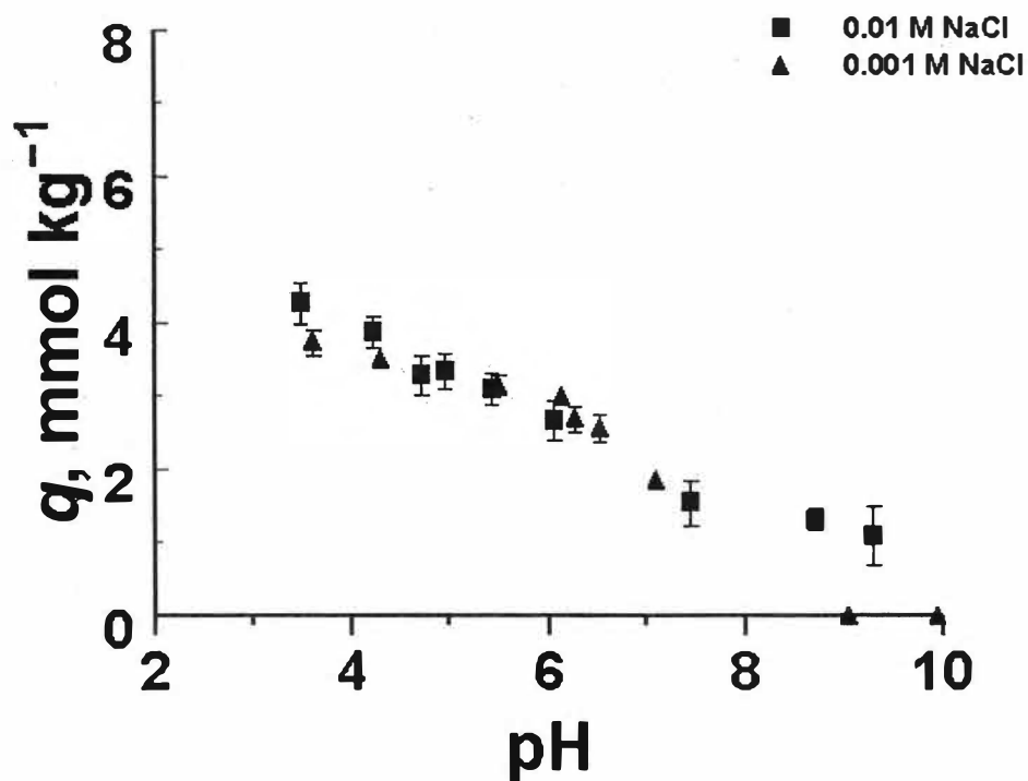
Figure 31. The adsorption edge of 2-ketogluconate (kG) on kaolinite in 0.01 and 0.001 M NaCl. Error bars represent the standard error (Eq. [22]) of q . Where error bars cannot be seen, they are within the range of the marker.
