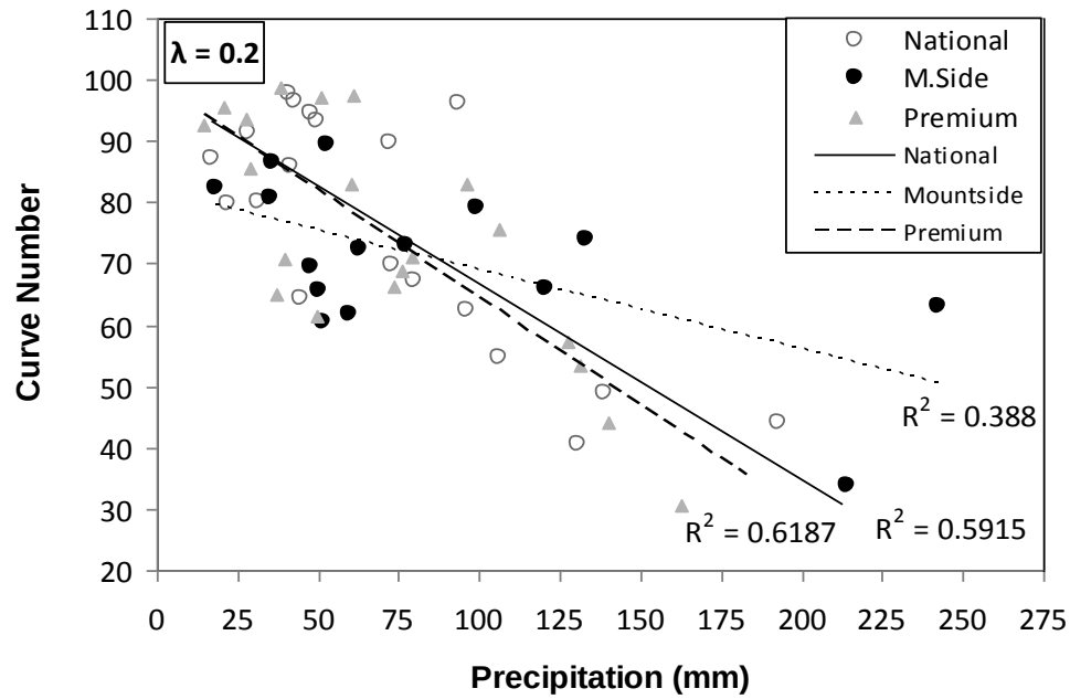
Figure 7. Curve numbers for each of the three sites in relation to precipitation amounts for \lambda = 0.2 .
