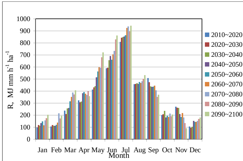
Figure 36. Rainfall erosivity ( \text{MJ} \cdot \text{mm} \cdot \text{h}^{-1} \cdot \text{ha}^{-1} ) distribution for B1 greenhouse gas emission scenario during projection period (2010~2099) and for different months.
