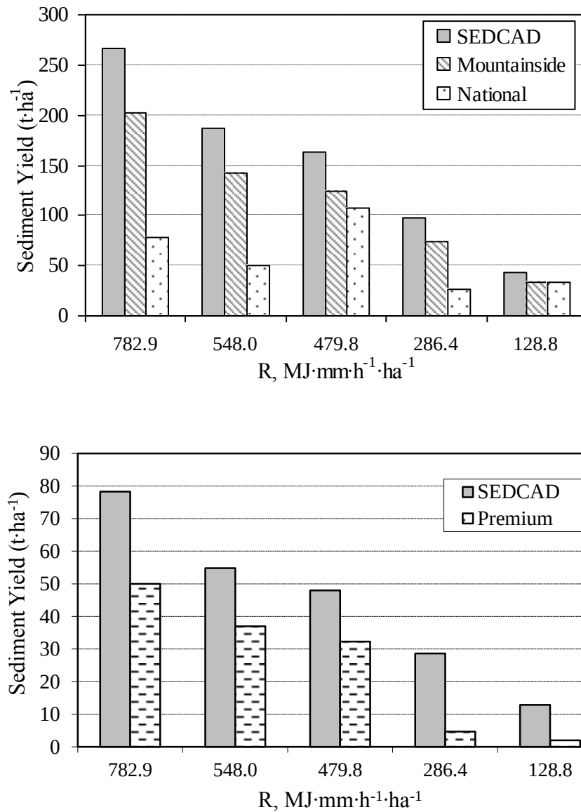
Figure 26. Sediment yields in \text{t}\cdot\text{ha}^{-1} from measured amounts at National, Premium, and Mountainside study sites, and SEDCAD calculated amounts, grouped by erosivity (R) classes: 782.9, 548.0, 479.8, 286.4, and 128.8 \text{MJ}\cdot\text{mm}\cdot\text{h}^{-1}\cdot\text{ha}^{-1} .
