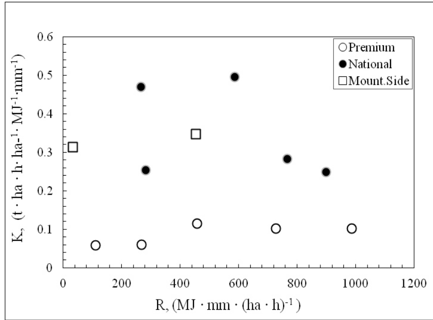
Figure 22. Erodibility (K-factors) ( \text{t} \cdot \text{ha} \cdot \text{h} \cdot \text{ha}^{-1} \cdot \text{MJ}^{-1} \cdot \text{mm}^{-1} ) related to each sampling event, for Premium, National, and Mountainside study sites from June to August 2009.
