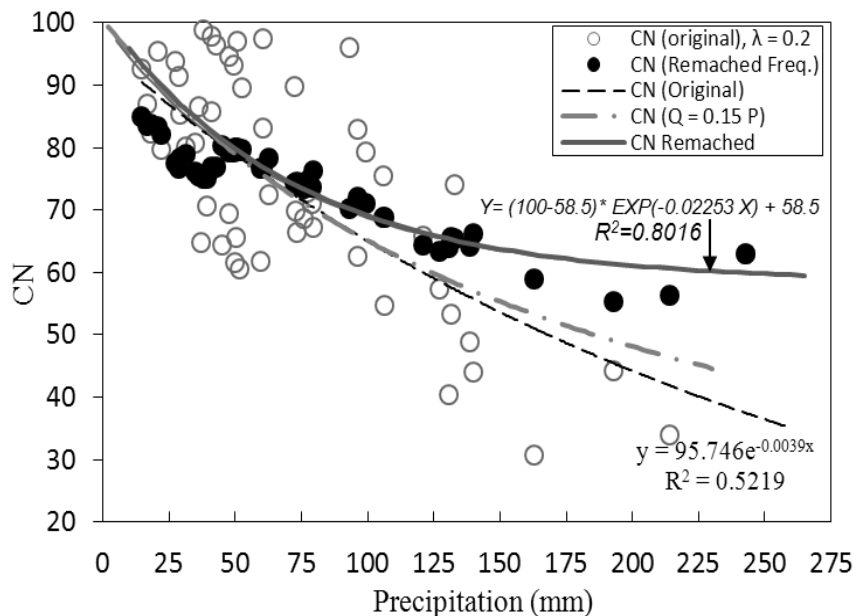
Figure 12. Best fit exponential curve for P-Q matched frequency pairs and \lambda = 0.2 .
