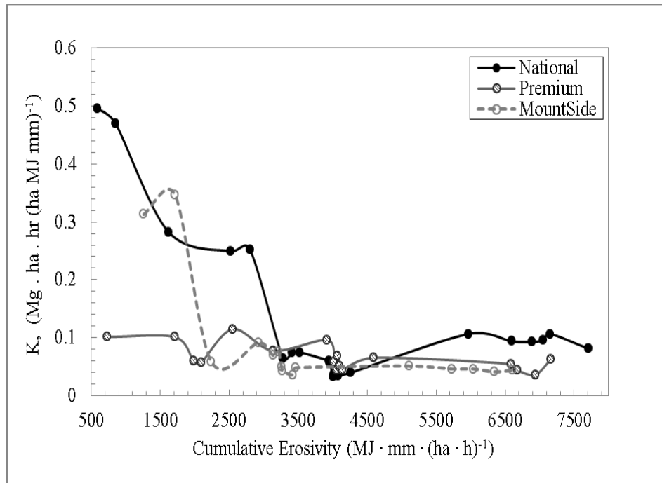
Figure 24. Erodibility (K-factors) ( \text{t} \cdot \text{ha} \cdot \text{h} \cdot \text{ha}^{-1} \cdot \text{MJ}^{-1} \cdot \text{mm}^{-1} ) related to each sampling event versus cumulative erosivity (R-factor) ( \text{MJ} \cdot \text{mm} \cdot (\text{ha} \cdot \text{h})^{-1} ) over the 14-month monitoring period from June 2009 through July 2010 for Premium, National, and Mountainside study sites.
