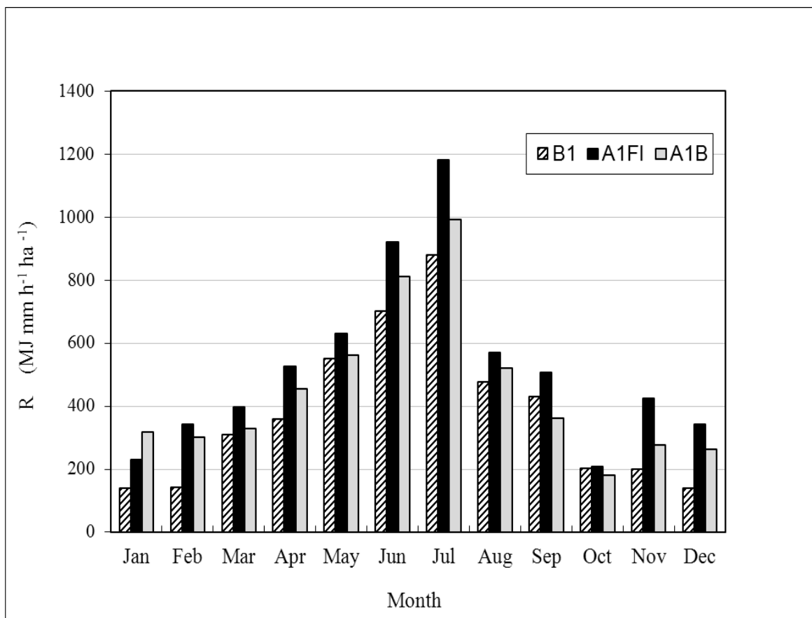
Figure 34. Rainfall erosivity for period 2010 – 2099 (New River Basin, TN).
