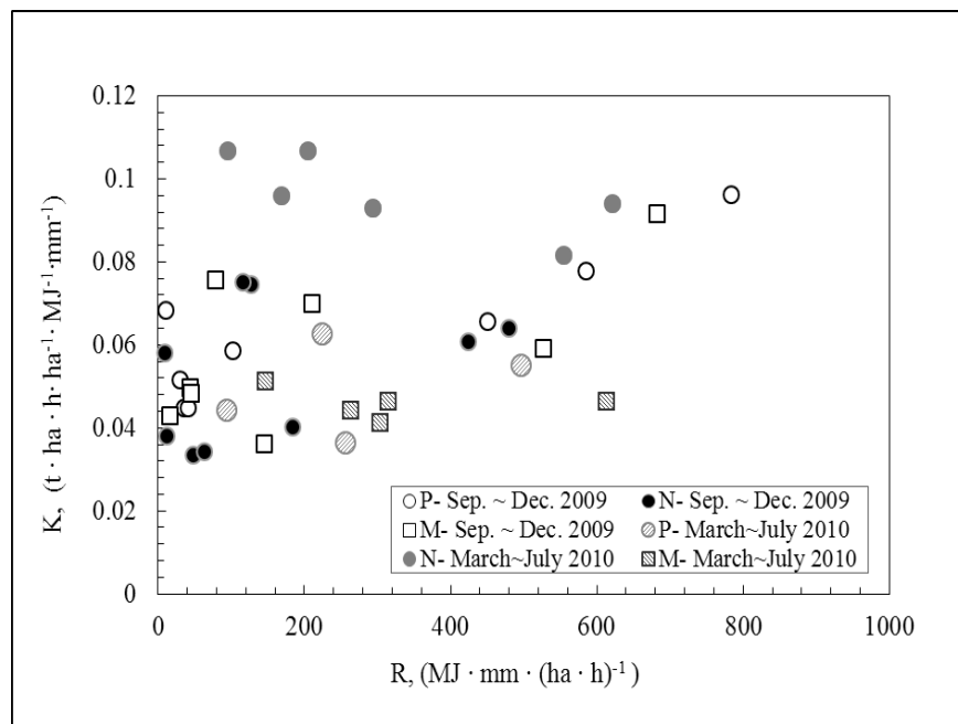
Figure 23. Erodibility (K-factors) ( \text{t} \cdot \text{ha} \cdot \text{h} \cdot \text{ha}^{-1} \cdot \text{MJ}^{-1} \cdot \text{mm}^{-1} ) related to each sampling event, for each study site (N = National, P = Premium, and M = Mountainside) from September 2009 to July 2010.
