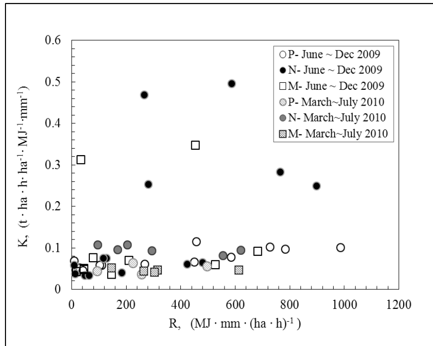
Figure 21. Erodibility (K factors) ( \text{t} \cdot \text{ha} \cdot \text{h} \cdot \text{ha}^{-1} \cdot \text{MJ}^{-1} \cdot \text{mm}^{-1} ) related to each sampling event, for each study site (N = National, P = Premium, and M = Mountainside) for the entire monitoring period from June 2009 to July 2010.
