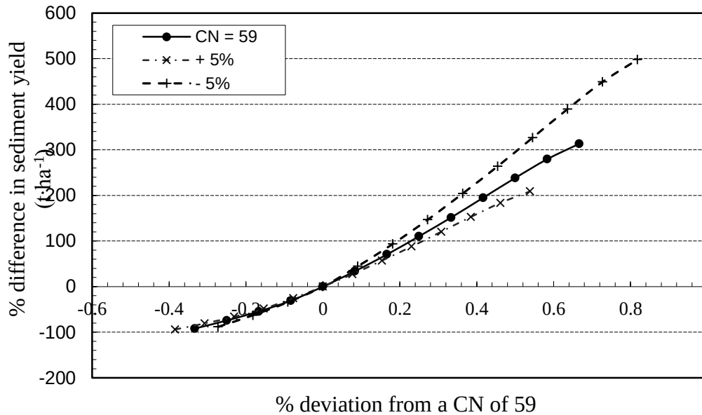
Figure 27. Percent difference in amount of estimated sediment yields ( \text{t}\cdot\text{ha}^{-1} ) relative to a percent deviation in CN selection from the measured estimate of 59 for loose compaction spoils on reclaimed surface coal mining sites.
