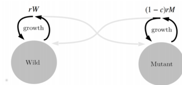
(a) simple-model
