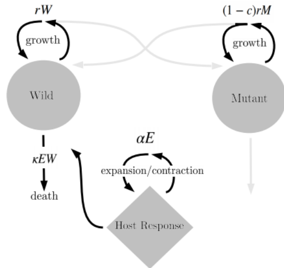
(b) immune-model
