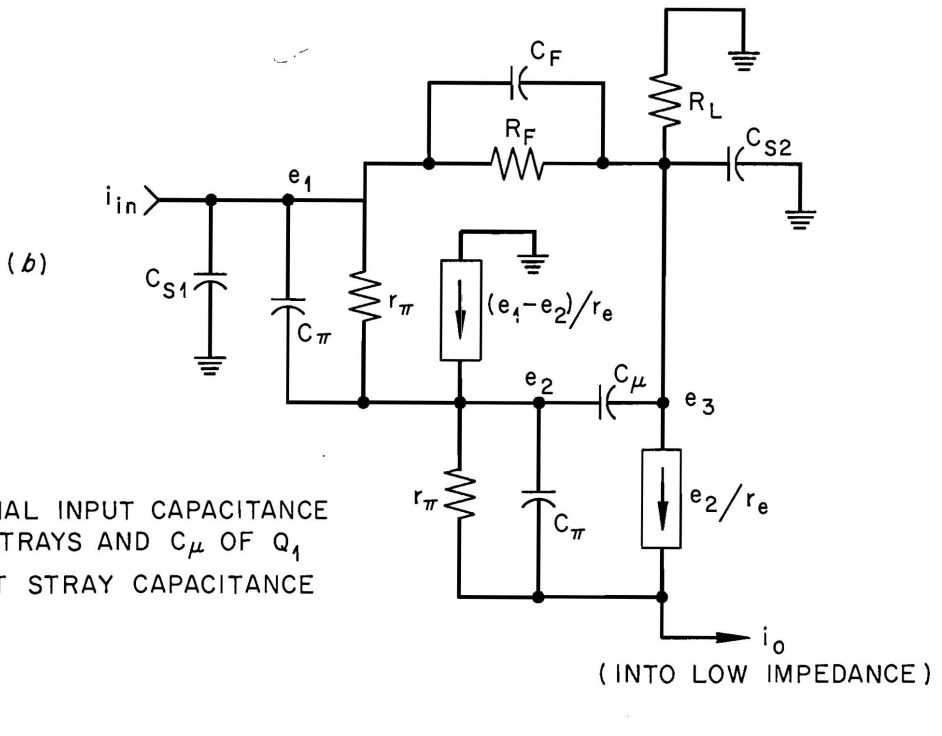
Figure 19. (a) Circuit diagram of a high-frequency, two-transistor, shunt-feedback stage with (b) the corresponding equivalent circuit.
