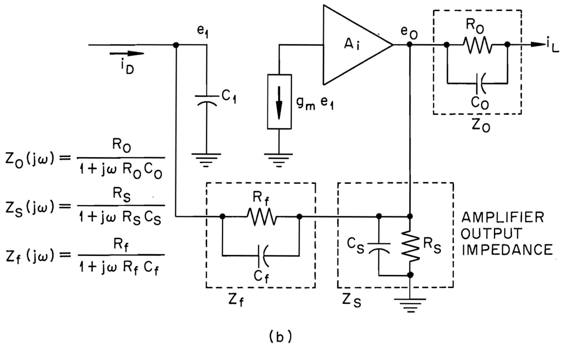
Figure 11. (a) Modification of the preamplifier stage of Fig. 10, page 37, with (b) the equivalent circuit.
