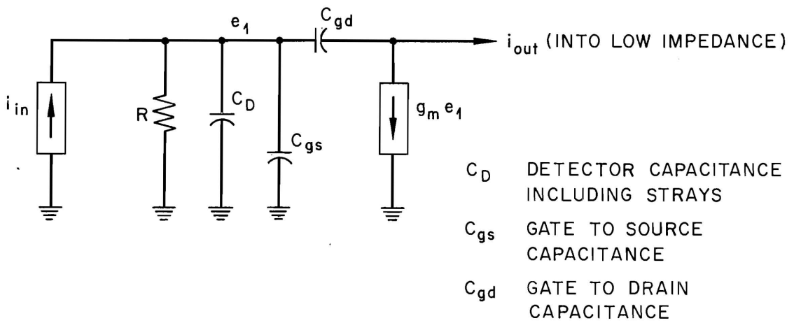
Figure 17. Equivalent circuit of the input FET.
