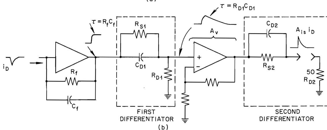
Figure 9. Illustration of a differentiation technique for recovering the detector-current waveform from a charge-sensitive preamplifier.
