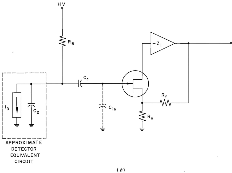
Figure 1. General configurations of (a) the charge-sensitive and (b) the voltage-sensitive preamplifiers.
