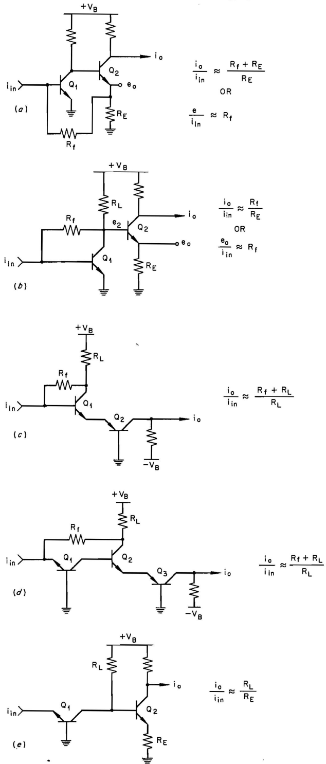
Figure 2. Current amplifying stages with approximate current gains indicated.
