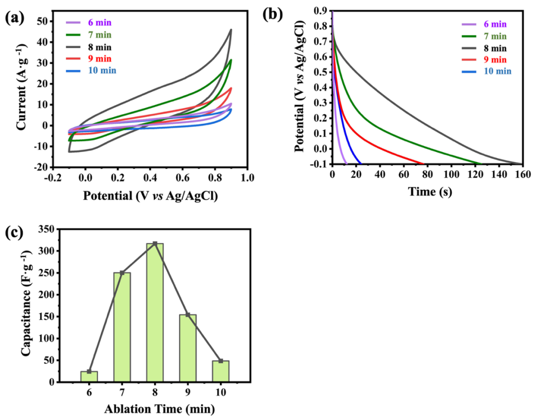
Figure 5.4. (a) CV curves for the \text{Mn}_3\text{O}_4 -rGO HNCs composites in 0.5 M \text{Na}_2\text{SO}_4 (b) discharge curves at 2 A/g and (c) calculated capacitance
