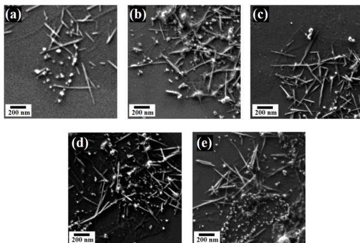
Figure 5.2. SEM images of \text{Mn}_3\text{O}_4 -rGO hybrid nanocomposites prepared under (a) 6 min (b) 7 min (c) 8 min (d) 9 min and (e) 10 min ablation time
