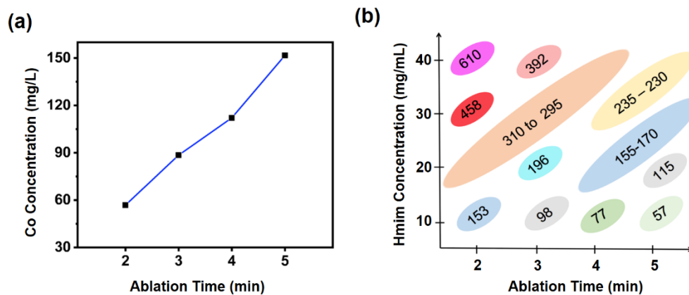
Figure 2.4. (a) ICP-OES Co concentration as a function of ablation time (b) Stochiometric ratio of Hmim to Cobalt for the various experimental conditions used
