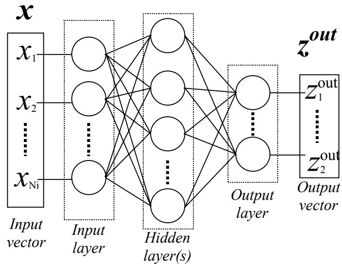
Figure 4: Fully Connected Artificial Neural Network.
