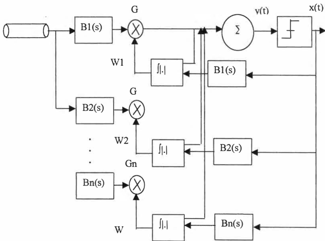
Figure 2.1: General Equalizer block diagram
