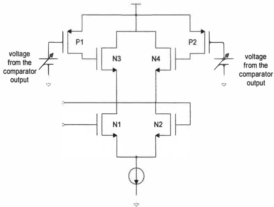
Figure 3.13: Variable resistance implementation by triode connected PMOS
