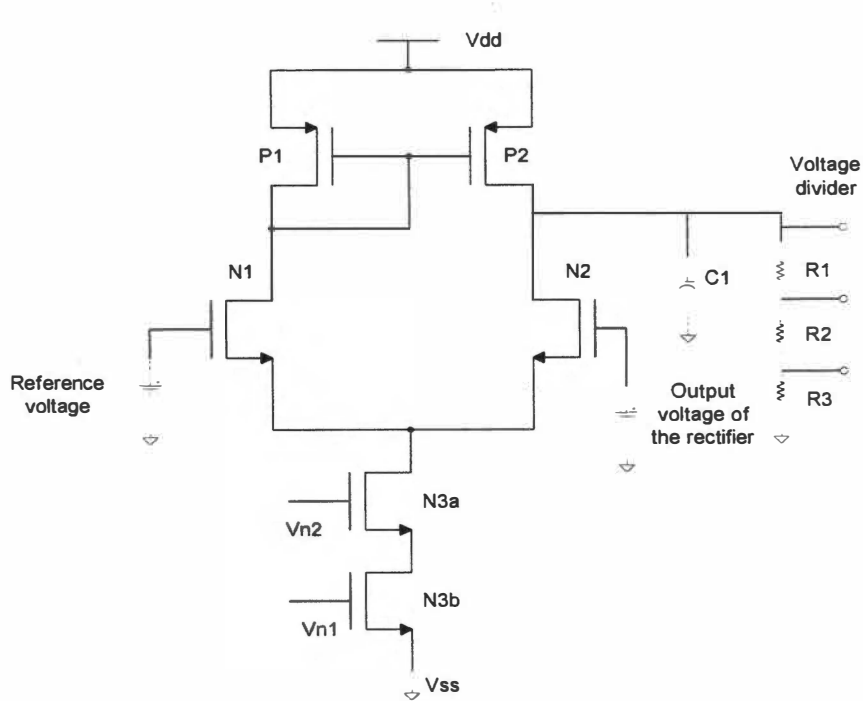
Figure 3.8: Comparator circuit with three- resistor voltage divider
