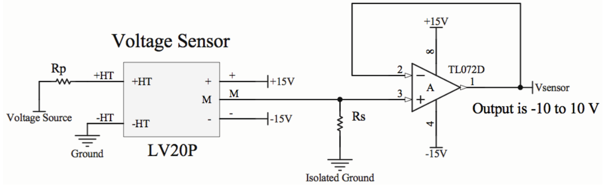
Figure 5.5: Voltage sensor circuit.
