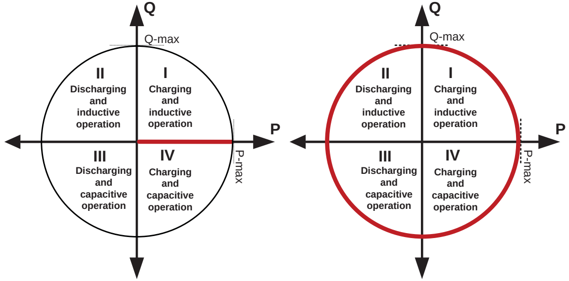
(a) Power factor-corrected unidirectional charger operation (b) Four-quadrant bidirectional charger operation
