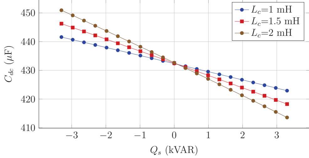
Figure 3.8: Change of C_{dc} with varying Q_s and for different L_c values for the case of S = 3.3 kVA.
