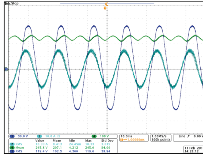
Figure 5.15: Charging and capacitive reactive power operation of the ac-dc converter for \text{pf}=0.91 leading.
