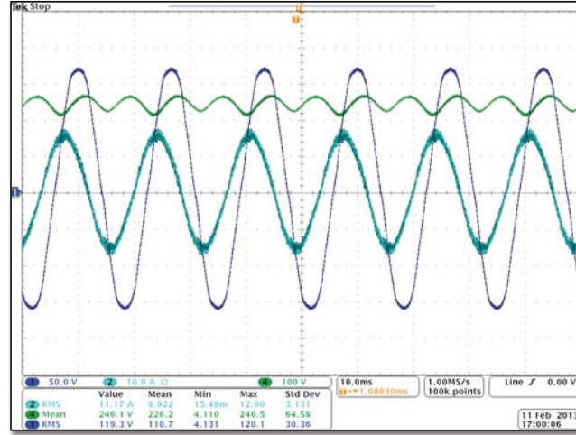
Figure 5.16: Charging and capacitive reactive power operation of the ac-dc converter for pf=0.67 leading.
