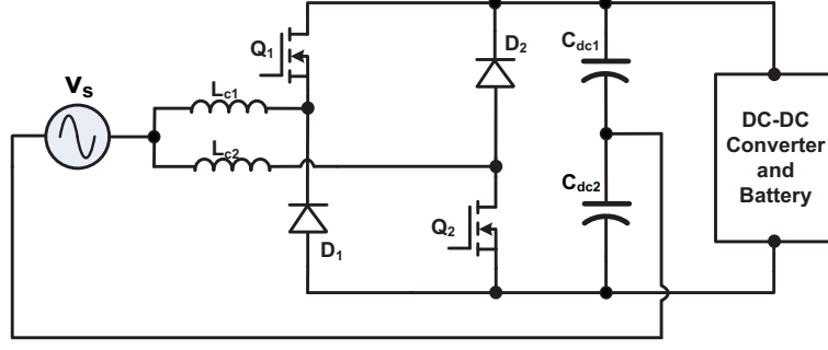
Figure 2.7: Dual-buck ac-dc half-bridge converter.
