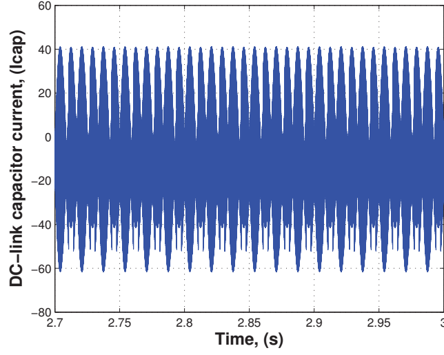
Figure 4.21: DC-link capacitor current for Level 2 6.6 kVA P_s = 1.0 charging only operation ( L_c=1.5 mH).
