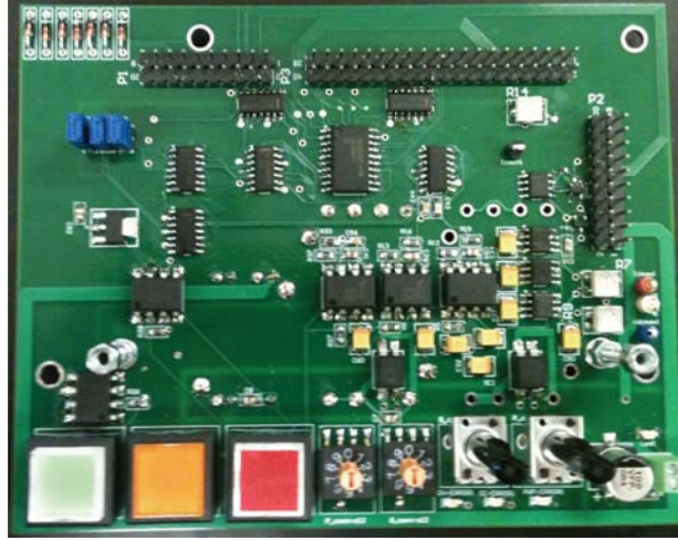
Figure 5.6: DSP interface board circuit revision 1.
