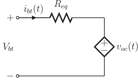
Figure 4.4: Equivalent model of the battery pack.
