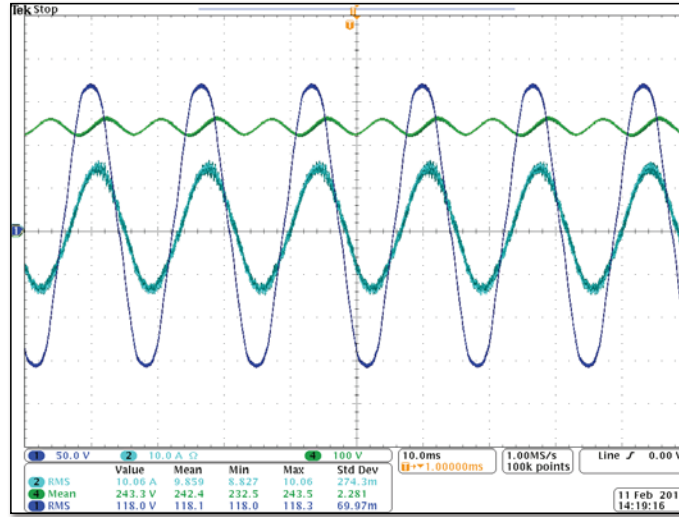
Figure 5.17: Charging and capacitive reactive power operation of the ac-dc converter for pf=0.91 lagging.
