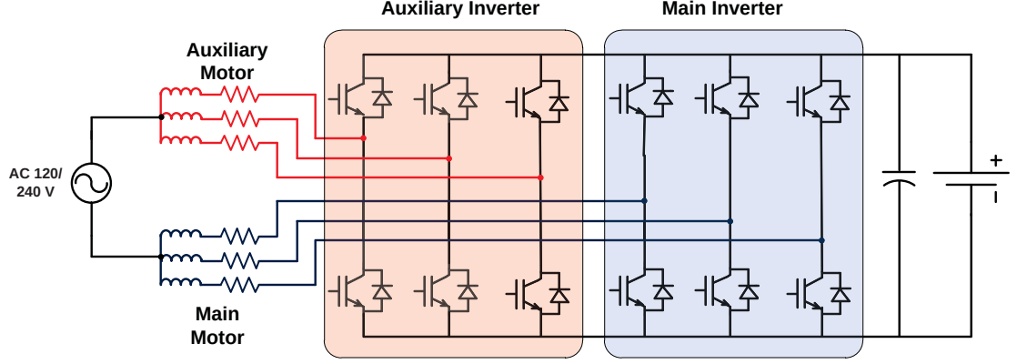
Figure 2.13: An integrated charger employing two inverters [12].
