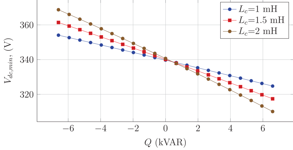
Figure 3.15: Change of the required minimum dc link voltage for different reactive power values for S = 6.6 kVA.
