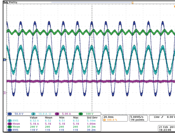
Figure 5.14: Charging only operation of the total system.
