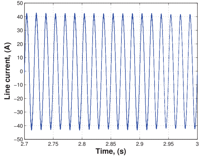
Figure 4.19: Line current for Level 2 6.6 kVA P_s = 1.0 charging only operation ( L_c=1.5 mH).
