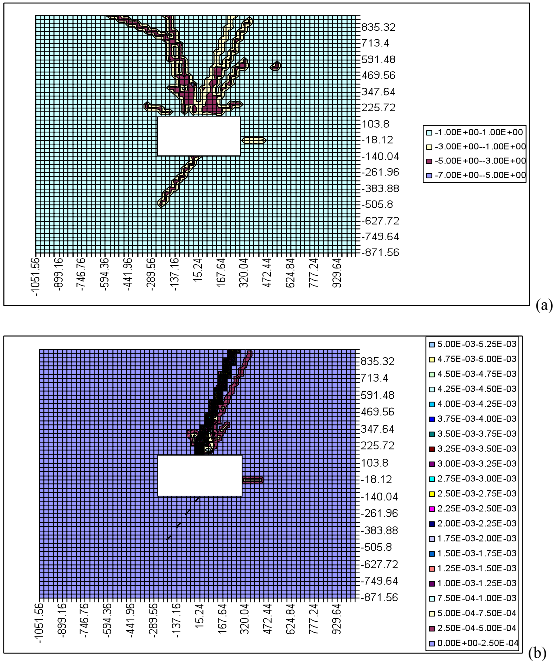
Figure 5.1.15: Dose Rate Outside of Conex. White Box represents the Conex boundaries.
