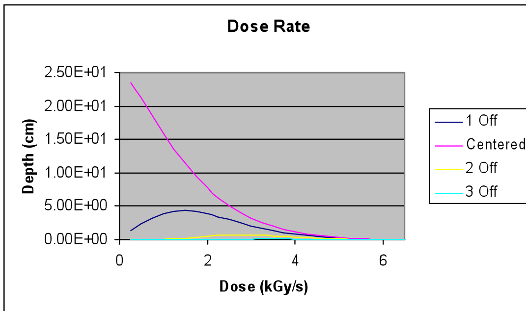
Figure 5.2.2: Dose rates as a function of depth for varying widow distances from the beam. The Curves represent the beam location with relation the volume where the dose rate is being tallies (i.e. 1 off means the beam window is 1 beam window distance away – 1.05cm).
