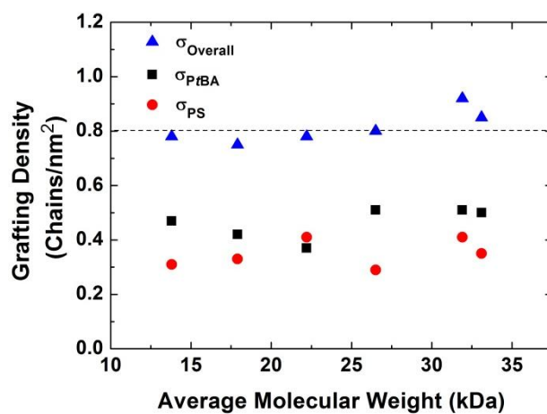
Figure 3.2 Plots of individual grafting density of PtBA ( \sigma_{\text{PtBA}} , black square), individual grafting density of PS ( \sigma_{\text{PS}} , red circle), and overall grafting density of mixed PtBA/PS brushes ( \sigma_{\text{overall}} , blue triangle) versus average molecular weight of the two polymers.
