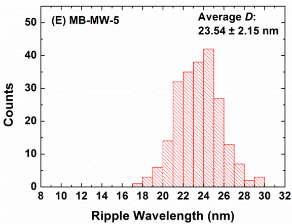
Figure 3.4 Distributions of ripple wavelengths of features (sum of both widths of neighboring PtBA and PS nanostripes) obtained from TEM image analysis of (A) Figure 3.3A, MB-MW-1, (B) Figure 3.3B, MB-MW-2, (C) Figure 3.3C, MB-MW-3, (D) Figure 3.3D, MB-MW-4, (E) Figure 3.3E, MB-MW-5, and (F) Figure 3.3F, MB-MW-6.
