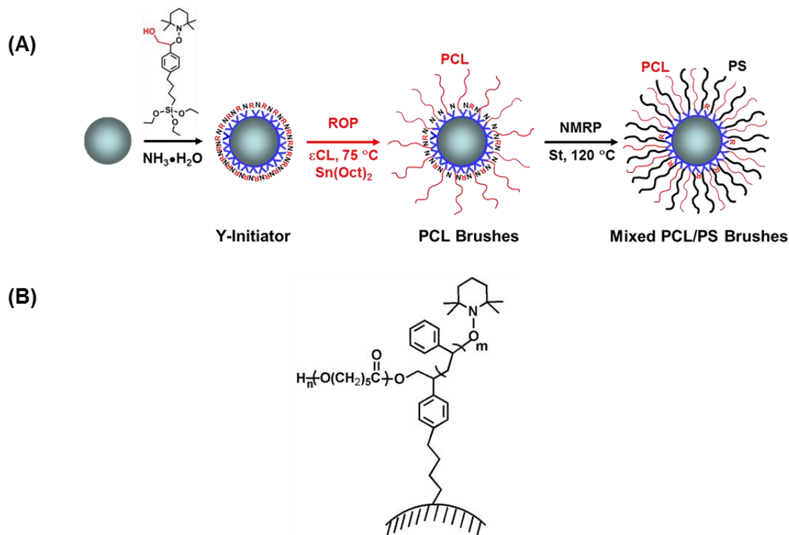
Scheme 4.1 (A) Synthesis of mixed poly( \epsilon -caprolactone) (PCL)/polystyrene (PS) brushes on silica particles functionalized with a Y-initiator bearing a hydroxyl group and a TEMPO moiety by combining \text{Sn}(\text{Oct})_2 -catalyzed ring-opening polymerization (ROP) of \epsilon -caprolactone ( \epsilon\text{CL} ) and nitroxide-mediated radical polymerization (NMRP) of styrene (B) Schematic illustration of mixed PCL/PS brushes on silica particles
