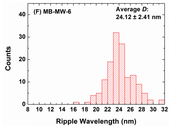
Figure 3.4 Distributions of ripple wavelengths of features (sum of both widths of neighboring PtBA and PS nanostripes) obtained from TEM image analysis of (A) Figure 3.3A, MB-MW-1, (B) Figure 3.3B, MB-MW-2, (C) Figure 3.3C, MB-MW-3, (D) Figure 3.3D, MB-MW-4, (E) Figure 3.3E, MB-MW-5, and (F) Figure 3.3F, MB-MW-6.
