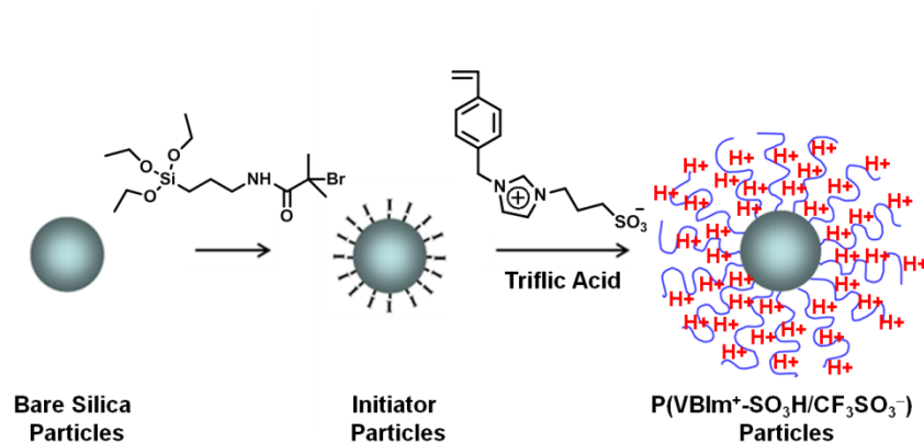
Scheme 5.3 Synthesis of P(VBIm + -SO 3 H/CF 3 SO 3 - ) brush-grafted silica particles from 2-bromo-2-methyl- N -(3-(triethoxysilyl)propyl)propanamide-functionalized silica particles by surface-initiated atom transfer radical polymerization and subsequent acidification with triflic acid
