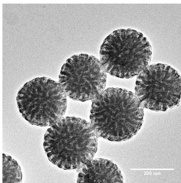
Figure B11. Top-view, bright field TEM micrograph of MB-MW-5 (PtBA M_n = 32.1 kDa, \sigma_{\text{PtBA}} = 0.51 chains/nm 2 ; PS M_n = 31.6 kDa, \sigma_{\text{PS}} = 0.41 chains/nm 2 ; \sigma_{\text{overall}} = 0.92 chains/nm 2 ) after being cast from a surfactant-stabilized aqueous dispersion. The sample was stained with RuO 4 vapor at room temperature for 20 min.
