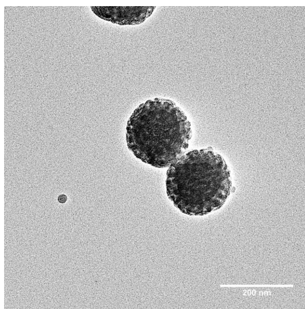
Figure B8. Top-view, bright field TEM micrograph of MB-MW-2 (PtBA M_n = 18.3 kDa, \sigma_{\text{PtBA}} = 0.42 chains/nm 2 ; PS M_n = 17.5 kDa, \sigma_{\text{PS}} = 0.33 chains/nm 2 ; \sigma_{\text{overall}} = 0.75 chains/nm 2 ) after being cast from a surfactant-stabilized aqueous dispersion. The sample was stained with RuO 4 vapor at room temperature for 20 min.
