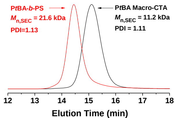
Figure B14. Size exclusion chromatography (SEC) analysis of macro-CTA poly( tert -butyl acrylate) (PtBA) and diblock copolymer poly( tert -butyl acrylate)- b -polystyrene (PtBA- b -PS, DB-1). PtBA macro-CTA was synthesized by RAFT polymerization; [ t BA]:[CTA]:[AIBN] = 536:1.0:0.10, anisole, 70 °C. PtBA- b -PS was synthesized using PtBA as macro-CTA in anisole at 70 °C. SEC analysis was conducted using THF as eluent solvent with a flow rate at 1 mL/min.
