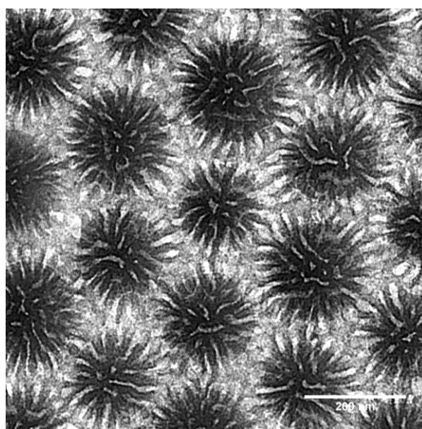
Figure B5. Top-view, bright field TEM micrograph of MB-MW-5 (PtBA M_n = 32.1 kDa, \sigma_{\text{PtBA}} = 0.51 chains/nm 2 ; PS M_n = 31.6 kDa, \sigma_{\text{PS}} = 0.41 chains/nm 2 ; \sigma_{\text{overall}} = 0.92 chains/nm 2 ) after being cast from a CHCl 3 dispersion and annealed with CHCl 3 vapor. The sample was stained with RuO 4 vapor at room temperature for 20 min.
