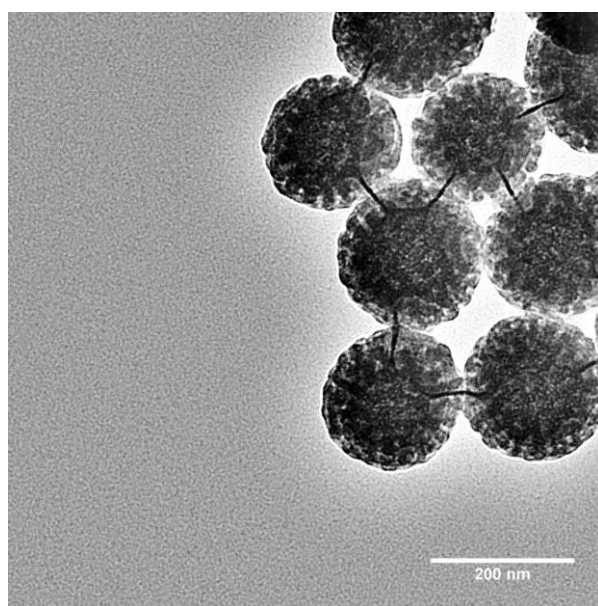
Figure B9. Top-view, bright field TEM micrograph of MB-MW-3 (PtBA M_n = 22.0 kDa, \sigma_{\text{PtBA}} = 0.37 chains/nm 2 ; PS M_n = 22.3 kDa, \sigma_{\text{PS}} = 0.41 chains/nm 2 ; \sigma_{\text{overall}} = 0.78 chains/nm 2 ) after being cast from a surfactant-stabilized aqueous dispersion. The sample was stained with RuO 4 vapor at room temperature for 20 min.
