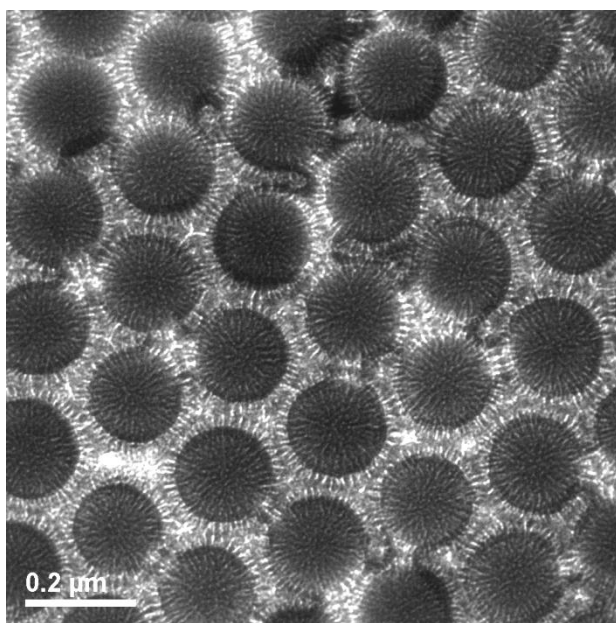
Figure A1. A top-view bright field TEM micrograph of MB-1 (PtBA M_n = 18.6 kDa, \sigma_{\text{PtBA}} = 0.63 chains/nm 2 ; PS M_n = 19.4 kDa, \sigma_{\text{PS}} = 0.43 chains/nm 2 ; \sigma_{\text{overall}} = 1.06 chains/nm 2 ) after being cast from a CHCl 3 dispersion, annealed with CHCl 3 vapor for at least 3 h, and stained with RuO 4 vapor at room temperature for 20 min. CHCl 3 is a good solvent for both PtBA and PS.
