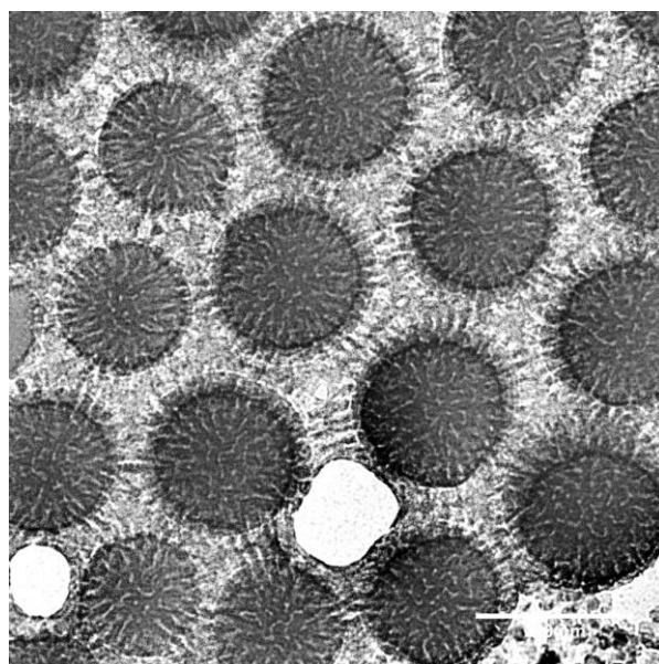
Figure B2. Top-view, bright field TEM micrograph of MB-MW-2 (PtBA M_n = 18.3 kDa, \sigma_{\text{PtBA}} = 0.42 chains/nm 2 ; PS M_n = 17.5 kDa, \sigma_{\text{PS}} = 0.33 chains/nm 2 ; \sigma_{\text{overall}} = 0.75 chains/nm 2 ) after being cast from a CHCl 3 dispersion and annealed with CHCl 3 vapor. The sample was stained with RuO 4 vapor at room temperature for 20 min.
