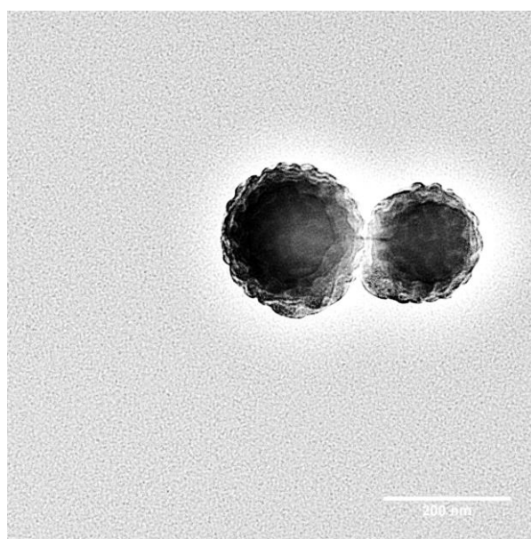
Figure B10. Top-view, bright field TEM micrograph of MB-MW-4 (PtBA M_n = 26.7 kDa, \sigma_{\text{PtBA}} = 0.51 chains/nm 2 ; PS M_n = 26.3 kDa, \sigma_{\text{PS}} = 0.29 chains/nm 2 ; \sigma_{\text{overall}} = 0.80 chains/nm 2 ) after being cast from a surfactant-stabilized aqueous dispersion. The sample was stained with RuO 4 vapor at room temperature for 20 min.
