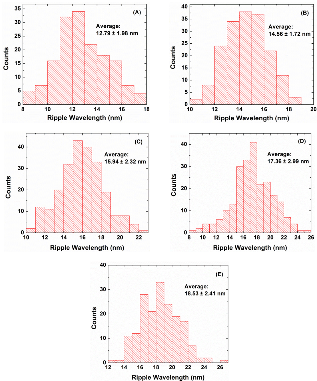
Figure 2.4 Distributions of ripple wavelengths of features (sum of widths of neighboring PtBA and PS stripes) obtained from TEM image analysis of (A) Figure 2.3A, MB-1, (B) Figure 2.3B, MB-2, (C) Figure 2.3C, MB-3, (D) Figure 2.3D, MB-4, and (E) Figure 2.3E, MB-5.
