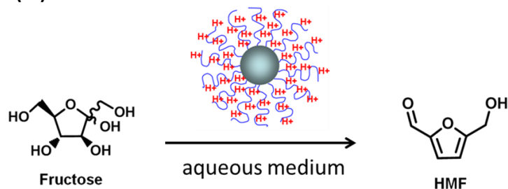
Scheme 5.1 (A) Schematic illustration for the dehydration of fructose to HMF catalyzed by an acidic hairy particle catalyst and (B) molecular structures of two acidic polymer brush catalysts: poly(3-(3-sulfopropyl)-1-(4-vinylbenzyl)-1H-imidazol-3-ium trifluoromethanesulfonate) (P(VBIm + -SO 3 H/CF 3 SO 3 - )) brush- and poly(4-vinylbenzenesulfonic acid) (PVBSA) brush-grafted silica particles.
