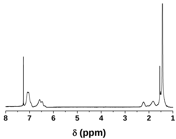
Figure B17. ^1\text{H} NMR spectrum of poly( tert -butyl acrylate)- b -polystyrene (PtBA- b -PS) (DB-2, M_{n,\text{SEC}} = 29.2 kDa, PDI = 1.15). \text{CDCl}_3 was used as solvent.
