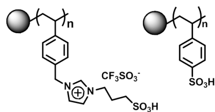
Scheme 5.1 (A) Schematic illustration for the dehydration of fructose to HMF catalyzed by an acidic hairy particle catalyst and (B) molecular structures of two acidic polymer brush catalysts: poly(3-(3-sulfopropyl)-1-(4-vinylbenzyl)-1H-imidazol-3-ium trifluoromethanesulfonate) (P(VBIm + -SO 3 H/CF 3 SO 3 - )) brush- and poly(4-vinylbenzenesulfonic acid) (PVBSA) brush-grafted silica particles.
