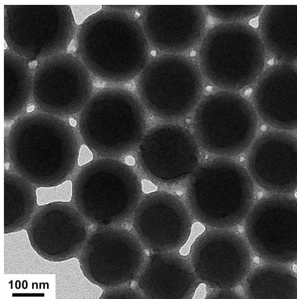
Figure A7. A top-view bright field TEM micrograph of MB-7 (PtBA M_n = 22.1 kDa, \sigma_{\text{PtBA}} = 0.10 chains/nm 2 ; PS M_n = 23.5 kDa, \sigma_{\text{PS}} = 0.022 chains/nm 2 ; \sigma_{\text{overall}} = 0.122 chains/nm 2 ) after being cast from a CHCl 3 dispersion, annealed with CHCl 3 vapor for at least 3 h, and stained with RuO 4 vapor at room temperature for 20 min. CHCl 3 is a good solvent for both PtBA and PS.
