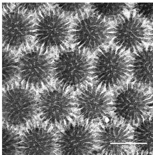
Figure B6. Top-view, bright field TEM micrograph of MB-MW-6 (PtBA M_n = 34.1 kDa, \sigma_{\text{PtBA}} = 0.50 chains/nm 2 ; PS M_n = 32.1 kDa, \sigma_{\text{PS}} = 0.35 chains/nm 2 ; \sigma_{\text{overall}} = 0.85 chains/nm 2 ) after being cast from a CHCl 3 dispersion and annealed with CHCl 3 vapor. The sample was stained with RuO 4 vapor at room temperature for 20 min.
