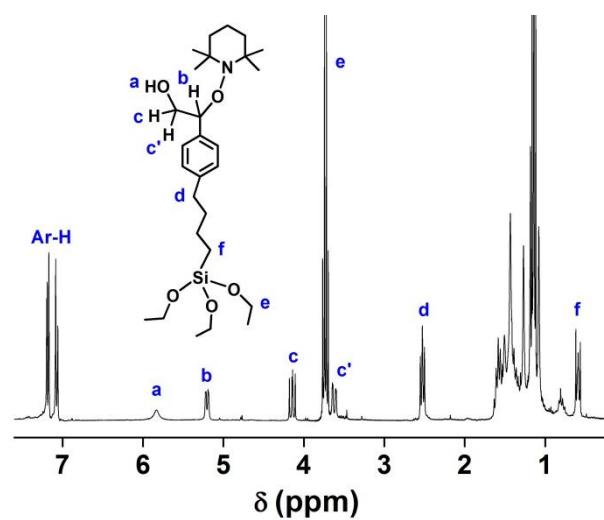
Figure 4.1 ^1\text{H} NMR spectra of 2-[4-(1-triethoxysilylbutyl)phenyl]-2-(2',2',6',6'-tetramethyl-1'-piperidinyloxy)ethanol (Y-Silane-B). \text{CDCl}_3 was used as solvent.
