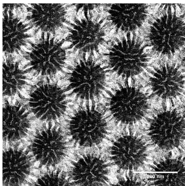
Figure B4. Top-view bright field TEM micrograph of MB-MW-4 (PtBA M_n = 26.7 kDa, \sigma_{\text{PtBA}} = 0.51 chains/nm 2 ; PS M_n = 26.3 kDa, \sigma_{\text{PS}} = 0.29 chains/nm 2 ; \sigma_{\text{overall}} = 0.80 chains/nm 2 ) after being cast from a CHCl 3 dispersion and annealed with CHCl 3 vapor. The sample was stained with RuO 4 vapor at room temperature for 20 min.
