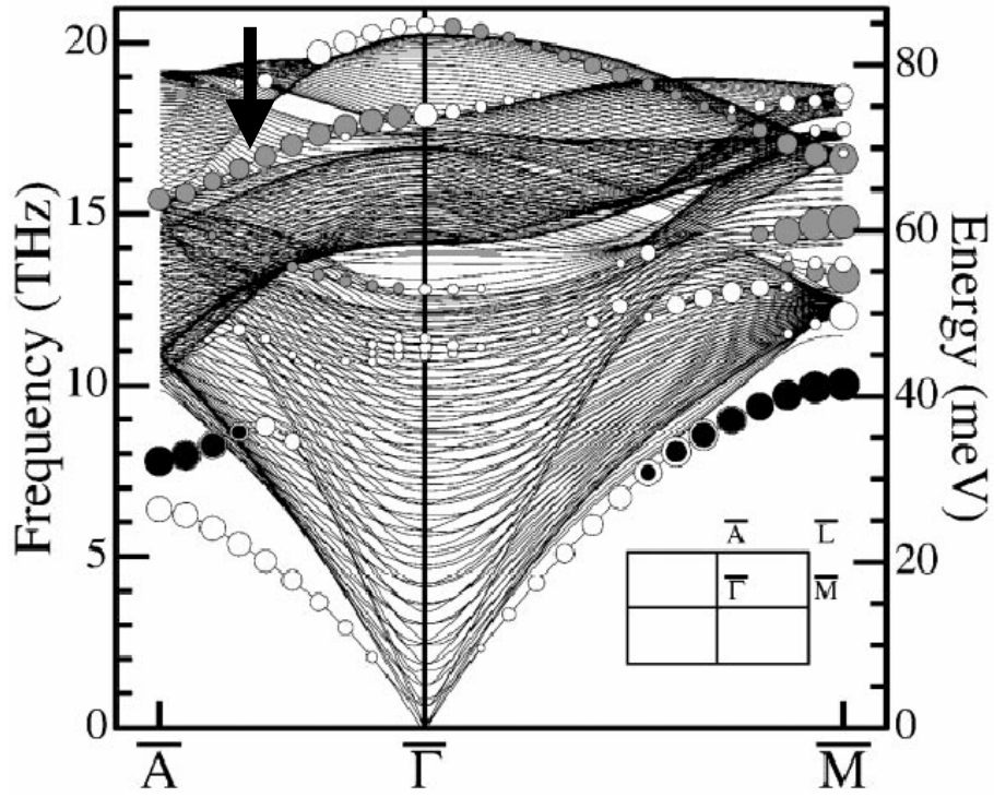
Figure 4.15 The calculated surface phonon band on the relaxed surface of Be(10 \bar{1} 0). The arrow indicates the optical phonon dispersion around 64 meV [19].
