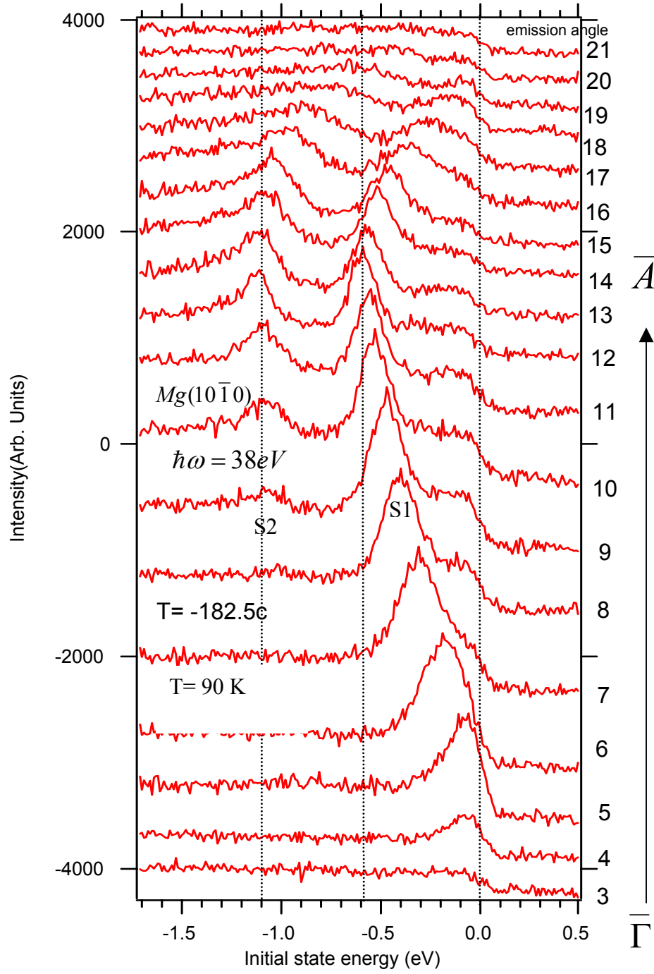
Figure 5.2 Energy dispersion curves of the surface states on Mg(10 \bar{1} 0) between \bar{\Gamma} and \bar{A} .
