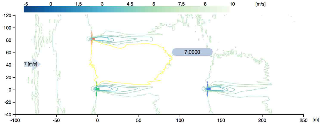
Figure 7.7: Velocity contours at hub height.
