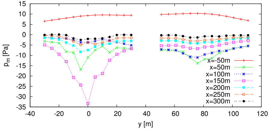
Figure 7.3: Mean pressure sampled on hub height transects upwind and down wind of turbines in 25 m/s inflow operating at 43 rpm over t=[40,50] s.
