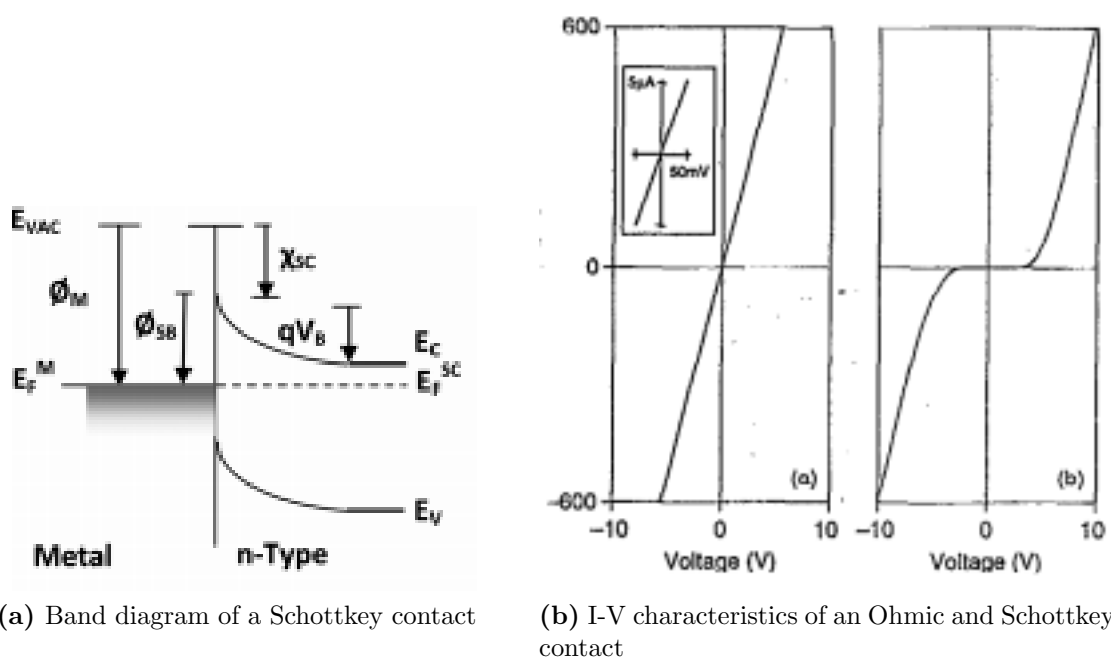
Figure 1.10: Diagram of (a) Schottky contact from Source [69] and (b) electrical behavior of contact type from Source [70].
